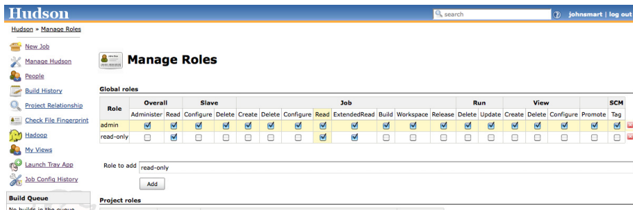
Figure 7.25. Managing global roles
