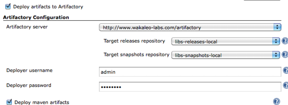
Figure 5.43. Deploying to Artifactory from Jenkins
