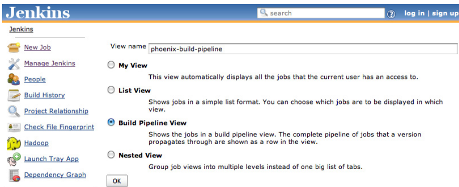
Figure 10.56. Creating a Build Pipeline view
