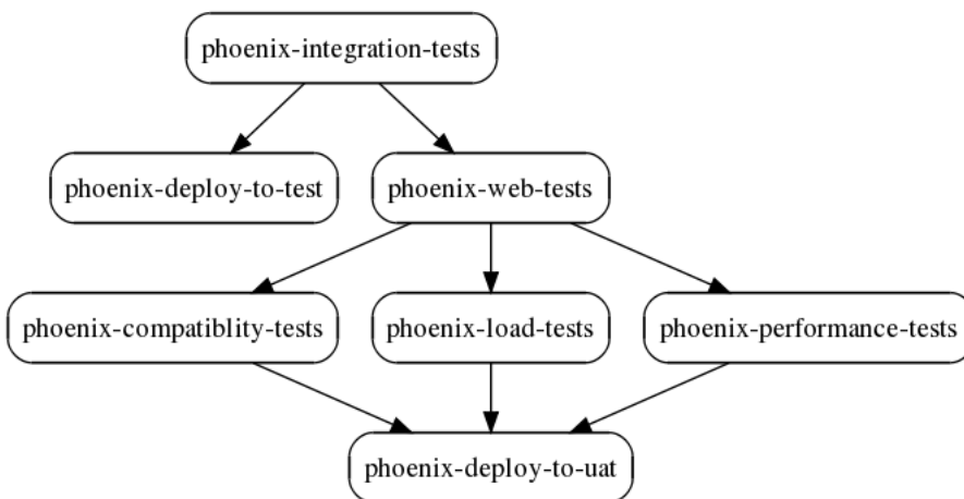
Figure 10.33. A more complicated build job dependency graph
