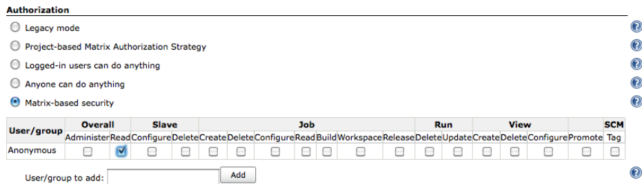
Figure 7.16. Matrix-based security configuration
