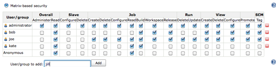
Figure 7.18. Setting up other users
