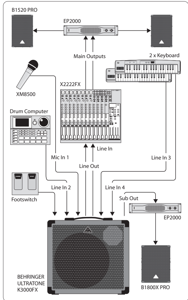
Afb. 3.2: Live-setup
