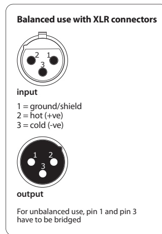
Afb. 4.3: XLR connectors
