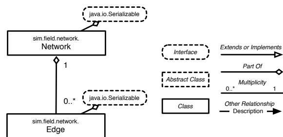
Figure 7.1 UML diagram of MASON's Network package. Not a very complex package!
