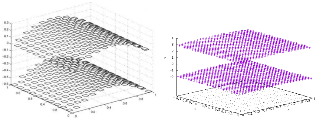
Left: pressure solution as shown in [30]; Right: pressure solution obtained with fieldstone.
