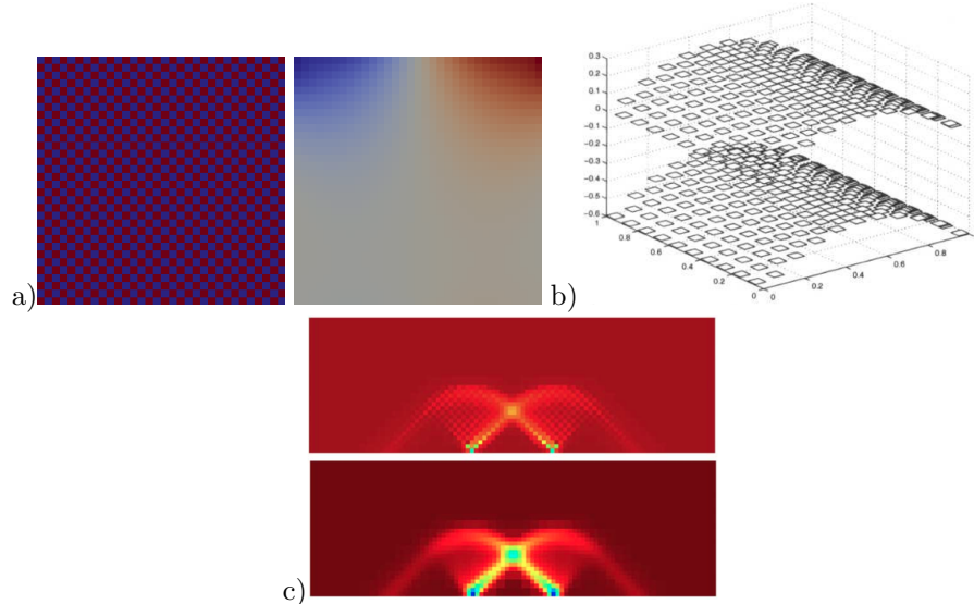
a) element pressure for a 32x32 grid and for a 33x33 grid; b) image from [29, p307] for a manufactured solution; c) elemental pressure and smoothed pressure for the punch experiment [93]
