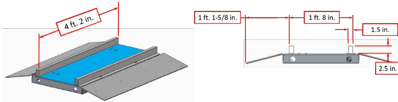
Figure 2-9: Moat Dimensions
