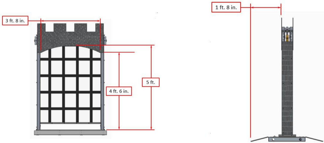
Figure 2-6: Portcullis Dimensions
