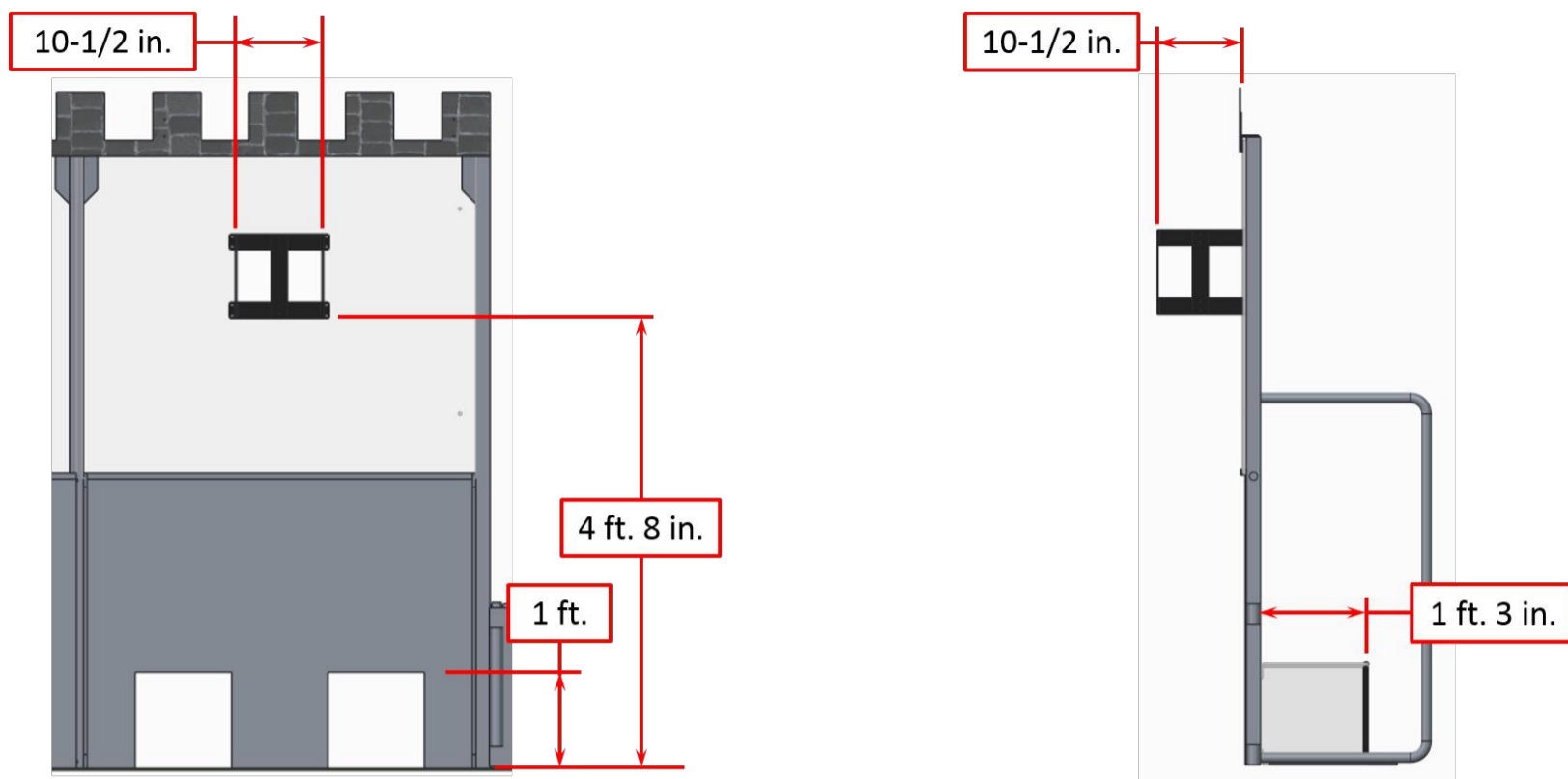
Figure 2-26: HUMAN PLAYER STATION Dimensions
