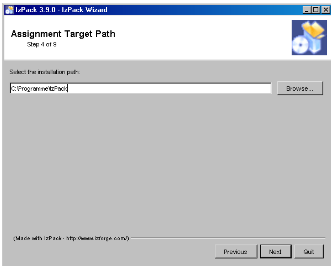
IzPack frame (TargetPanel) with heading panel and a text counter in the heading panel with alternative frame title, no panel image.
