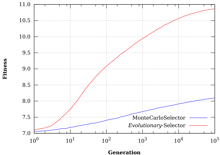
Figure 2.8.1: Selector-performance (Knapsack)
