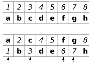
Figure 1.3.13: Uniform crossover
