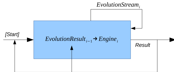
Figure 4.1.7: Adaptive Engine
