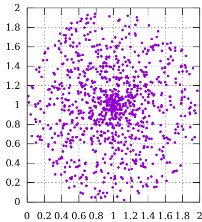
Figure 4.1.8: Circle points
