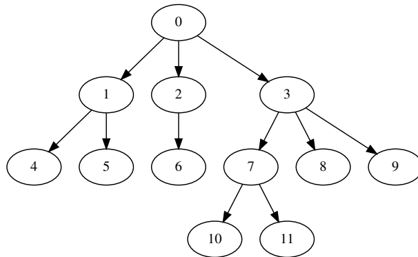
Figure 4.1.1: Example tree
