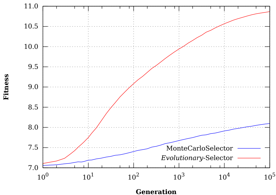
Figure 2.8.1: Selector-performance (Knapsack)
