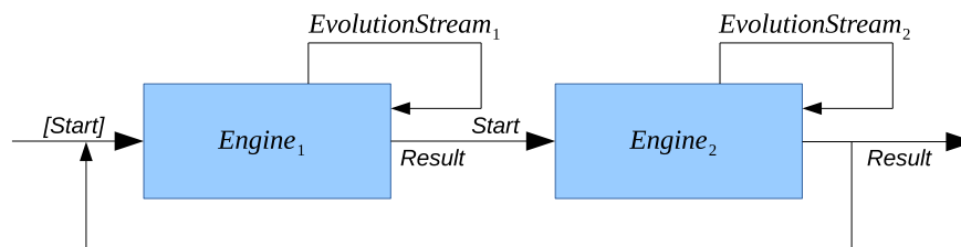
Figure 4.1.6: Cyclic Engine
