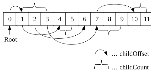
Figure 4.1.3: Example FlatTree
