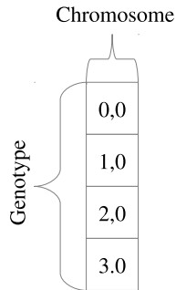
Figure 1.3.5: Column-major Genotype vector
