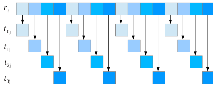
Figure 1.4.3: Leapfrogging
