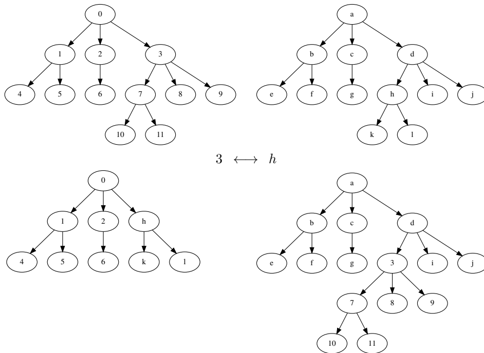
Figure 4.1.4: Single-node crossover
