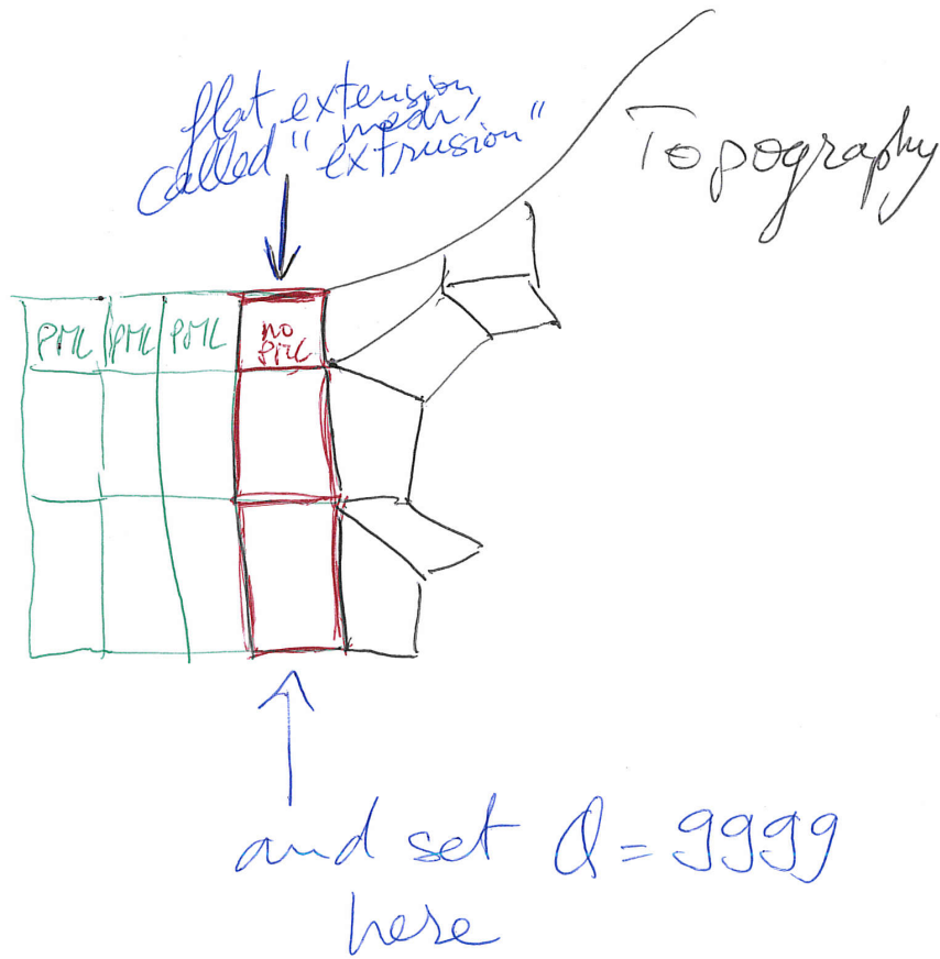
Figure 4.3: Mesh extrusion for PML (green elements) and a non-PML stabilization layer (red elements).
