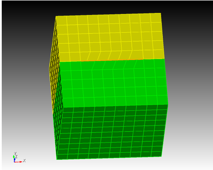
Figure 6.2: Screenshots of a CUBIT example showing split nodes for a fault reaching the surface. Surface trace of the fault is shown in orange. Note that the edges of the fault are not split while the interior nodes are offset by a small distance on either side of the fault
