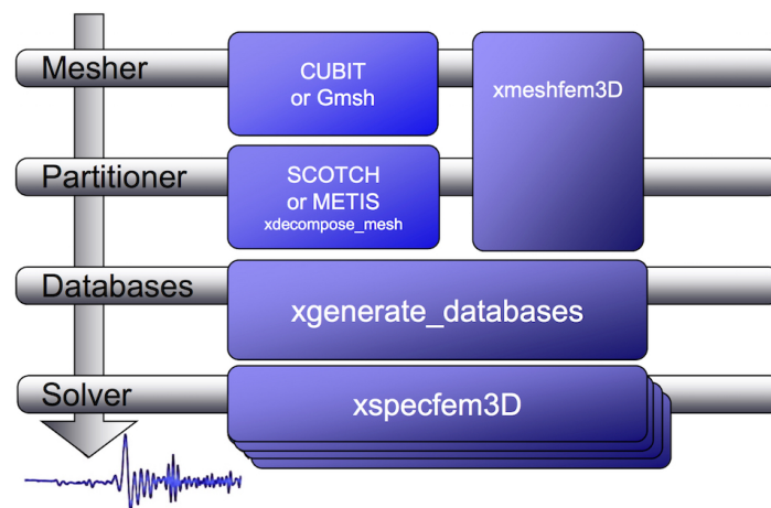
Figure 4.1: Schematic workflow for a SPECIFEM3D Cartesian simulation. The executable xgenerate_databases creates the GLL mesh points and assigns specific model parameters.
