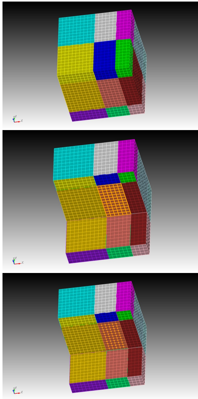
Figure 6.1: Screenshots of the CUBIT example for the embedded fault with split nodes: The entire mesh is decomposed into several volumes bounding the fault (top), the fault surface 168 is shown as orange squares (middle) and split nodes of the fault shown as orange dots (bottom). Note that only interior nodes of the fault are split while those on the edges of the fault surface are touching each other.
