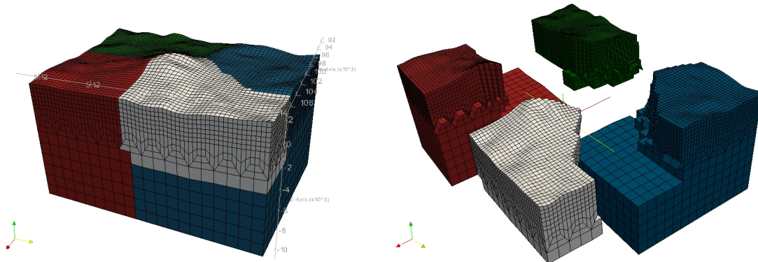
Figure 3.4: Example of a mesh partitioning onto four cores. Each single core partition is colored differently. The executable xdecompose_mesh can equally distribute the mesh on any arbitrary number of cores. Domain decomposition is explained in detail in Martin et al. [2008a], and excellent scaling up to 150,000 processor cores is shown for instance in Carrington et al. [2008], Komatitsch et al. [2008], Martin et al. [2008a], Komatitsch et al. [2010a], Komatitsch [2011].
