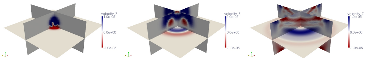
Figure 12.3: Paraview visualization using movie volume files (converted by xcombine_vol_data and mesh2vtu.pl ) and showing snapshots of vertical velocity components at different times.
