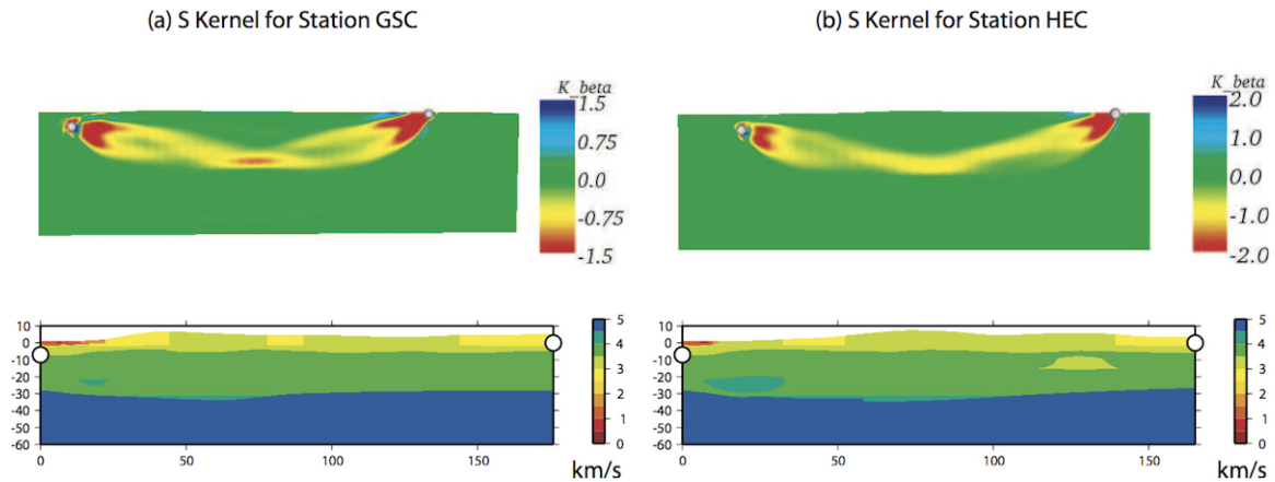
Figure 12.4: (a) Top Panel: Vertical source-receiver cross-section of the S-wave finite-frequency sensitivity kernel K_\beta for station GSC at an epicentral distance of 176 km from the September 3, 2002, Yorba Linda earthquake. Lower Panel: Vertical source-receiver cross-section of the 3D S-wave speed model used for the spectral-element simulations [Komatitsch et al., 2004]. (b) The same as (a) but for station HEC at an epicentral distance of 165 km [Liu and Tromp, 2006].
