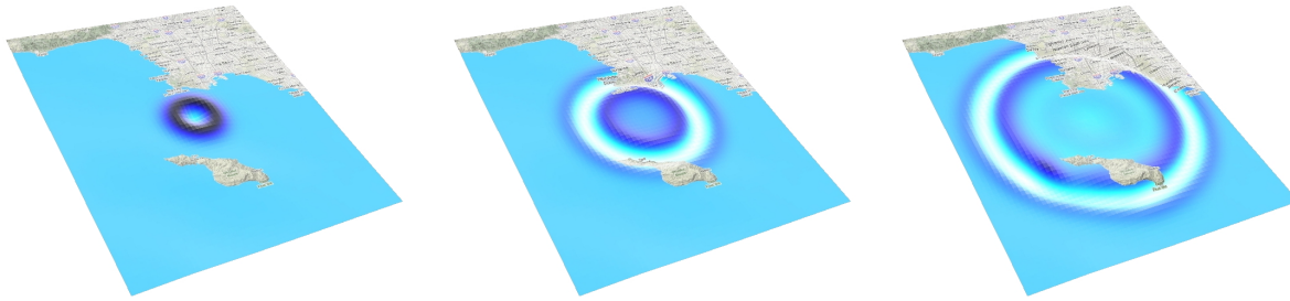
Figure 12.2: Visualization using AVS files created by xcreate_movie_shakemap_AVS_DX_GMT showing movie snapshots of vertical velocity components at different times.
