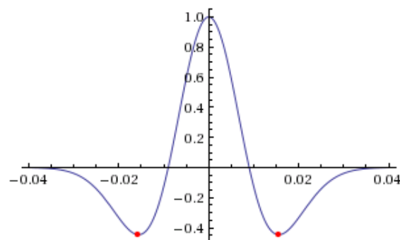
Figure 4.2: We use the standard definition of a Ricker (i.e., second derivative of a Gaussian). Image taken from http://subsurfwiki.org .
