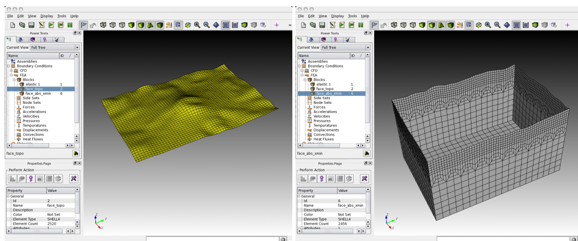
Figure 3.3: Example of the block definitions for the free surface 'face_topo' (left) and the absorbing boundaries, defined in a single block 'face_abs_xmin' (right) in CUBIT.
