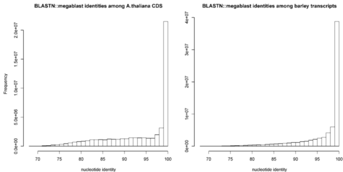
Figure 3: Histograms of % identity reported by BLASTN among Arabidopsis thaliana CDS sequences (left) and Hordeum vulgare (right) transcripts. Note that the default BLASTN algorithm ( megablast ) hardly reports alignments with identities < 70\% . Plots were computed from 51,110,547 and 70,653,179 alignments, respectively.
