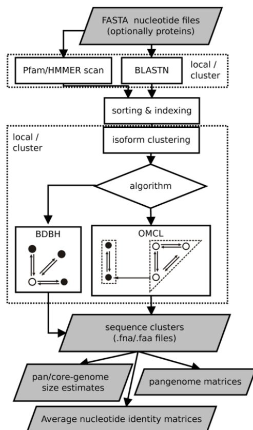
Figure 1: Flowchart of get.homologues-est.
