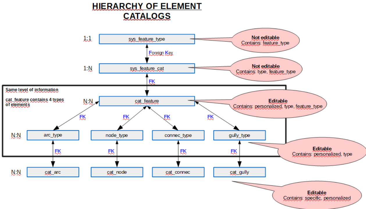
Image 21: Schema representing the hierarchy of tables related to principal elements of Giswater.
