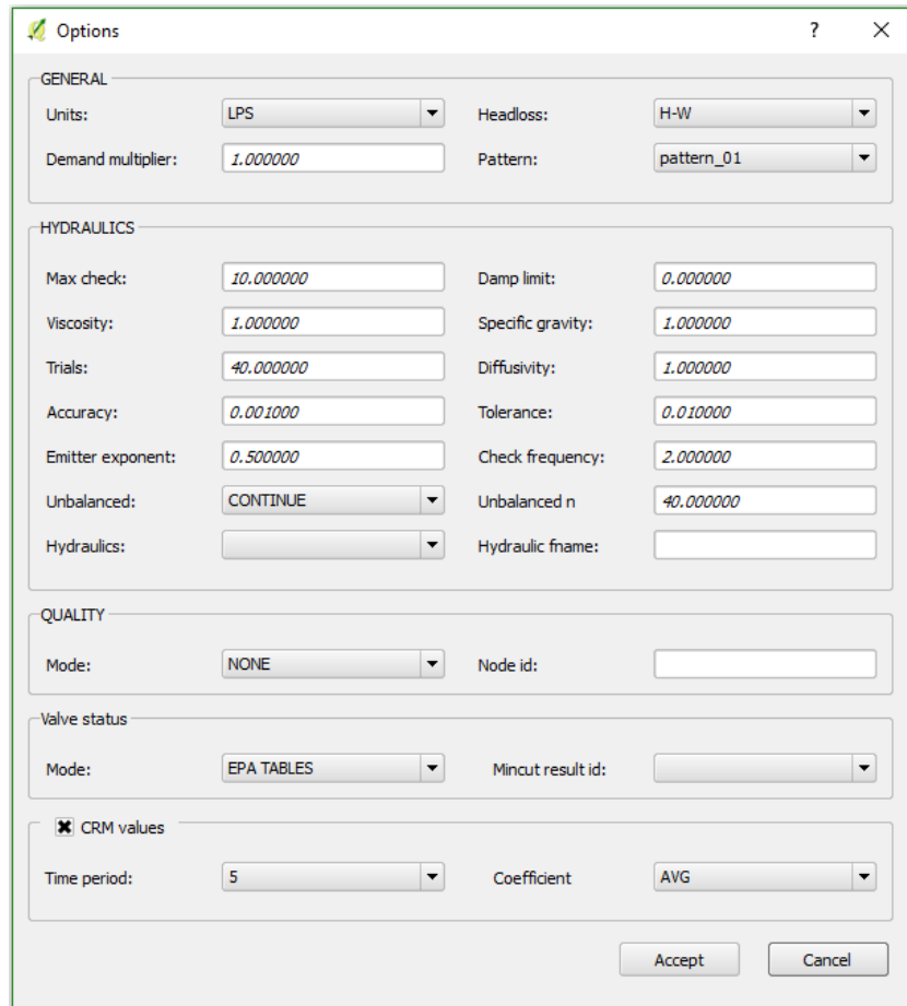
Image 67: Form of Options section of Go 2 EPA tool. All the data and configuration of the model should be introduced here.
