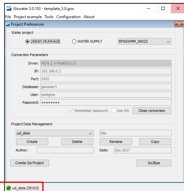
Image 7: Project preferences and management.
