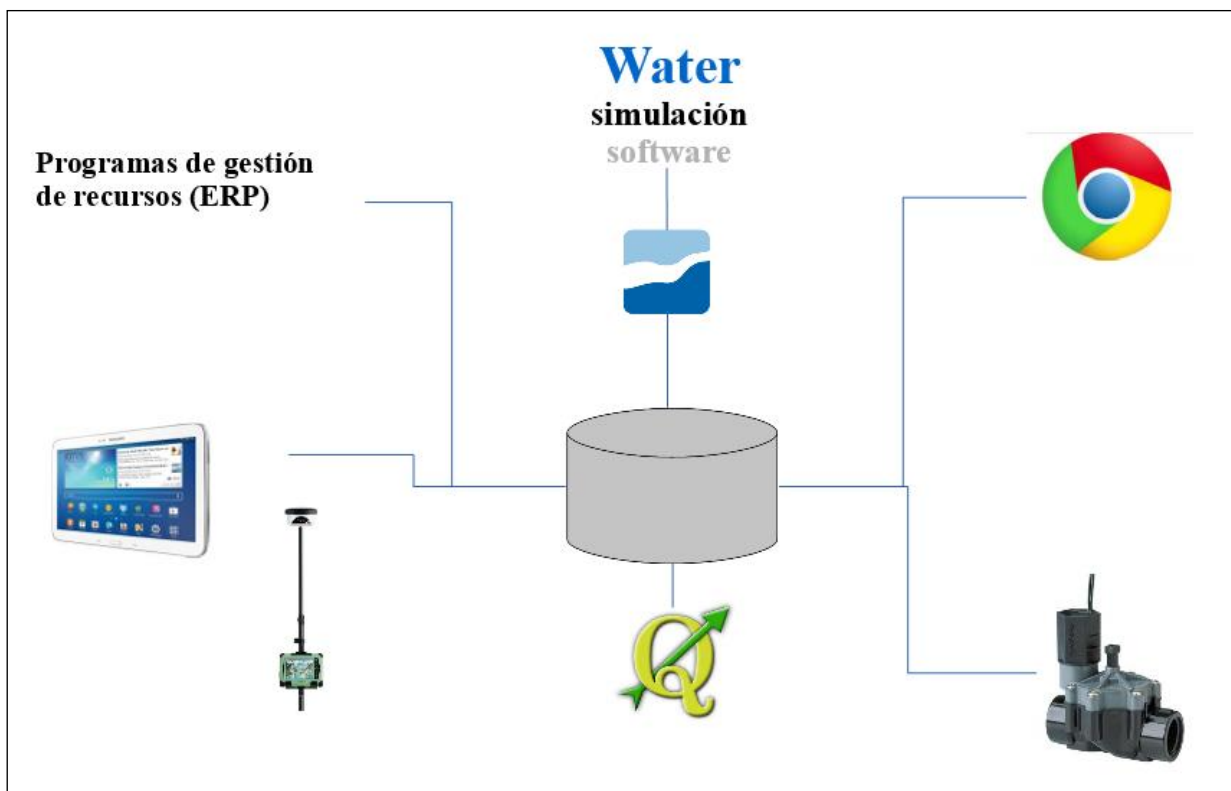
Image 1: Schema of the applications used by Giswater with a database in its central point.
