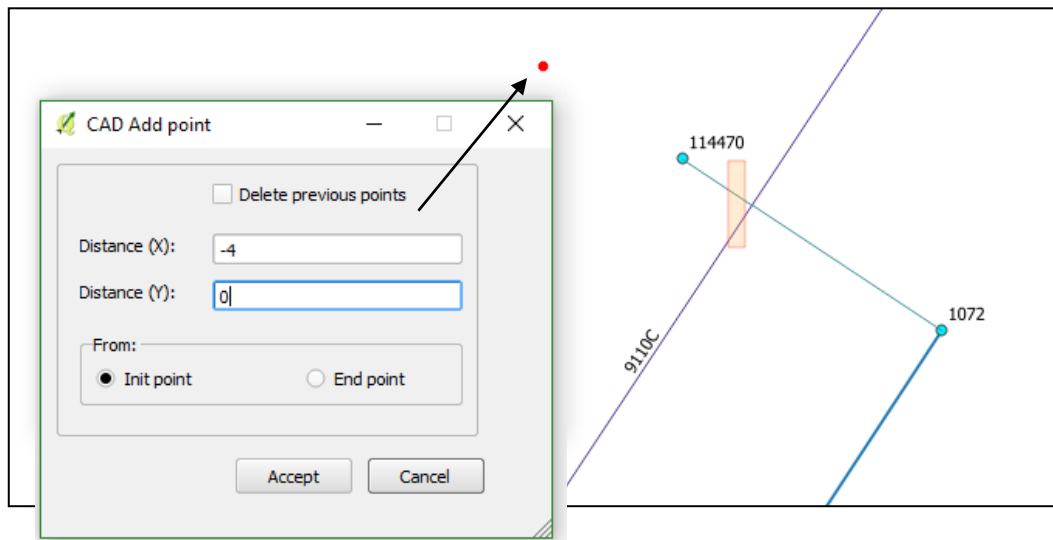
Image 93: the tool Add relative point can be used to place the point as the determined distance from another element. The temporal line is selected by the rectangle for its better visualization.
