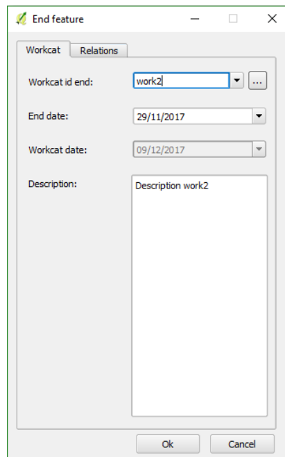
Image 61: Form of end feature. In the tab Relations it's possible to link one or many elements that will have their state changed to 0.
