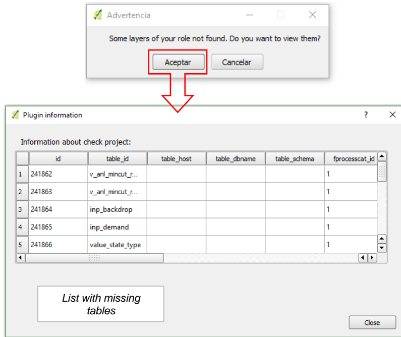
Image 103: The function audit_check_project acts every time the project is opened. In case of finding the layers that should be loaded, but are not, shows the list of those layers.
