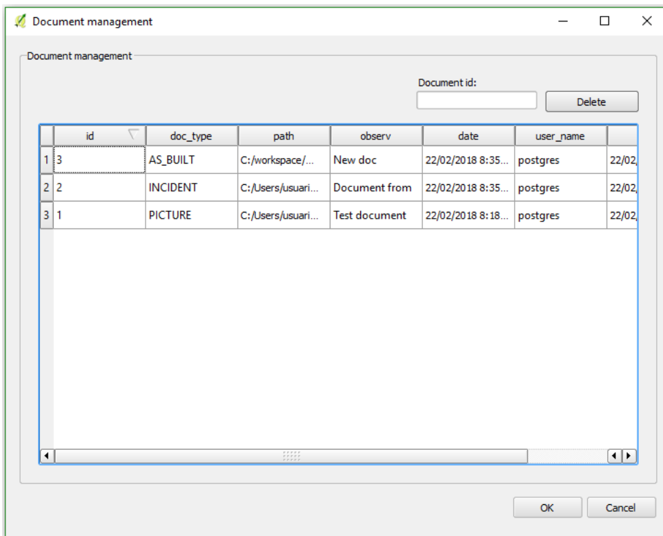
Image 58: Form of document manager. Here all the documents related to the network are visible. Form allows to filter, show and delete them.
