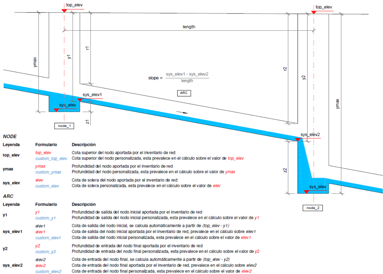
Image 19: Schema helps understand the information that should be put in the fields related to elevation, dimensions, depth of node and arc elements of urban drainage projects (UD).
