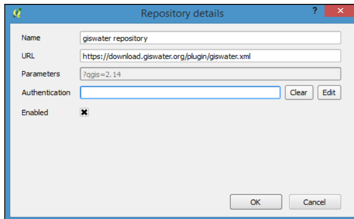
Image 24: The repository is added manually, using a URL.
