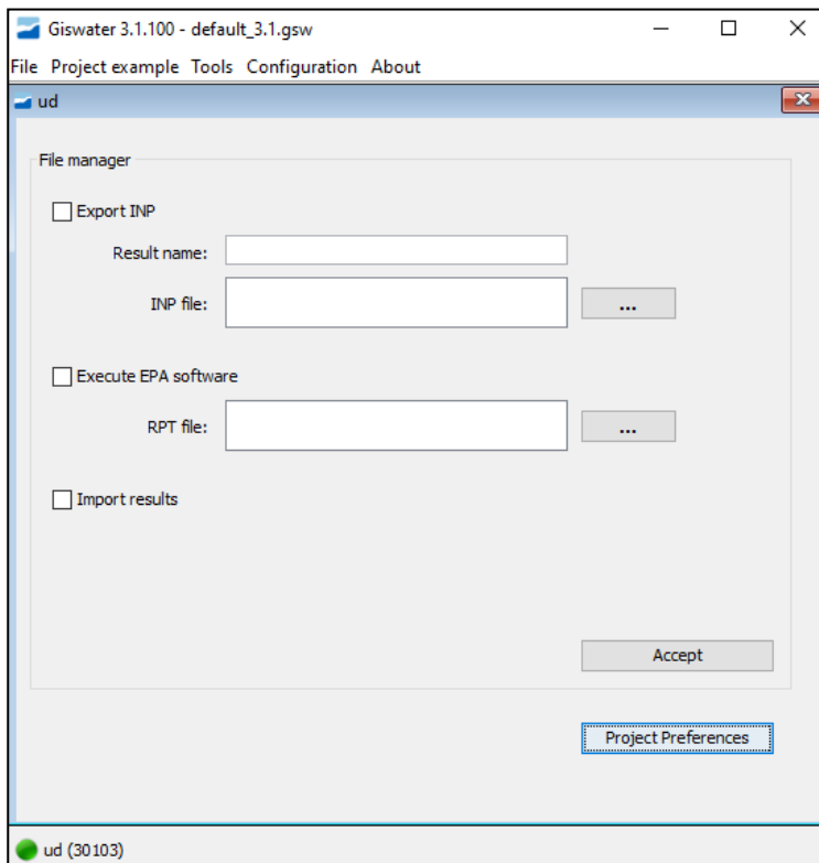
Image 69: Driver of Giswater allows to establish the paths where the files related to hydraulic model will be saved. In order to go to this page, click Go2Epa button located in Project preferences.
