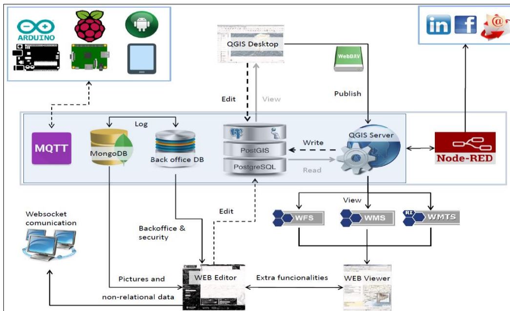
Image 3: All the technologies that should be installed in order to use Giswater with the most reliability.
