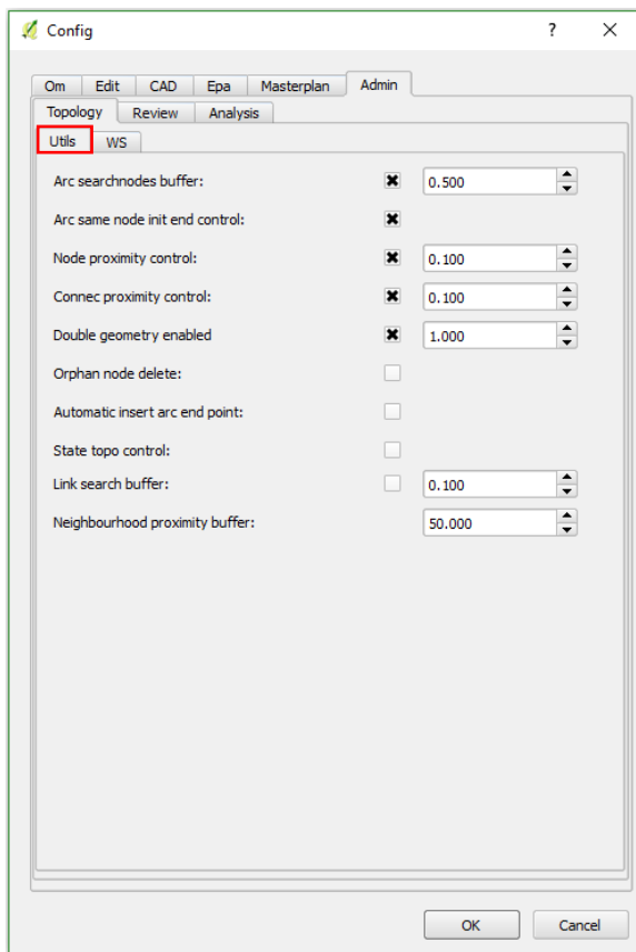
Image 82: Form of config, topology tab.
