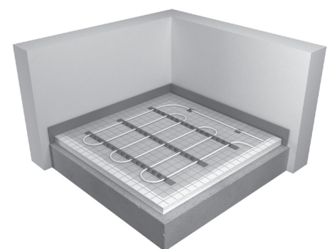
Fix the Metro cliprail to the insulation and fix the pipe.
