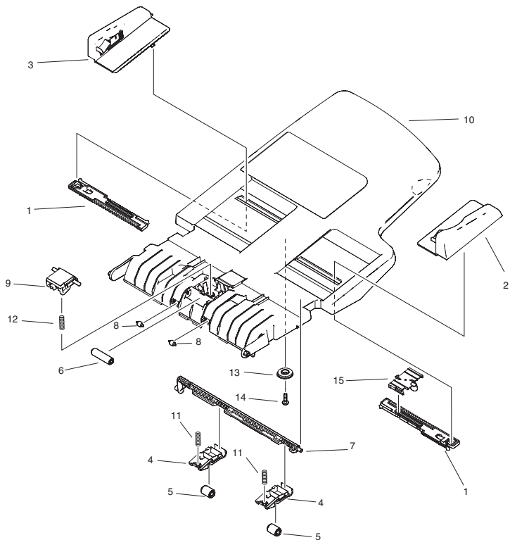
FIGURE 162 DOCUMENT TRAY ASSEMBLY
