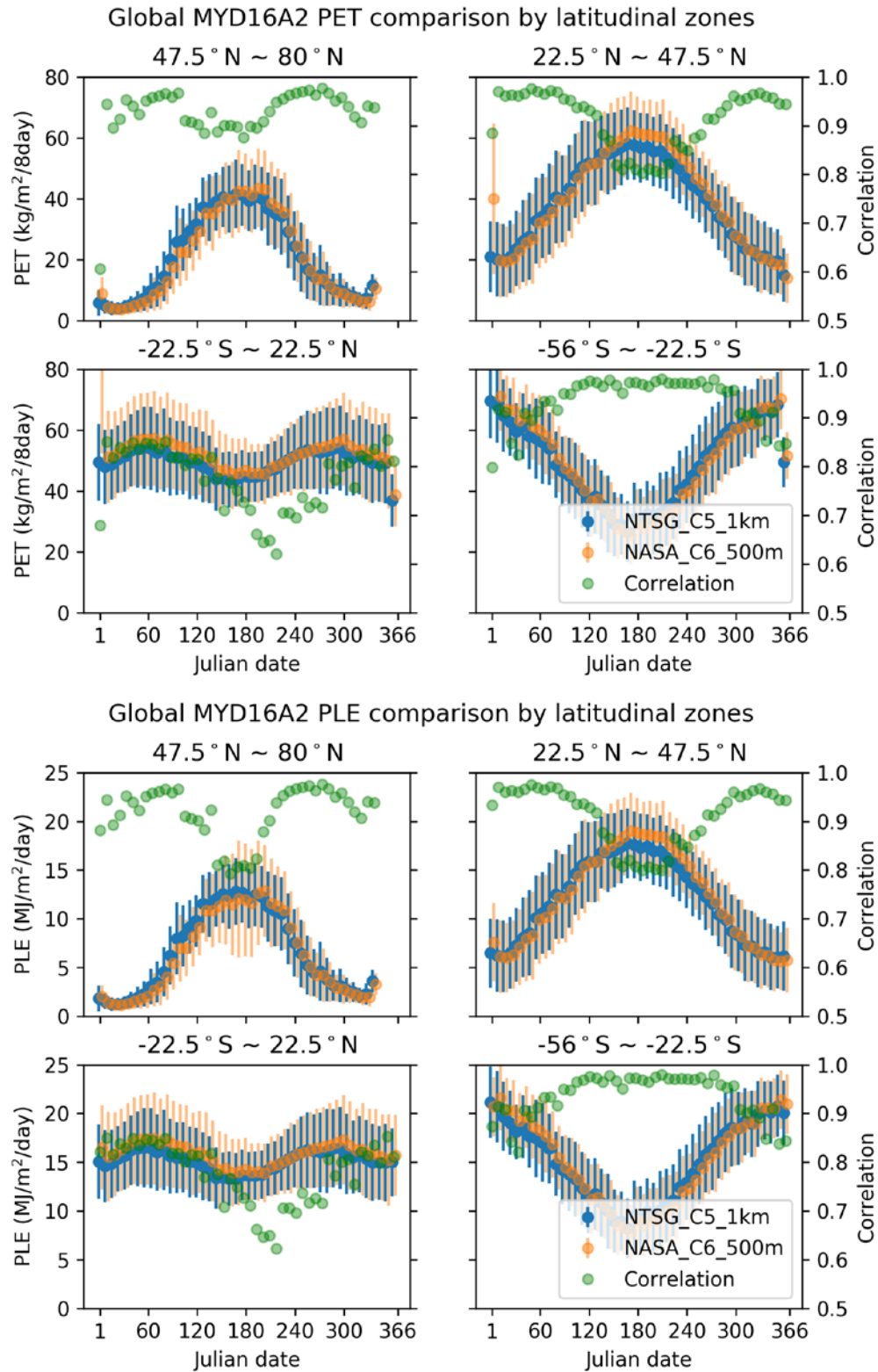
Figure 6.2. D) The 46 8-day mean, Standard Deviation (STD) of PET and PLE for NASA and NTSG MYD16A2 in year 2008, and the correlation between the two data sets by latitudinal zones.
