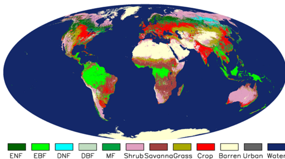
Figure 3.1. Collection5 1-km MODIS ET used land cover type 2 in 1-km Collection4 MOD12Q1 dataset. Whereas Collection6 operational 500-m MODIS ET is using land cover type 1 in Collection5.1 500-m MCDLCHKM which is a 3-year smoothed MODIS land cover data set. This figures shows land cover types from the Collection4 MOD12Q1 dataset: Evergreen Needleleaf Forest (ENF), Evergreen Broadleaf Forest (EBF), Deciduous Needleleaf Forest (DNF), Deciduous Broadleaf Forest (DBF), Mixed forests (MF), Closed Shrublands (CShrub), Open Shrublands (OShrub), Woody Savannas (WSavanna), Savannas (Savanna), grassland (Grass), and Croplands (Crop). Note that in this figure, we combined CShrub and OShrub into Shrub, and
