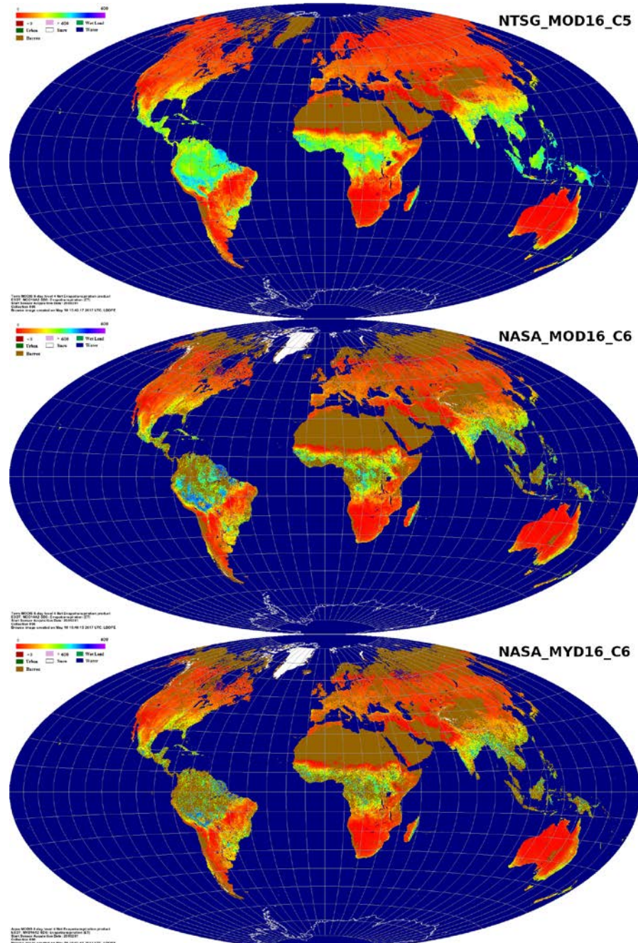
Figure 6.1. Comparison of MOD16A2 for an 8-day of 2008281 (Oct 7 th through Oct 14 th ) between NTSG Collection5 gap-filled and NASA operational Collection6 with data gaps due to cloudiness or snow cover.
