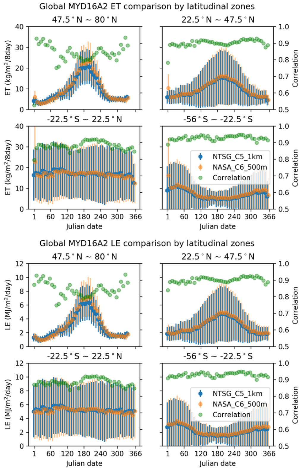
Figure 6.2. C) The 46 8-day mean, Standard Deviation (STD) of ET and LE for NASA and NTSG MYD16A2 in year 2008, and the correlation between the two data sets by latitudinal zones.
