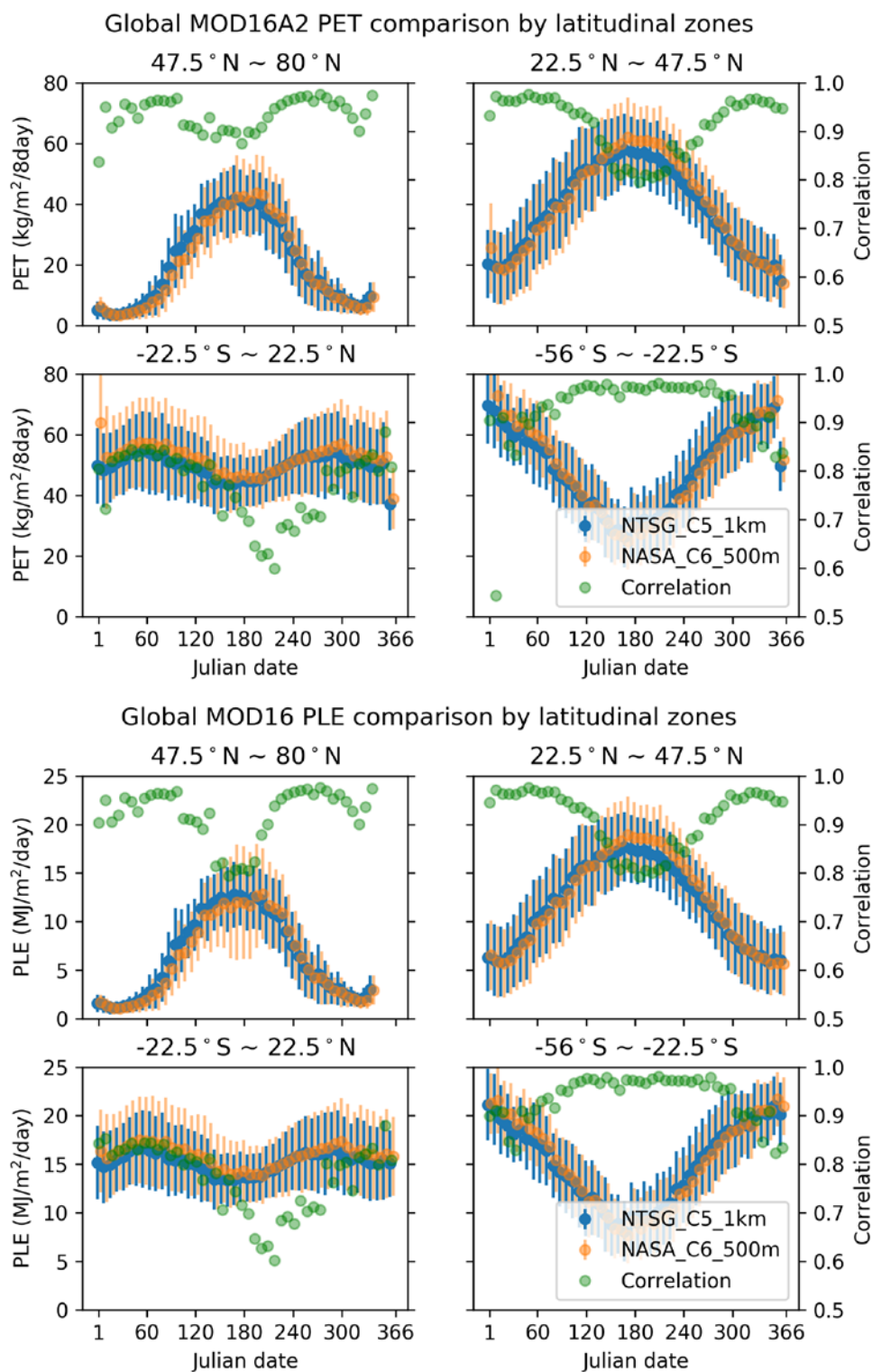
Figure 6.2. B) The 46 8-day mean, Standard Deviation (STD) of PET and PLE for NASA and NTSG MOD16A2 in year 2008, and the correlation between the two data sets by latitudinal zones.
