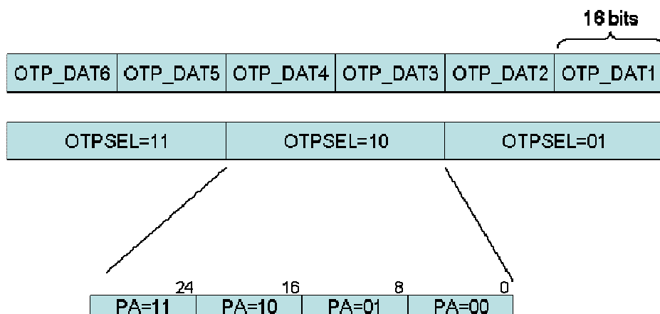
Figure 34 Programmable OTPs organization.
