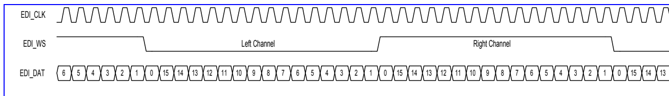
Figure 73 EDI Format 2: I 2 S (FMT = 1).
