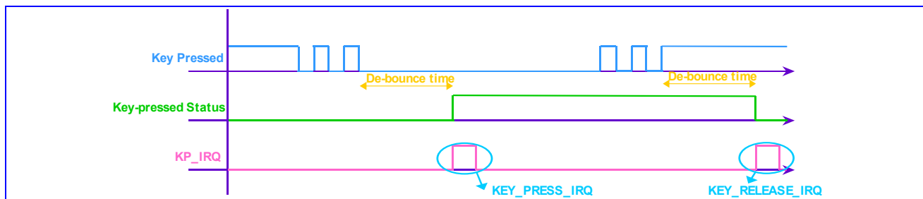
Figure 43 One key pressed with de-bounce mechanism denoted
