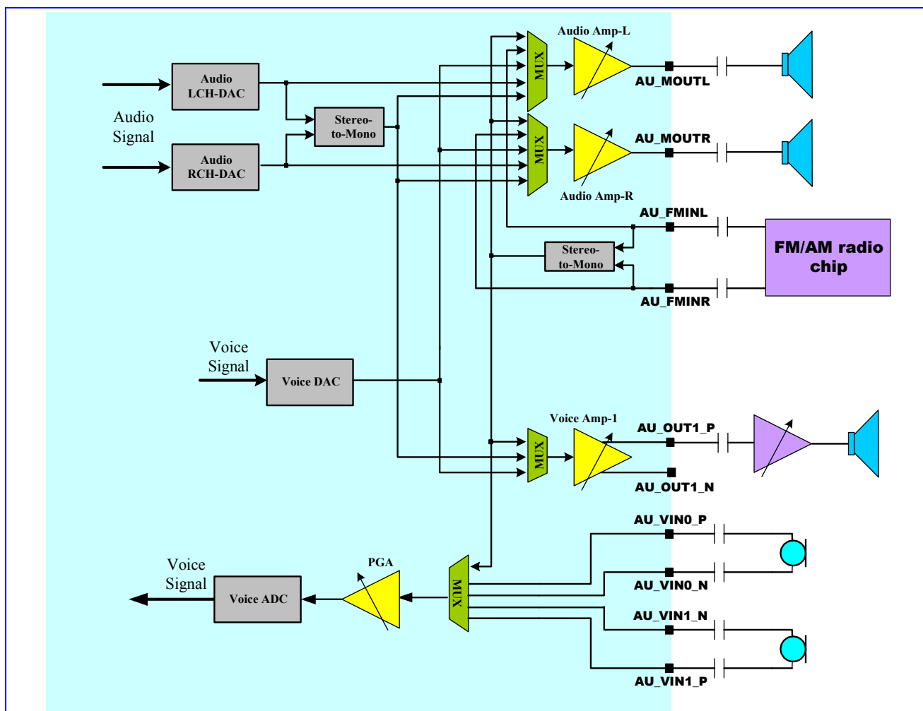
Figure 69 Block diagram of audio front-end
