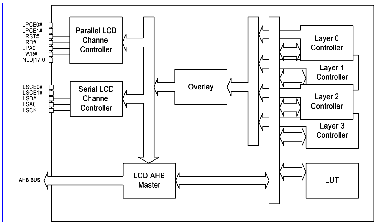
Figure 55 LCD Interface Block Diagram
