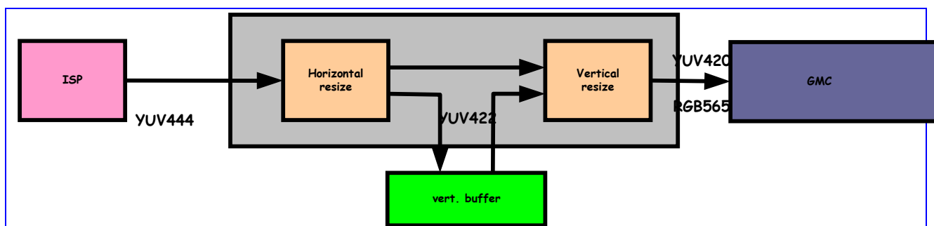
Figure 57 Overview of Image Resizer
