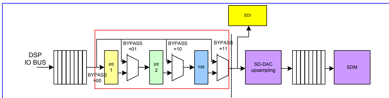
Figure 75 Block diagram of the audio path.
