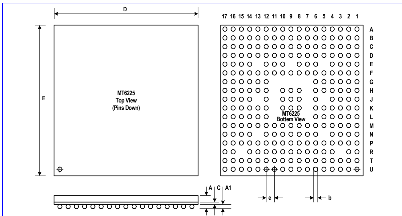
Figure 4 Outlines and Dimension of TFBGA 12mm*12mm, 264-ball, 0.65 mm pitch Package
