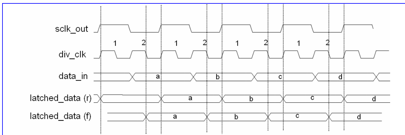
Figure 3 Illustration of data line latch timing
