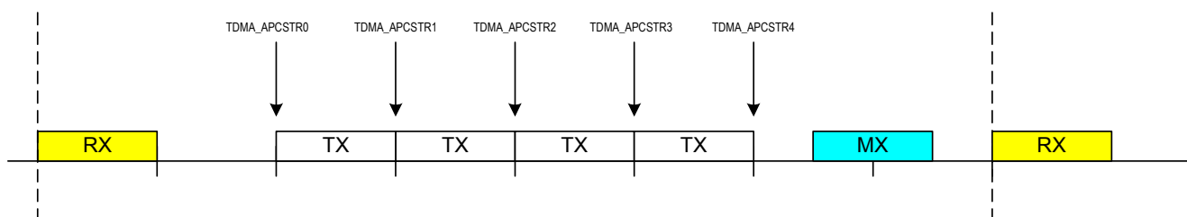
Figure 82 Timing diagram of TDMA_APCSTR.
