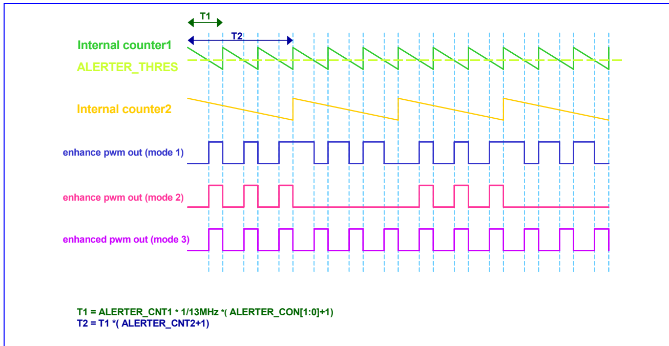
Figure 38 Alerter waveform
