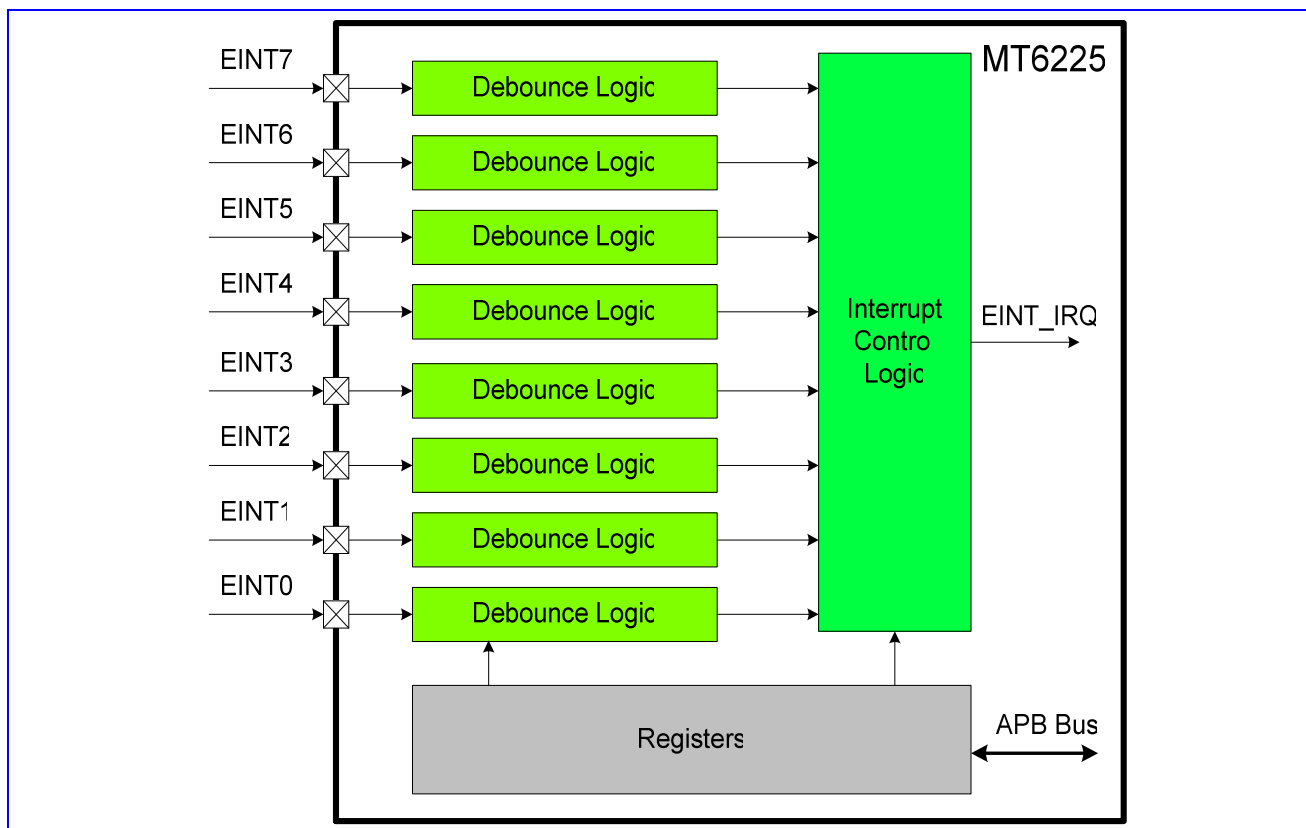
Figure 19 Block diagram of External Interrupt Controller
