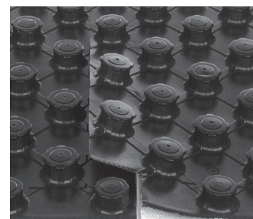
Overlap the edges of the Nexxa Panels.
