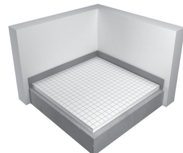
Install the perimeter strip and additional insulation if required.
