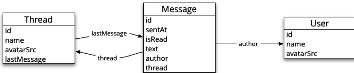
Chat Models
