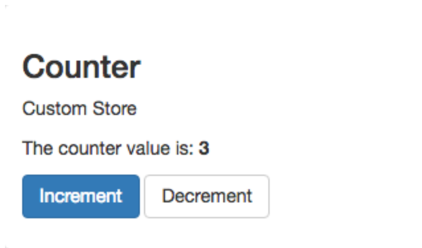
Counter App
