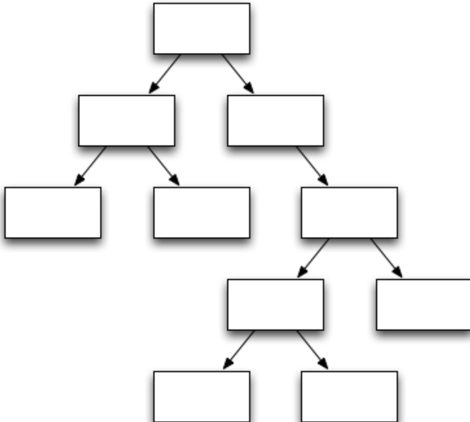
Component tree
