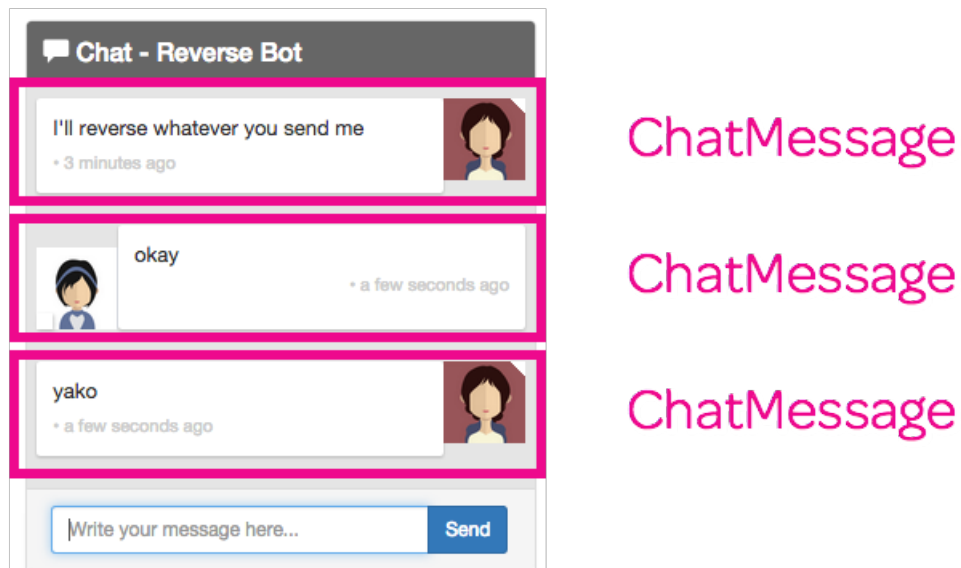
The ChatMessageComponent
