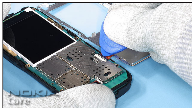
10. Use the SRT-6 for opening the flex connector.
