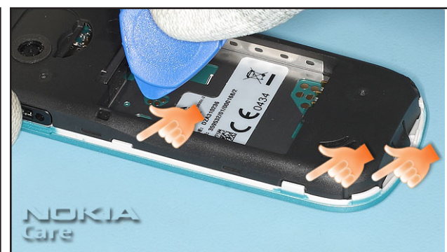
4. Unlock this 3 plastic clips with the SRT-6, starting at the top.
