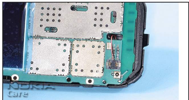
4. Close the connector. Mind the correct positioning of the connector before going on.
