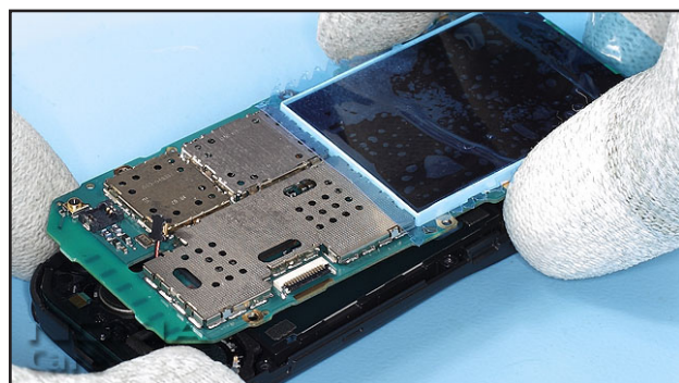
14. Gently lift up the ENGINE MODULE. Slot through the connector of the vibra.
