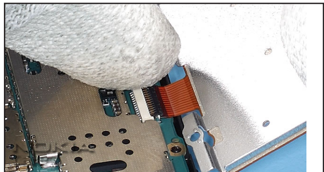
6. Now align the flex foil evenly and close the connector.
