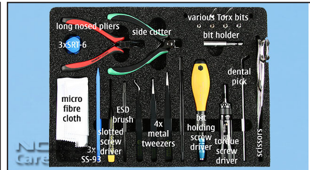
2. You need the Nokia Standard Toolkit version 2 and the SS-88.
