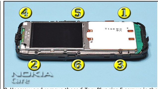
8. Unscrew and remove these 6 Torx Plus size 5 screws in the shown order.
