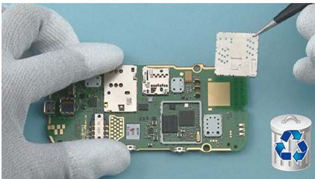
27) Remove the BB SHIELDING LID with the tweezers. Do not use the BB SHIELDING LID again. Discard it.
