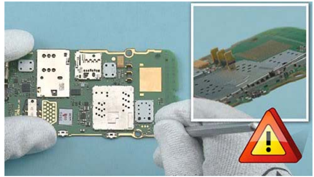
26) Use the dental tool to detach the BB SHIELDING LID. Be careful not to injure yourself with the sharp end of the dental tool.
