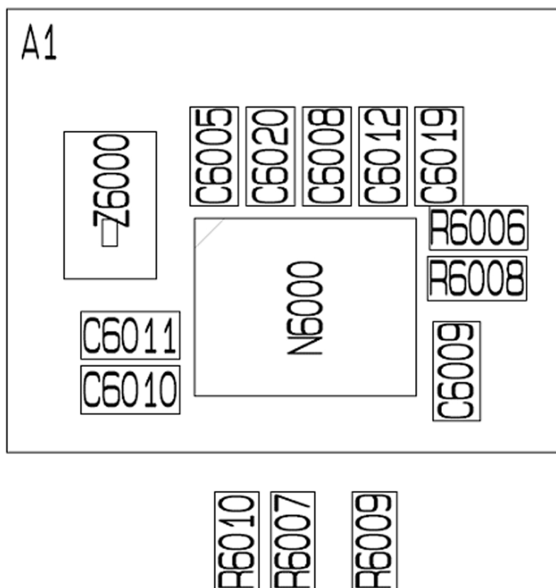
Figure 50 Test points in Archie Bluetooth ASIC circuit – BTHCost4.0D (CSR8810)
