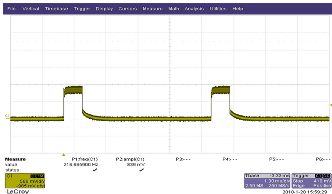
Figure 44 X-Gold TX pin volts @ C7108(LB) /C7109 (HB)
