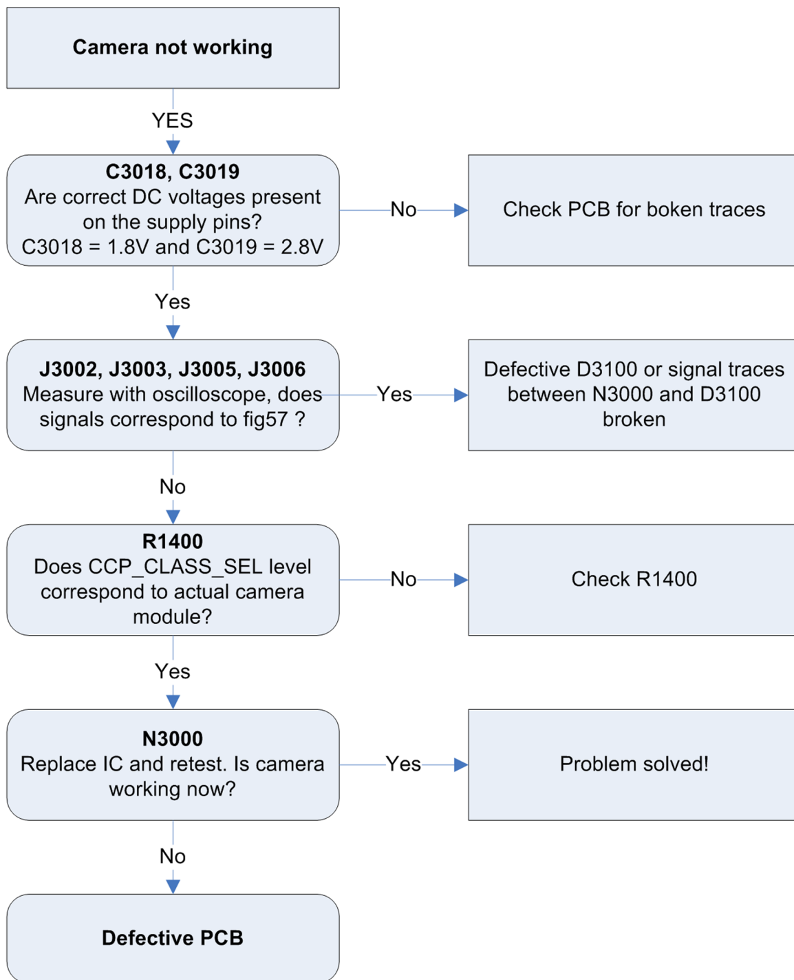
Figure 26 Camera interface IC troubleshooting guide
