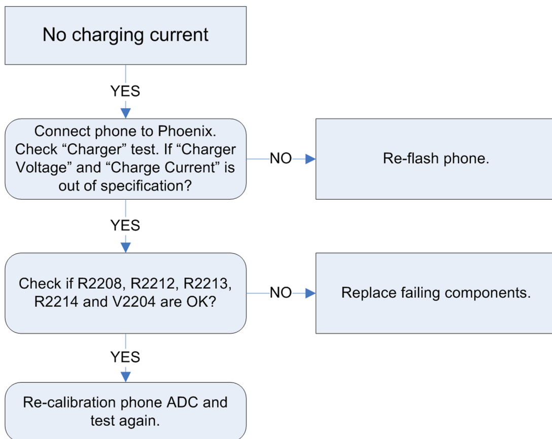
Figure 16 No charging current
