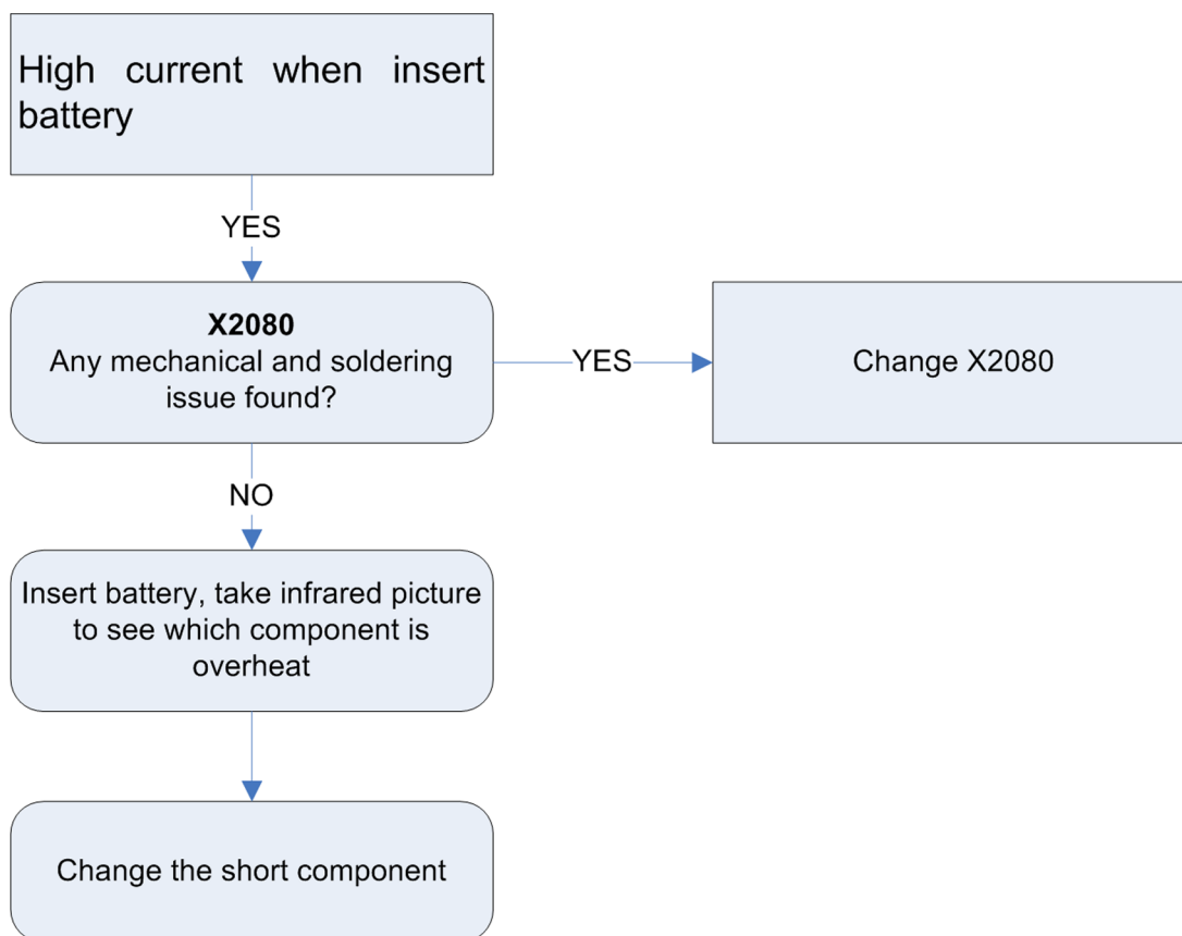
Figure 8 High current when battery inserted
