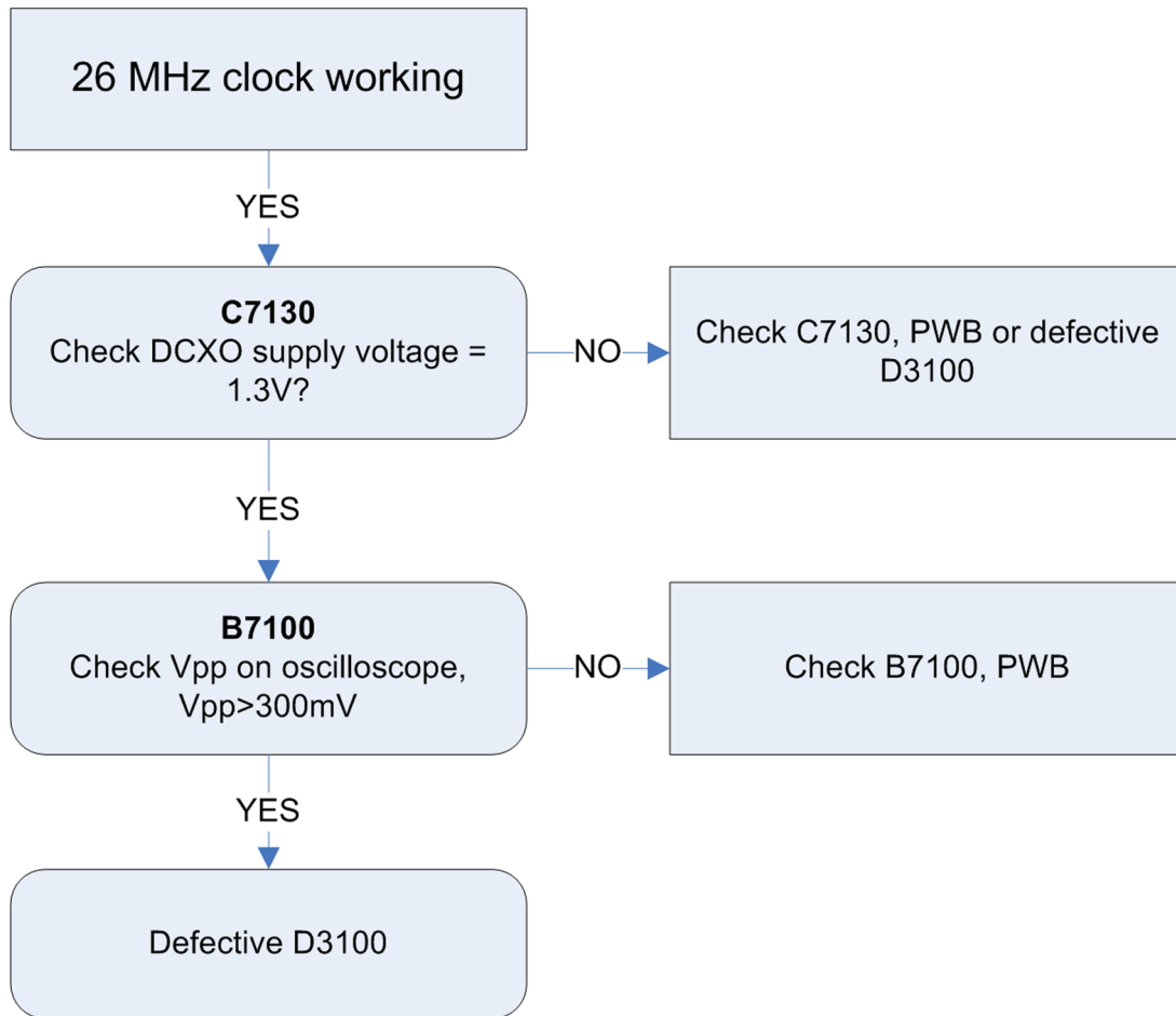
Figure 13 26 MHz Clock does not work
