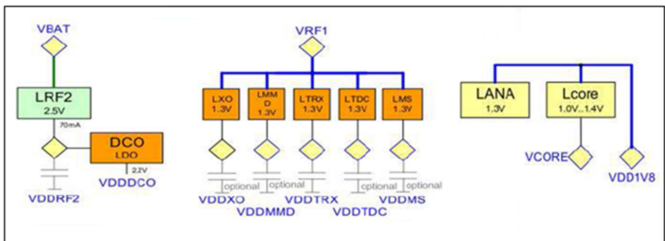
Figure 72 Power concepts for X-GOLD213 RF sub-system
