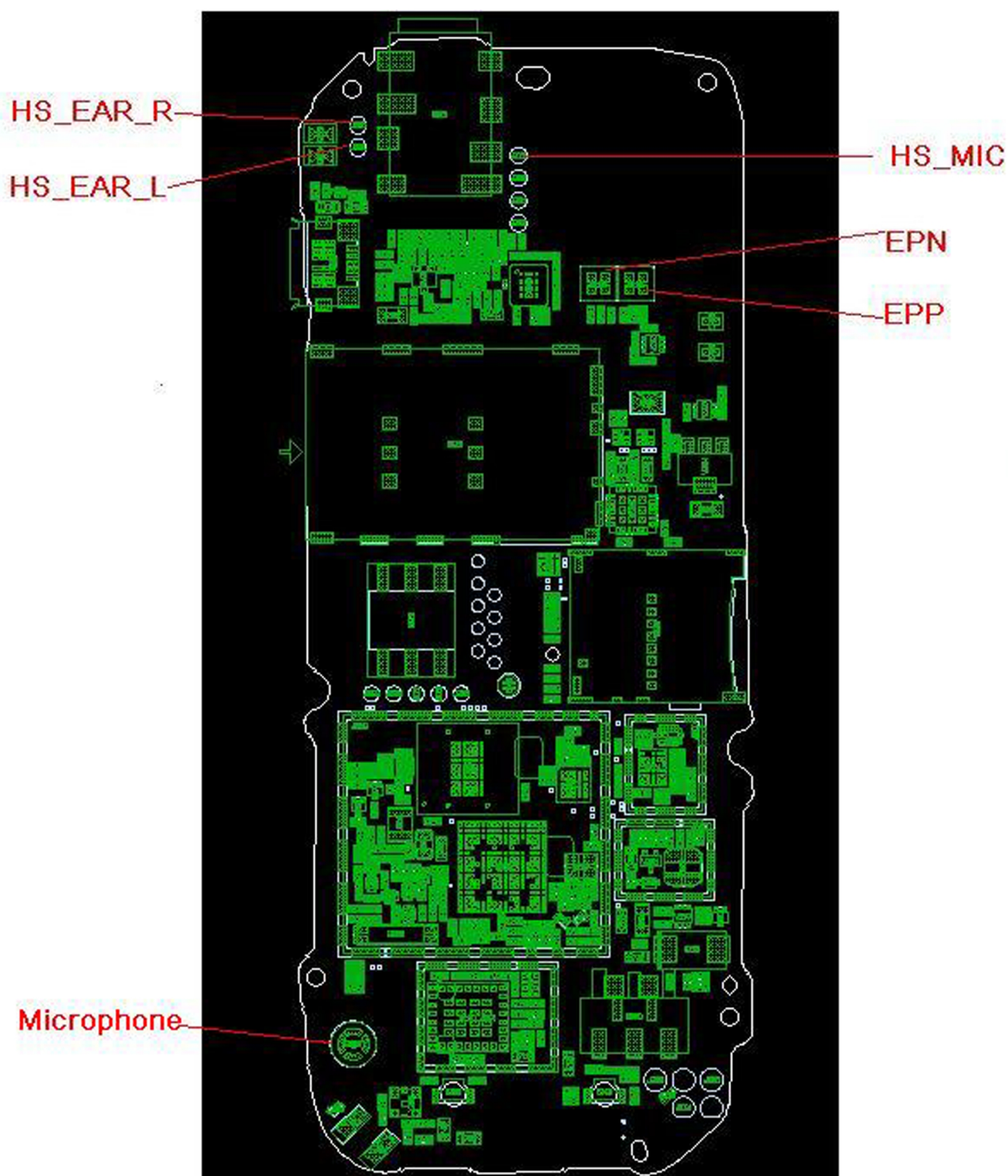
Figure 28 PWB audio test point
