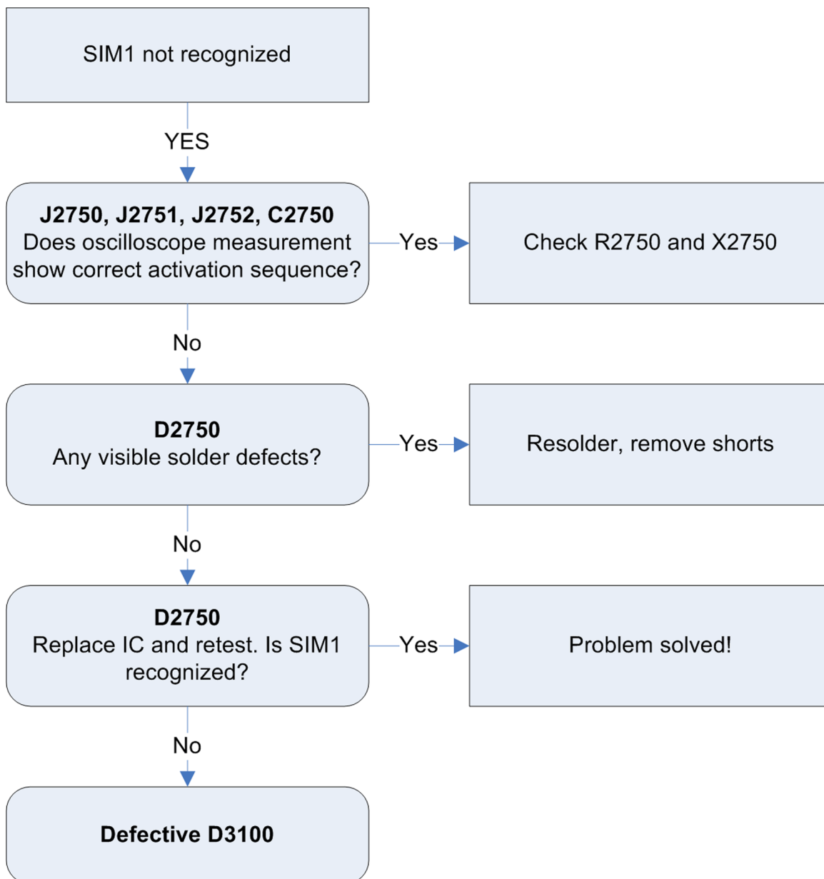
Figure 20 SIM 1 troubleshooting flow
