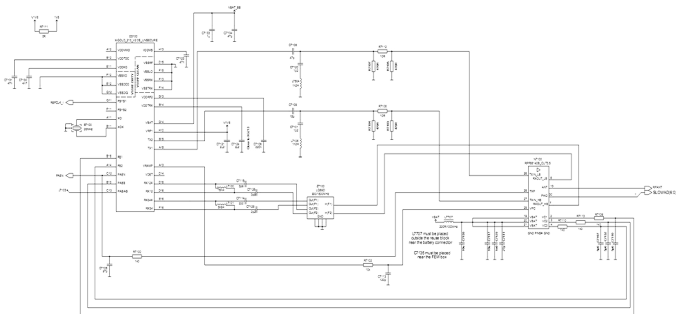
Figure 75 Quantum B2 RF schematic (For Release 3, see Table 2 for components values of the other releases)
