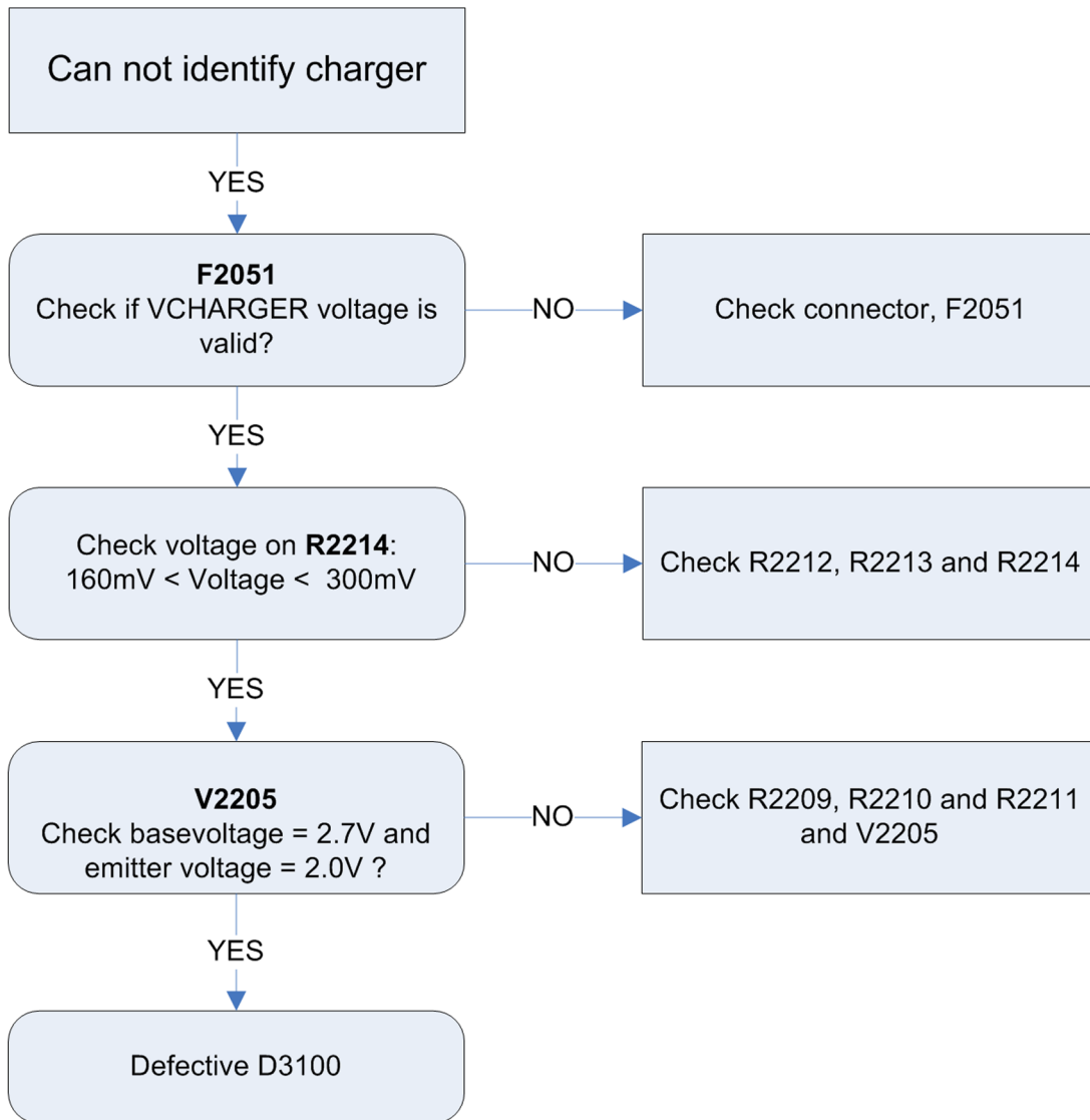
Figure 15 Cannot identify charger
