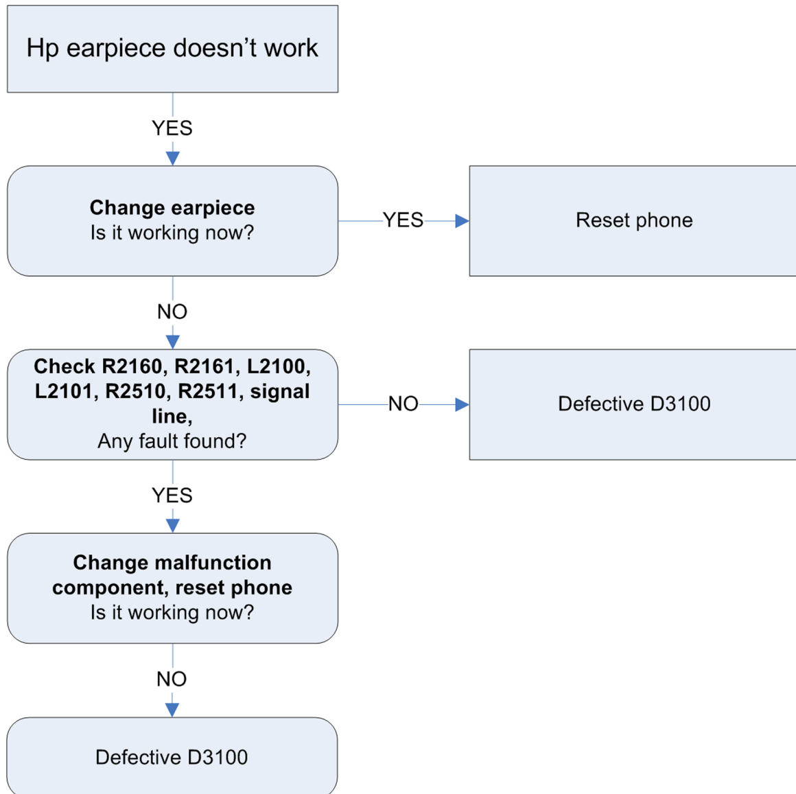
Figure 32 Internal earpiece troubleshooting flow
