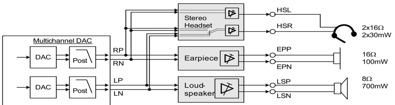
Figure 57 X-Gold213 audio output selection
