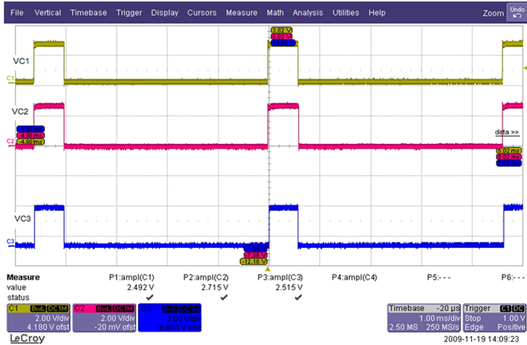
Figure 47 TX HB FEM logic waveform (C1:VC1; C2:VC2; C3:VC3)
