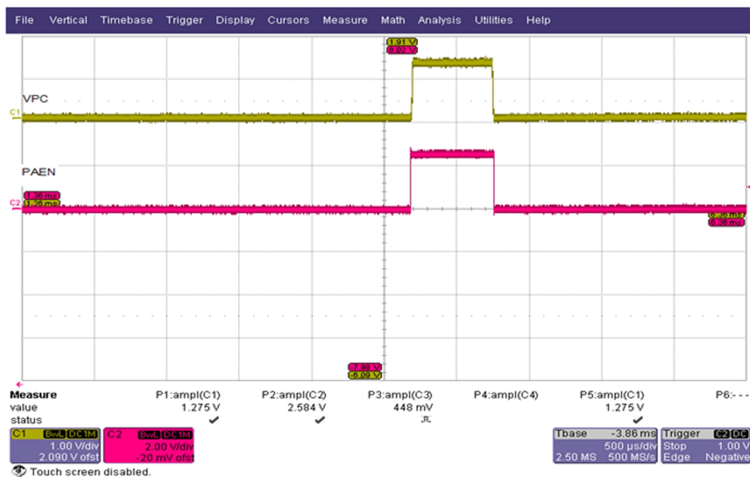
Figure 46 TX LB VPC logic waveform-PCL5 (C1: VPC; C2: PAEN)
