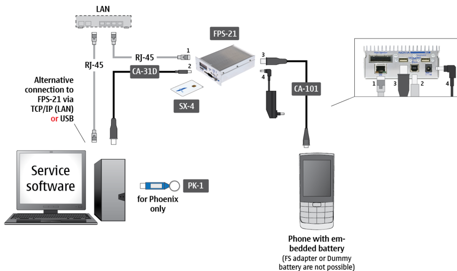
Figure 3 Flashing, certificate restore and product code change
