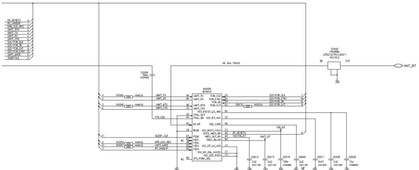
Figure 71 BT circuits
