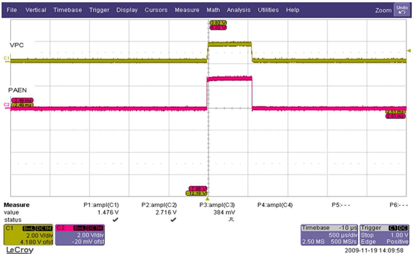
Figure 48 TX HB VPC logic waveform-PCL0 (C1: VPC; C2: PAEN)
