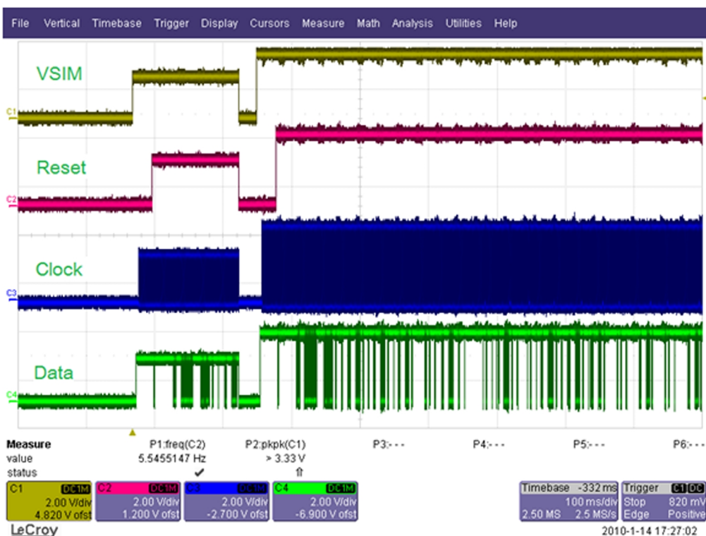
Figure 19 SIM voltages, normal startup at 3V
