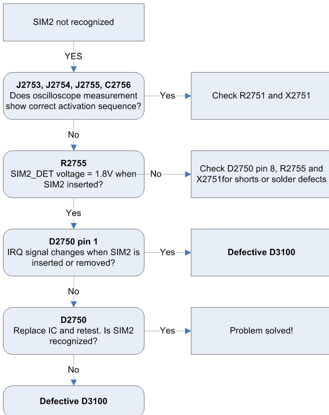
Figure 21 SIM 2 troubleshooting flow
