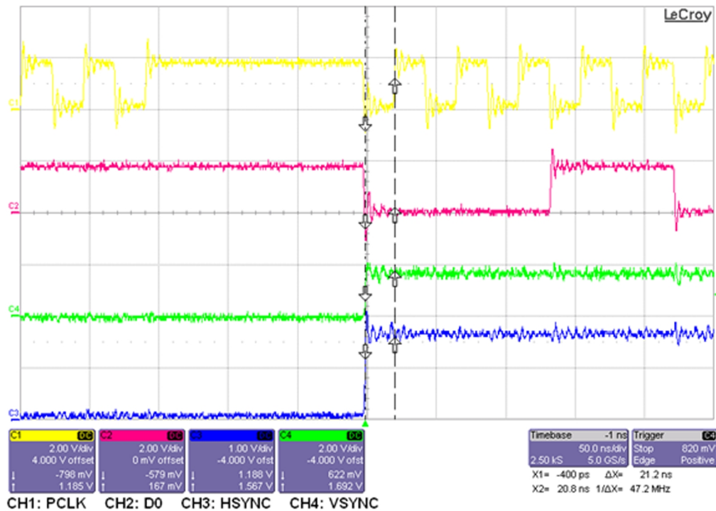
Figure 25 Interface signals between D3100 and N3000
