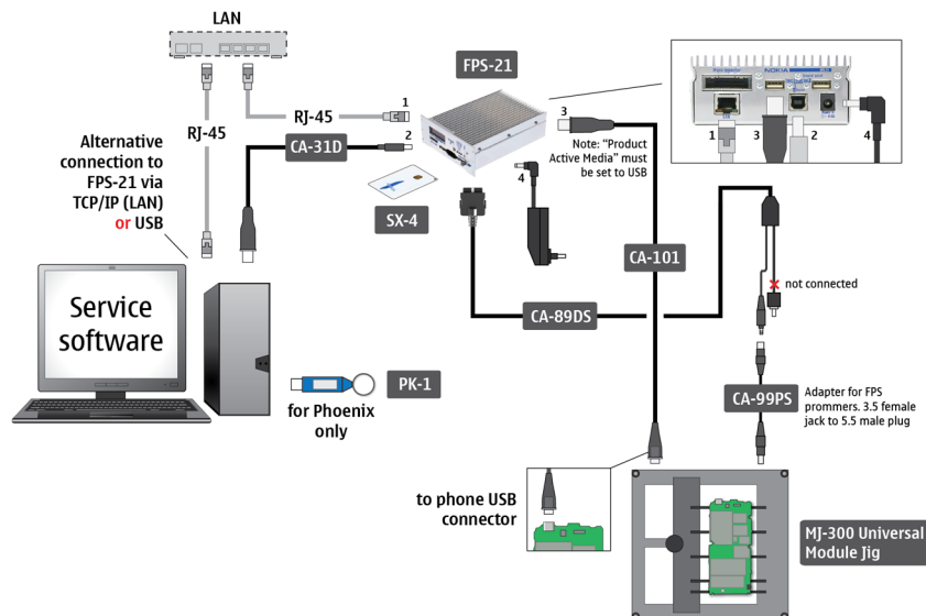
Figure 4 Flashing, certificate restore, product code change and EM calibration
