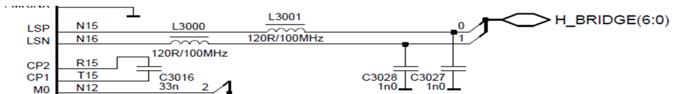
Figure 59 Speaker outputs with ferrite filters
