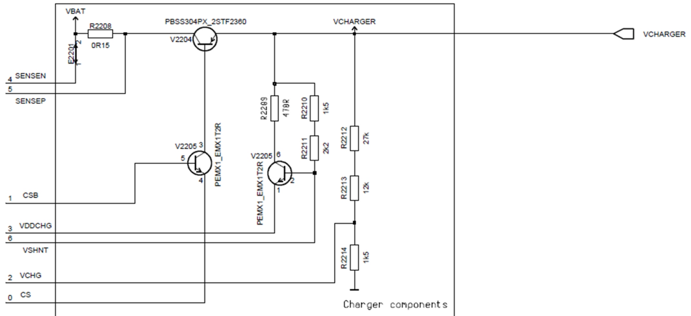
Figure 60 X-Gold213 reference charge circuit
