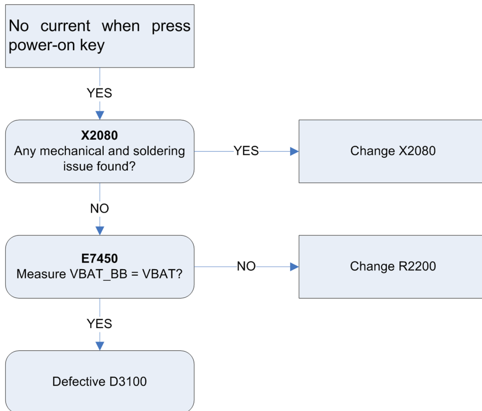
Figure 12 No current when pressing power on key
