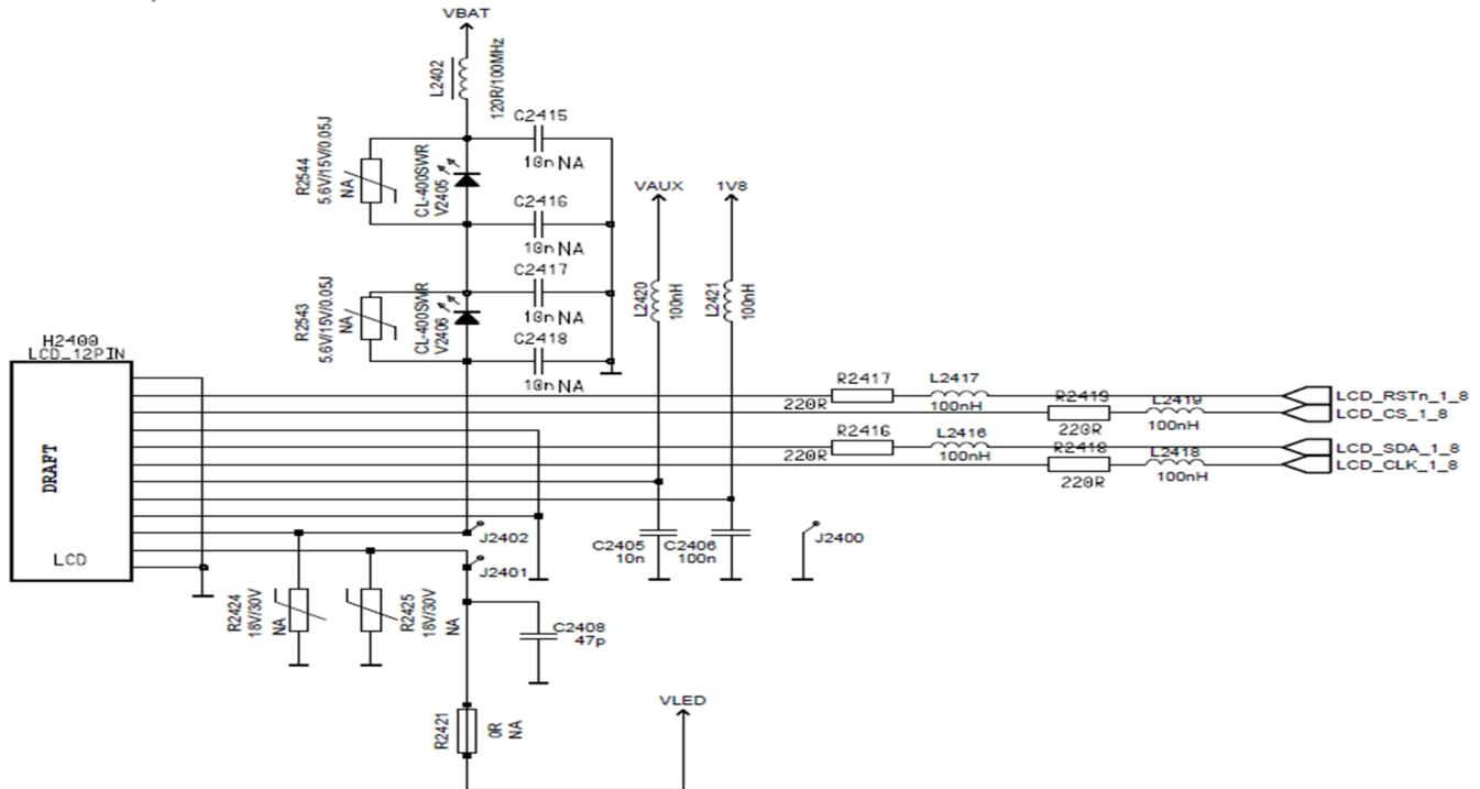
Figure 61 Serial display connection
