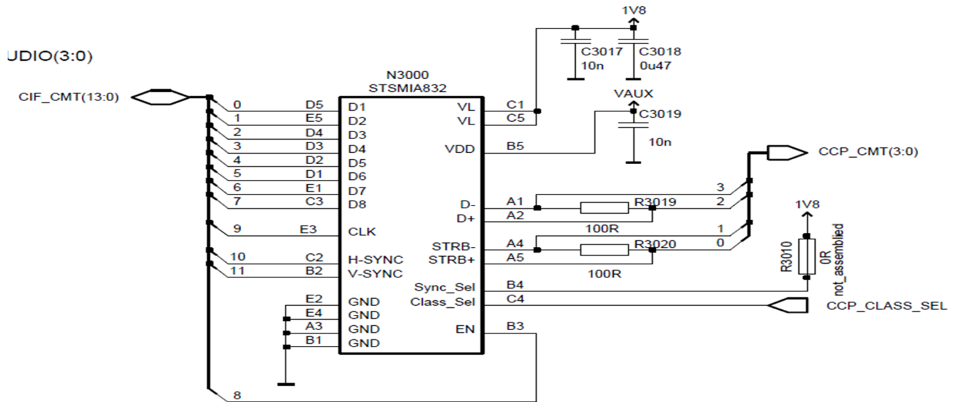
Figure 68 Camera de-serializer for serial camera module
