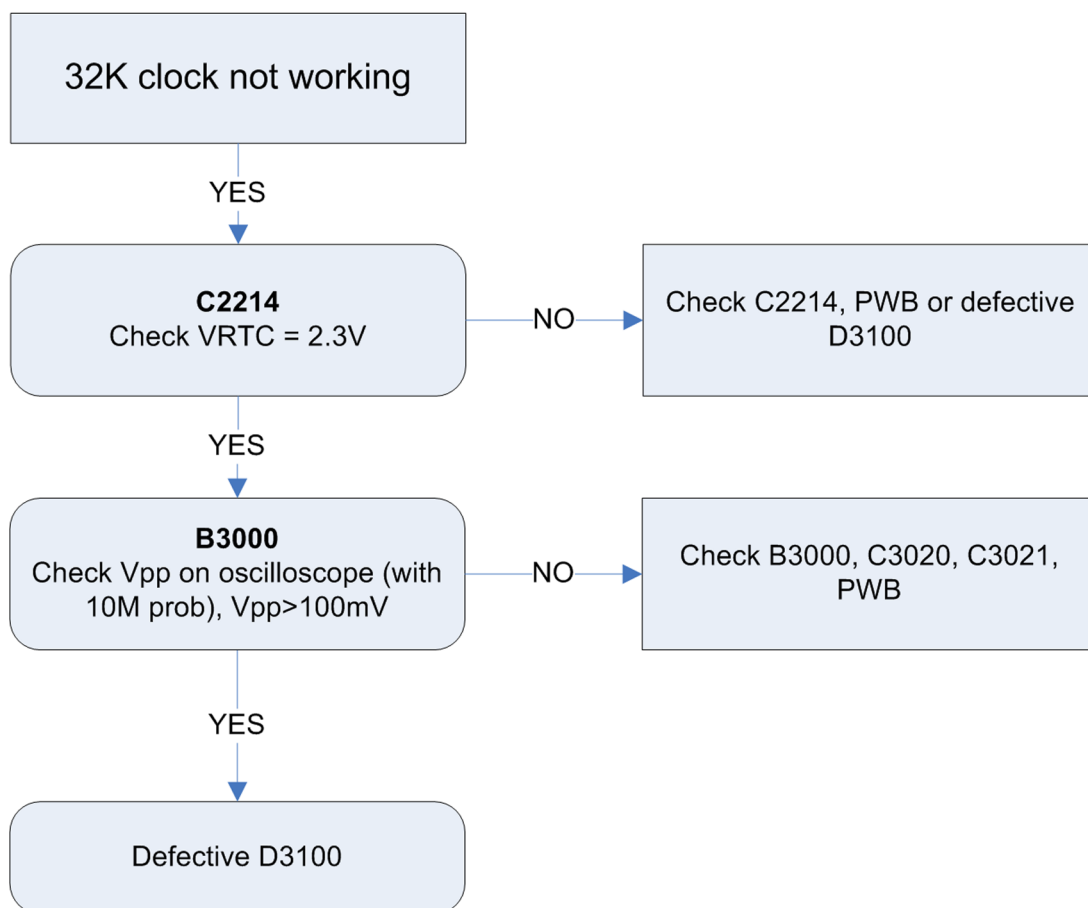
Figure 14 32 KHz RTC clock does not work
