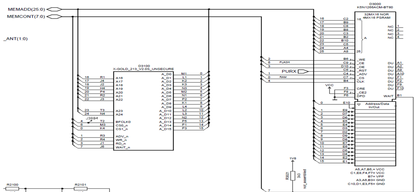
Figure 63 Memory interface connection
