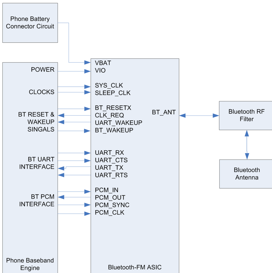
Figure 49 Bluetooth block diagram
