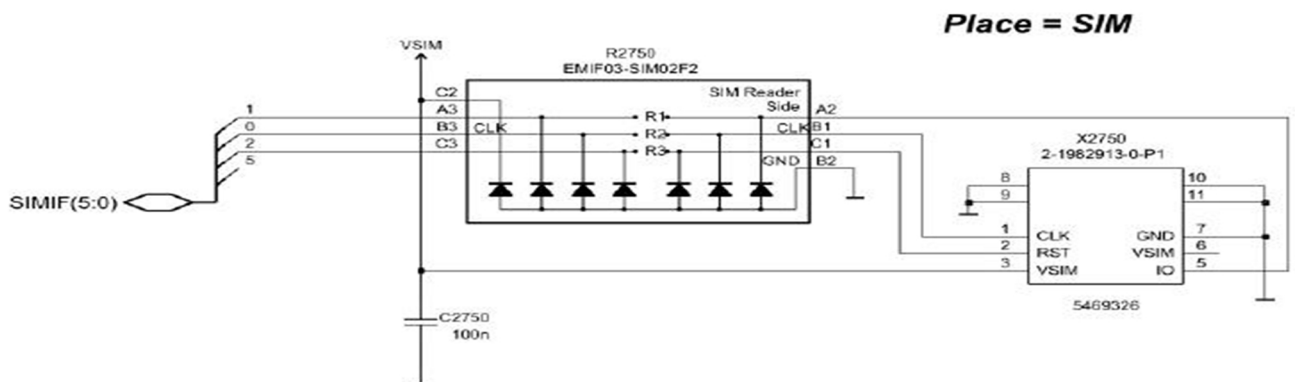
Figure 64 SIM card holder and signal protection
