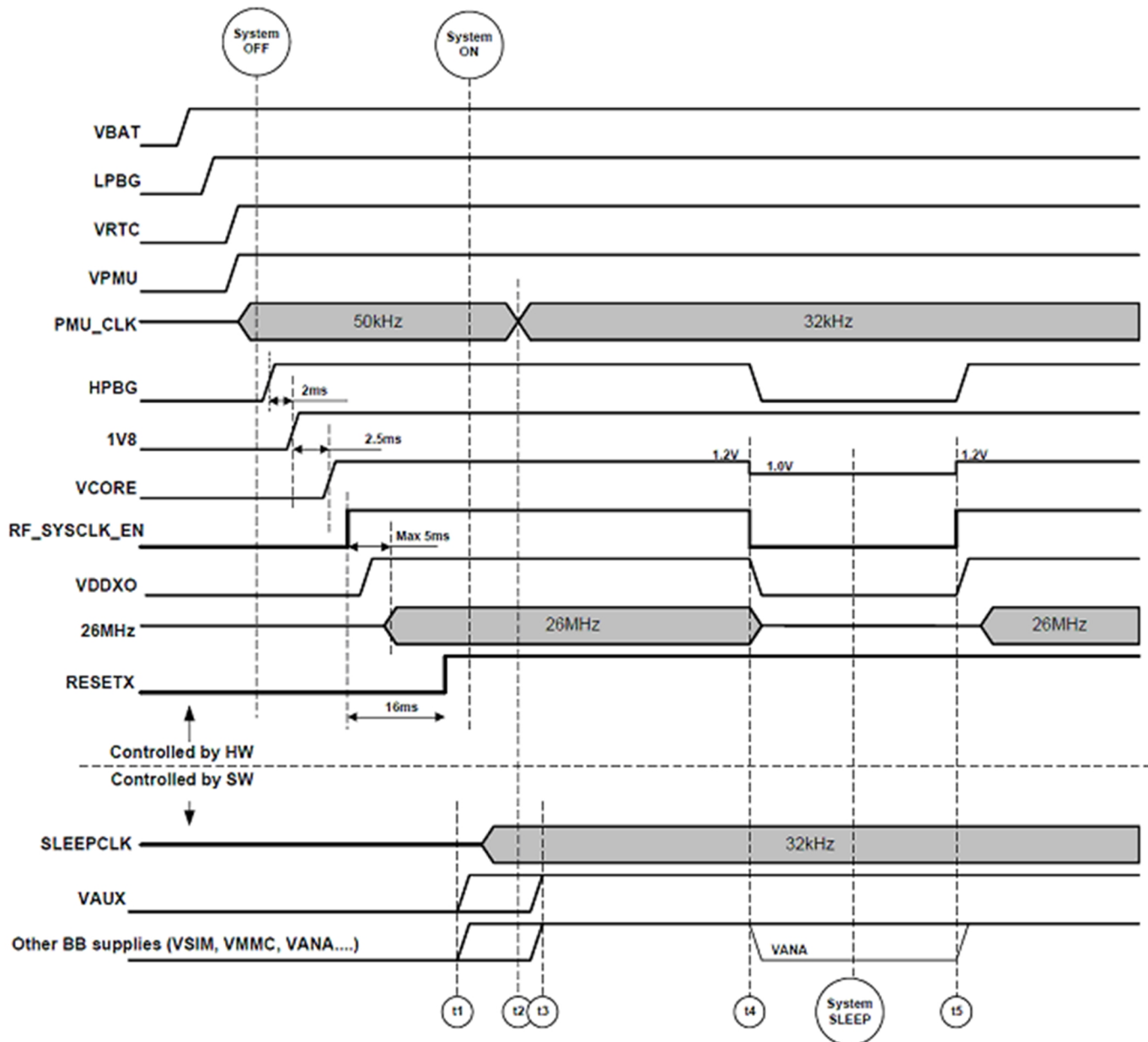
Figure 52 Power up timing and system sleep
