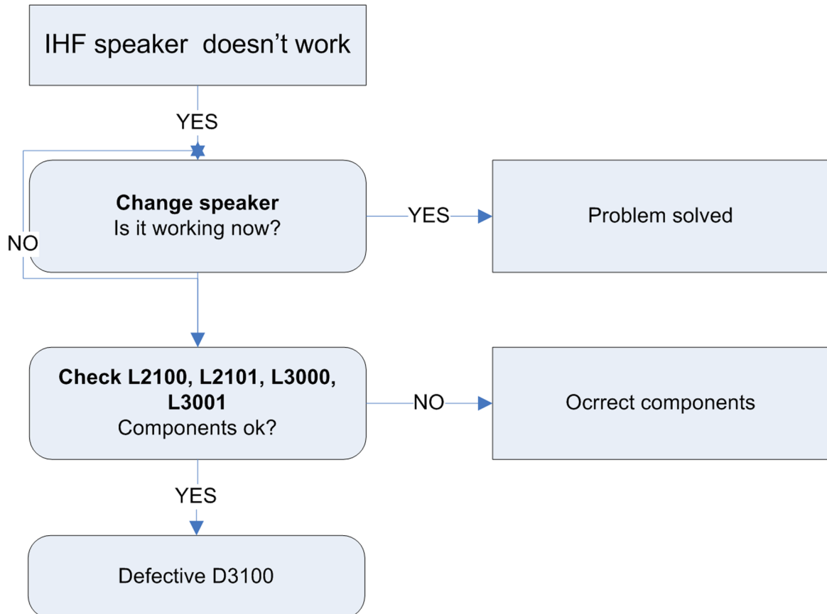
Figure 34 IHF speaker troubleshooting flow
