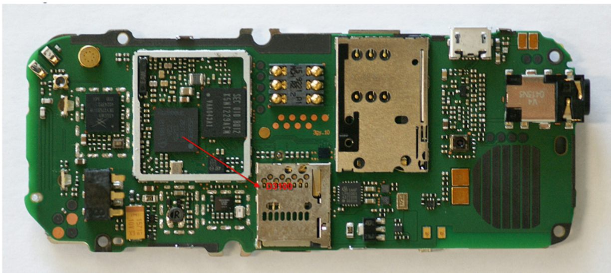
Figure 38 D3100 is the non-reworkable components on PWB
