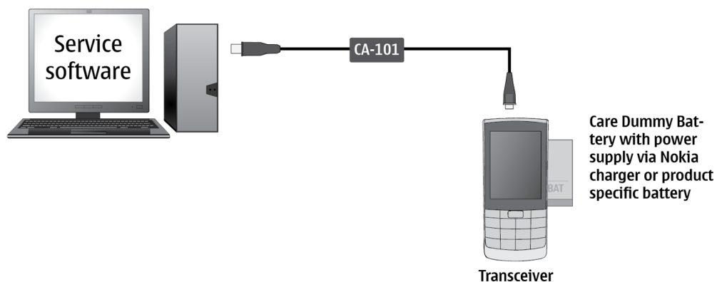
Figure 2 POS flash concept
