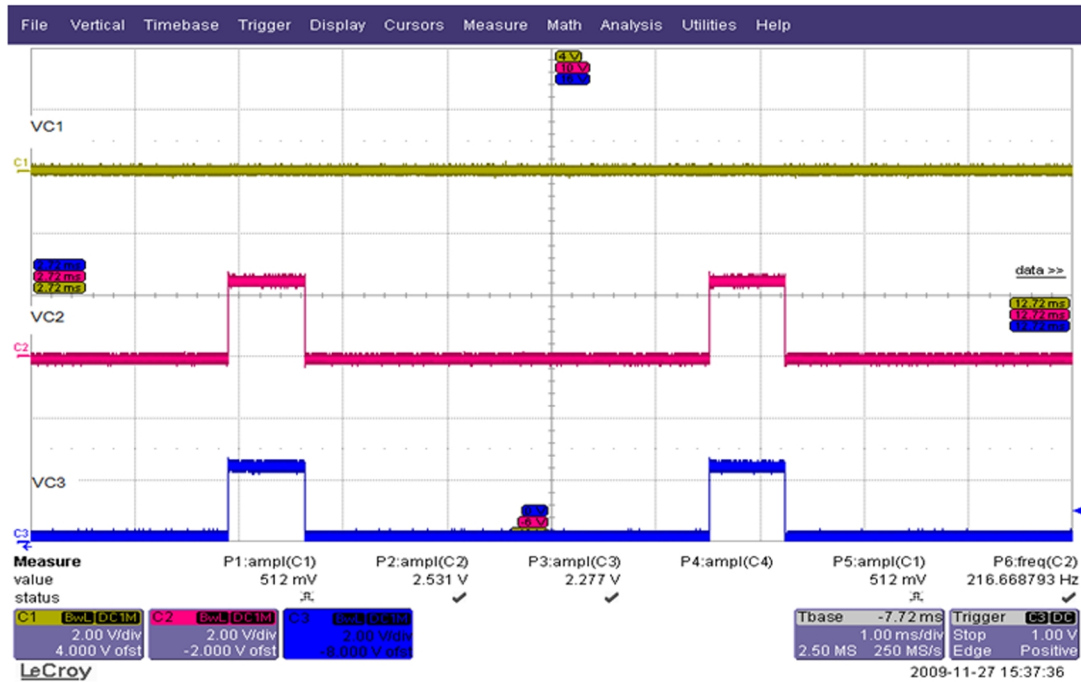
Figure 42 X-Gold RX pin volts @ L7100(LB) / L7101(HB)
