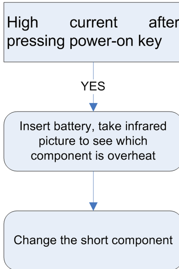
Figure 11 High current after pressing power-on key
