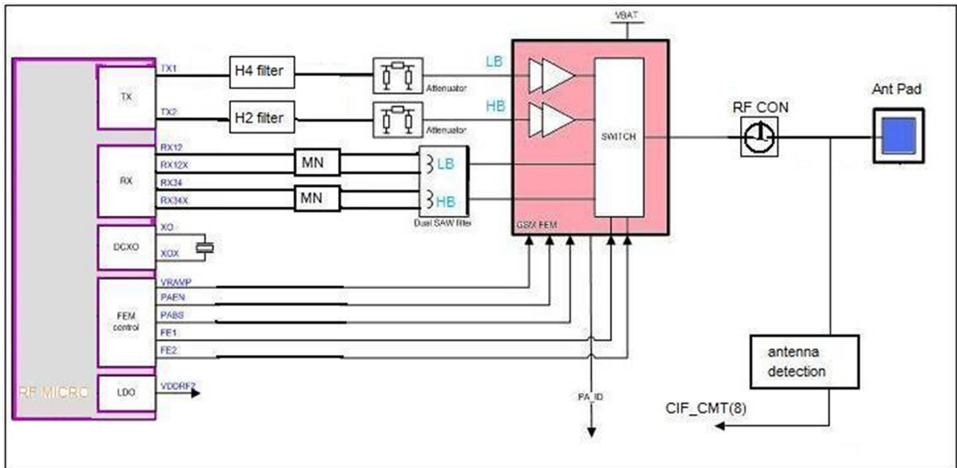
Figure 73 RF block diagram
