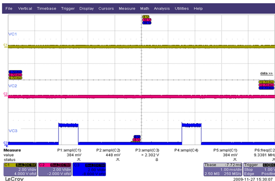
Figure 41 RX LB FEM logic waveform (C1:VC1; C2:VC2; C3:VC3)
