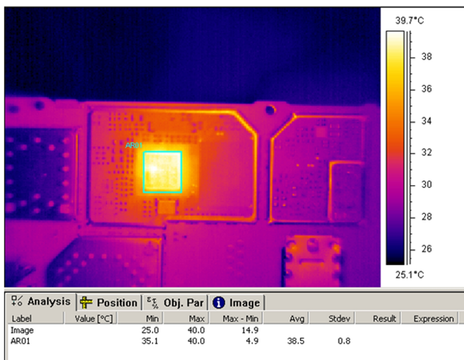
Figure 9 IR picture showing component overheat
