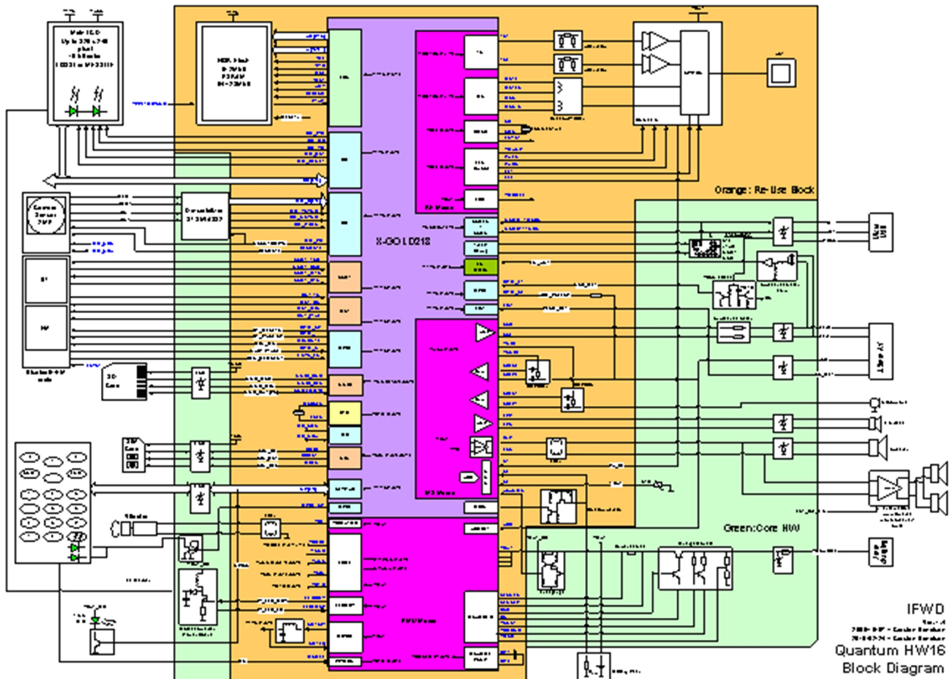
Figure 51 Quantum block diagram
