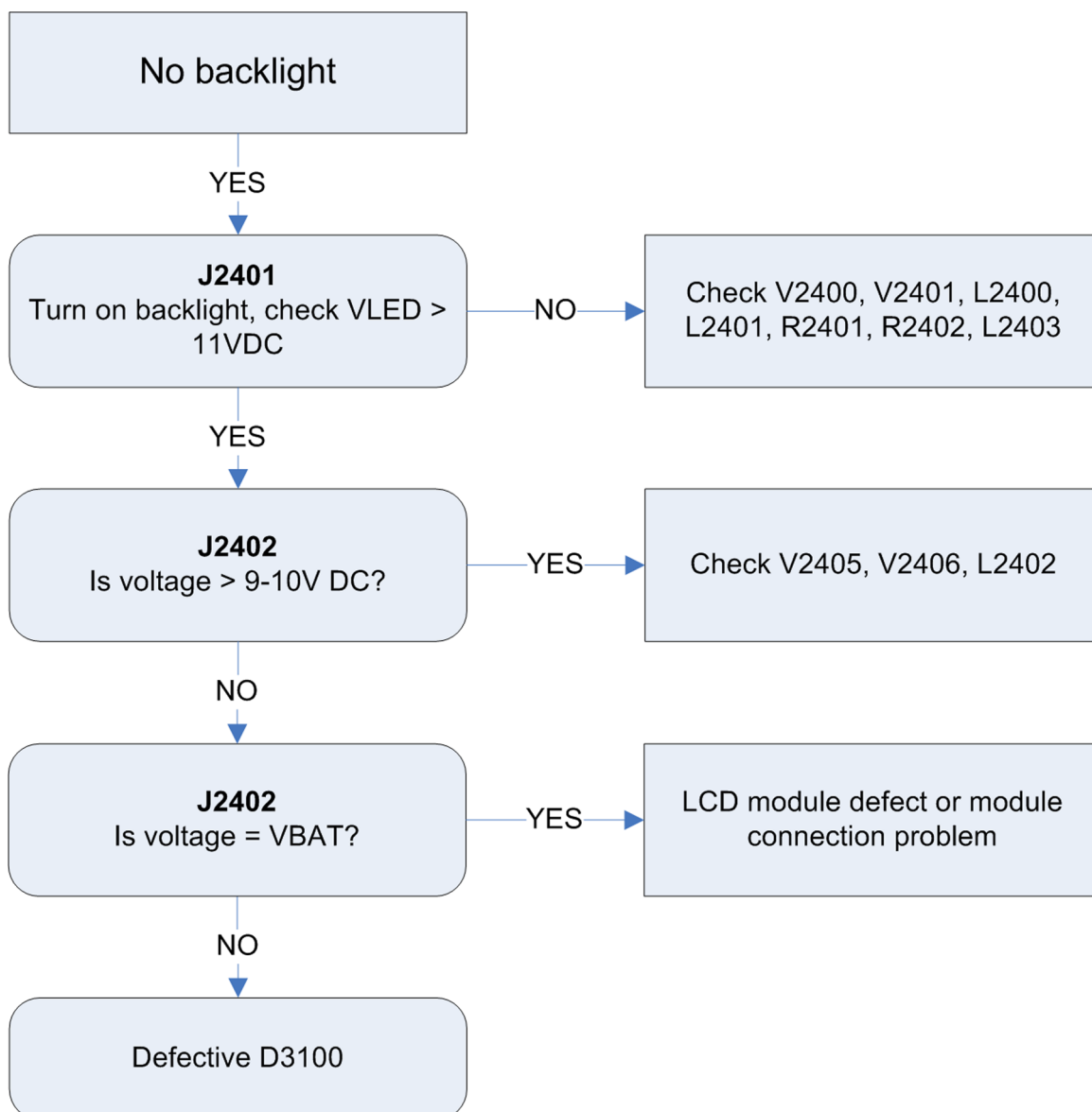
Figure 24 No backlight troubleshooting flow
