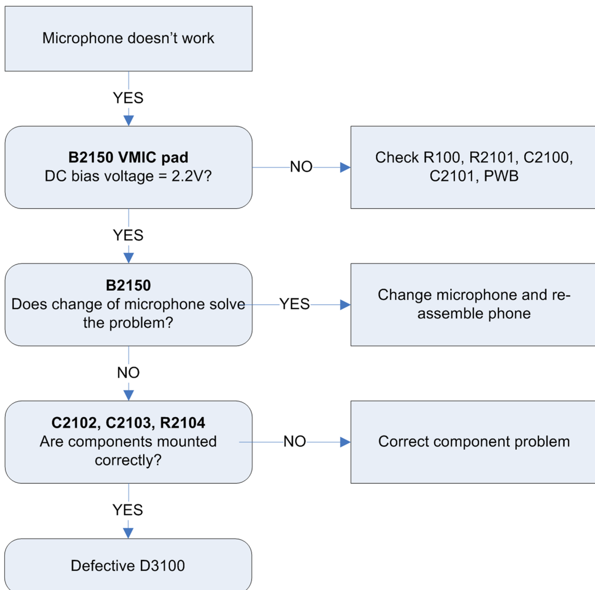
Figure 30 Internal microphone troubleshooting flow
