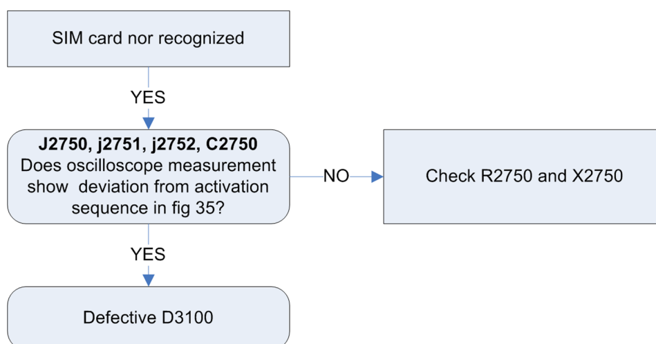
Figure 17 Cannot identify SIM card
