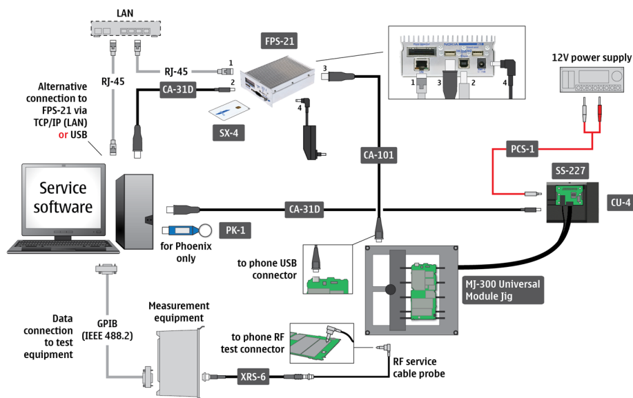
Figure 5 BB and RF tuning
