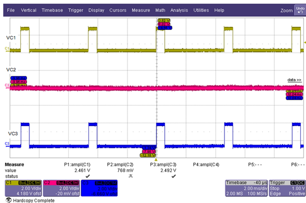
Figure 45 RX LB FEM logic waveform (C1:VC1; C2:VC2; C3:VC3)
