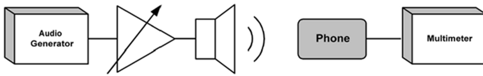
Figure 35 Test arrangement for external microphone
