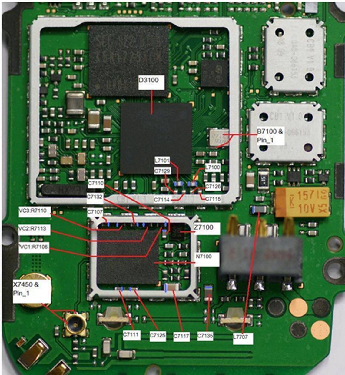
Figure 39 RX checkpoints and component overview (measurement point marked with blue)
