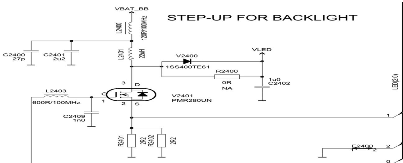
Figure 67 Step-up backlight driver
