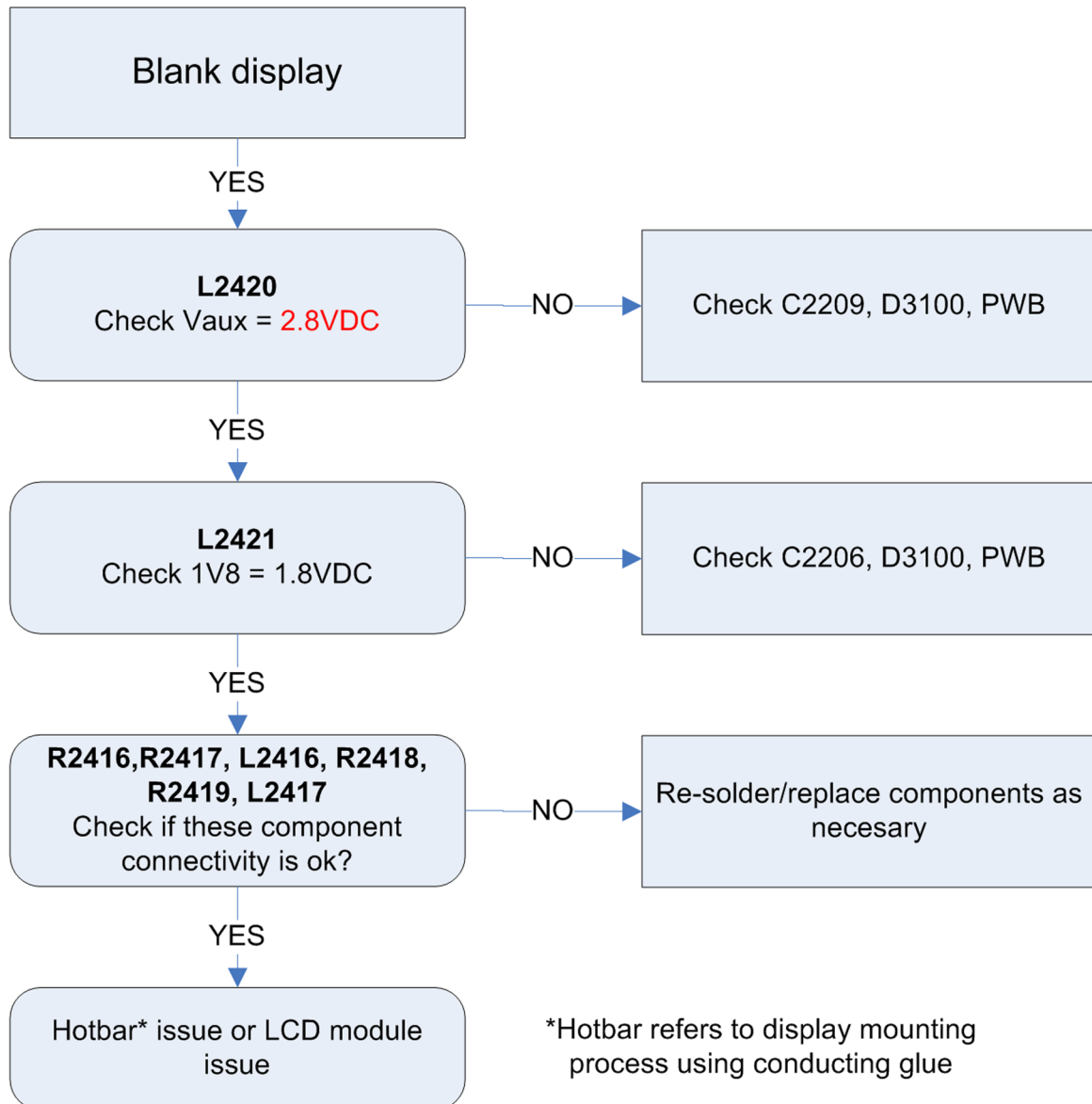
Figure 23 Blank display troubleshooting flow
