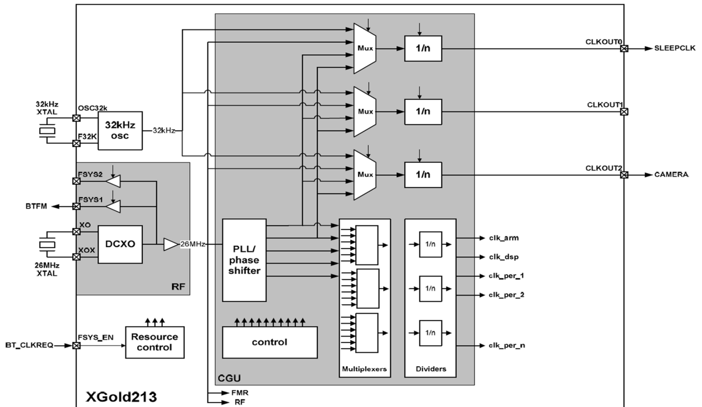
Figure 56 XG213 clock generation and distribution
