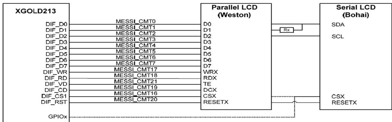
Figure 62 Display interface (parallel and serial coexist)
