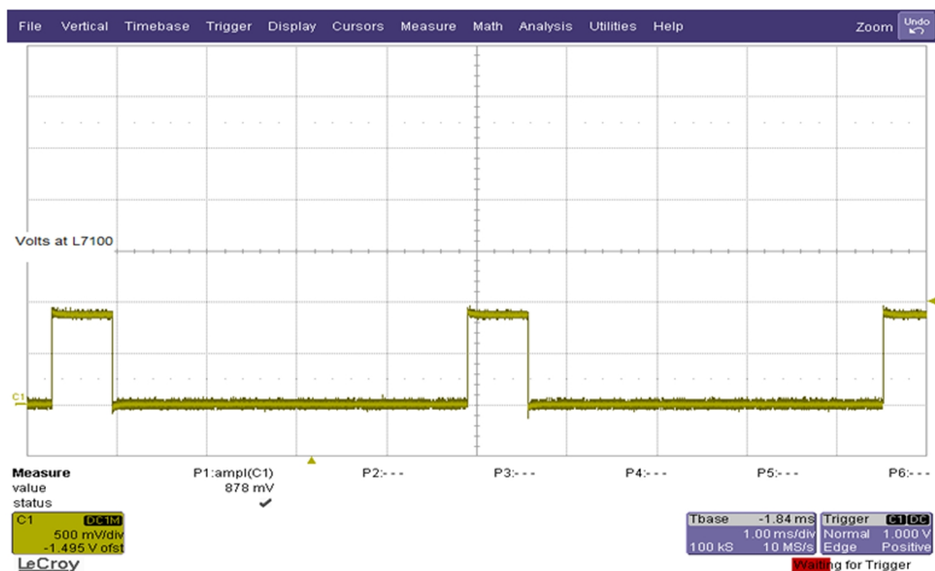
Figure 40 X-Gold RX pin volts @ L7100(LB) / L7101(HB)
