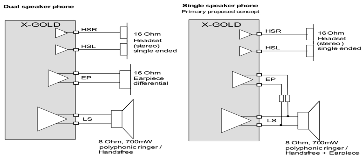
Figure 58 Dual and single speaker configurations
