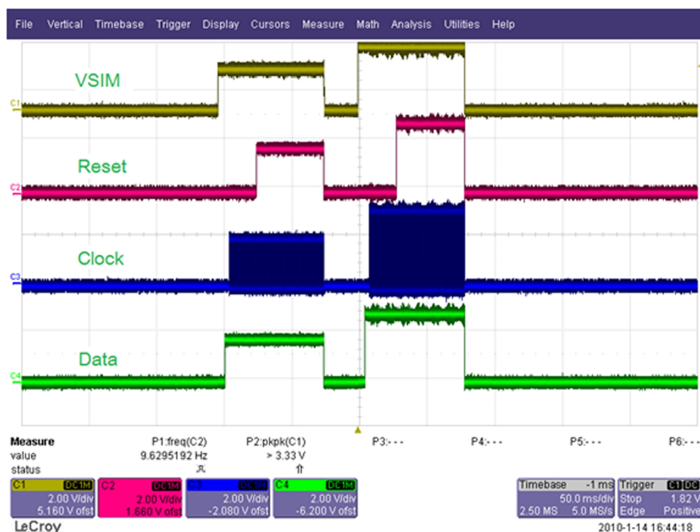
Figure 18 SIM voltages, no ATR
