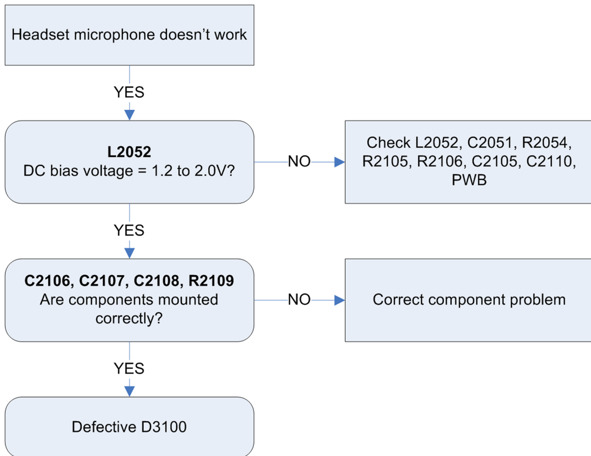
Figure 36 external microphone troubleshooting flow
