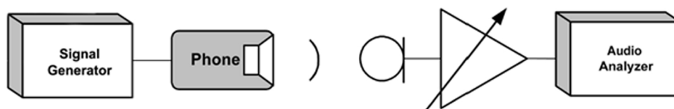
Figure 37 Test arrangement for headset speaker
