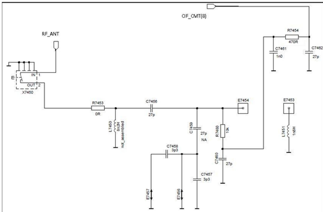
Figure 74 Antenna detection circuit
