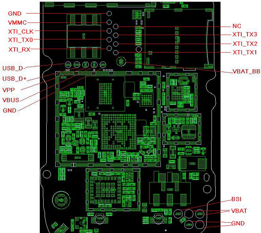
Figure 6 Baseband test point locations
