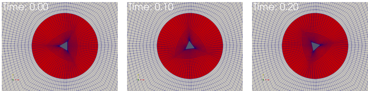
Figure 60: Varying the orientation of the investigated body. Since the body-fitting mesh of the inner domain is in an over-all cylindrical shape, we simply can rotate the inner domain with respect to the outer domain, to change the orientation of the investigated body with respect to the incident flow. After creating the mesh, we can use moveMesh to rotate the inner domain. With appropriate settings for the angular velocity and the write interval, we can get a mesh for any orientation of the triangular prism.
