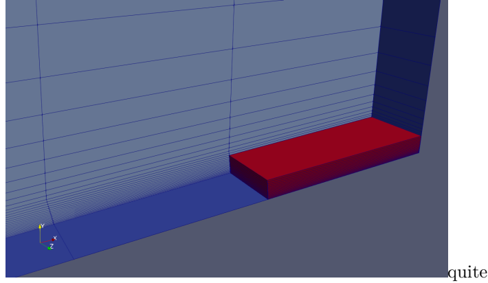
Figure 28: The under-determined cells, which were found by checkMesh in the mesh of an axi-symmetric simulation. These cells are on a far corner of the 2-D domain, and grading towards the more interesting regions led them to have a high aspect ratio. In fact, these cells have the highest aspect ratio of the whole mesh. The proximity to the lower wall results in these cells to be quite fine in the y -direction. Since, these cells are furthest from the axis of symmetry, they are relatively large in radial and tangential direction.
