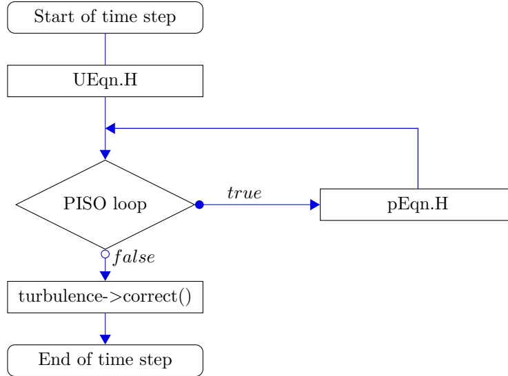
Figure 71: Flow chart of the PISO algorithm
