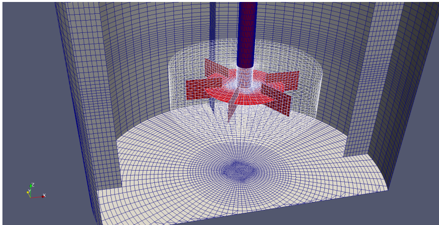
Figure 65: A baffled stirred tank with a Rushton impeller. The stator patch is shown in grey and the rotor patch is shown in red. The white wireframe shows the boundary of the rotor zone. For all cells of the rotor zone the MRF method is applied.
