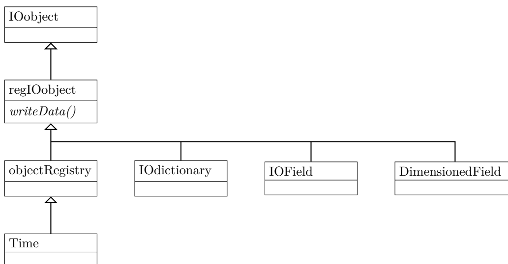
Figure 91: A partial view of the class hierarchy involving regIOobject ; note that this diagram is complete only for the classes IObject and regIOobject – meaning IObject is not derived from any other class and regIOobject is derived from only IObject ; the other classes have more base classes than shown in this diagram.
