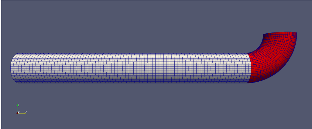
Figure 31: A cheap 90° pipe bend. The outlet patch of the original mesh was extruded along the sector of a circle.
