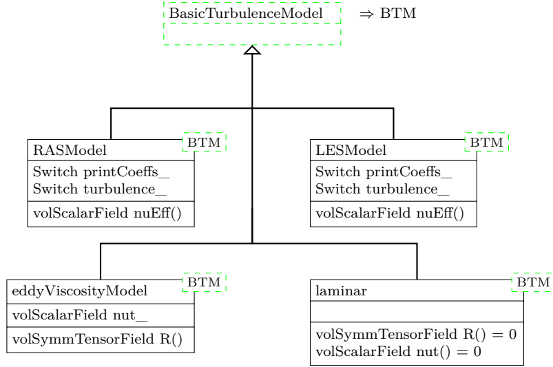
Figure 54: The class hierarchy of the elementary turbulence models of the new turbulence model framework. Note the shorthand notation BTM for the class BasicTurbulenceModel .
