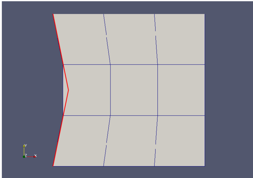
Figure 5: A block with a poly-line at the left side. The red line indicates the poly-line. This figure makes it obvious that edges defines in the blockMeshDict serve to compute the locations of the block's internal nodes. The block itself however, does not obey the poly-line.
