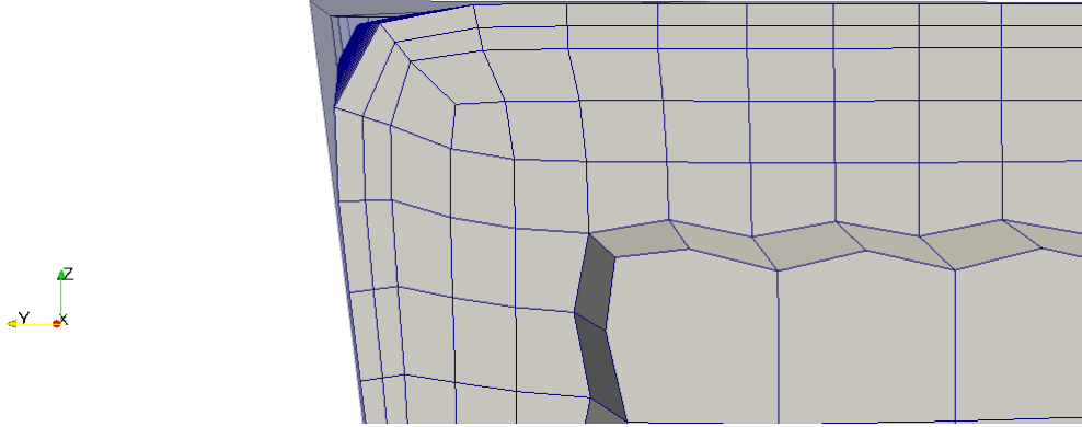
Figure 20: Poor feature edge resolution caused by not providing information on feature edges. Note, the whole geometry is bounded by a single patch.
