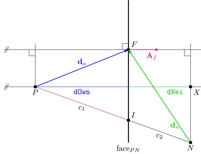
Figure 24: Definition of skewness of internal faces
