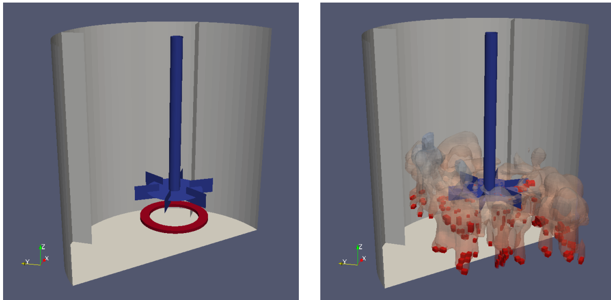
Figure 47: Left: The cut-away of the walls of a stirred tank with the rotor (blue) and the aeration device (red). The aeration device is a cellZone on which source terms are applied via the fvOptions mechanism in OpenFOAM-2.3.x.
