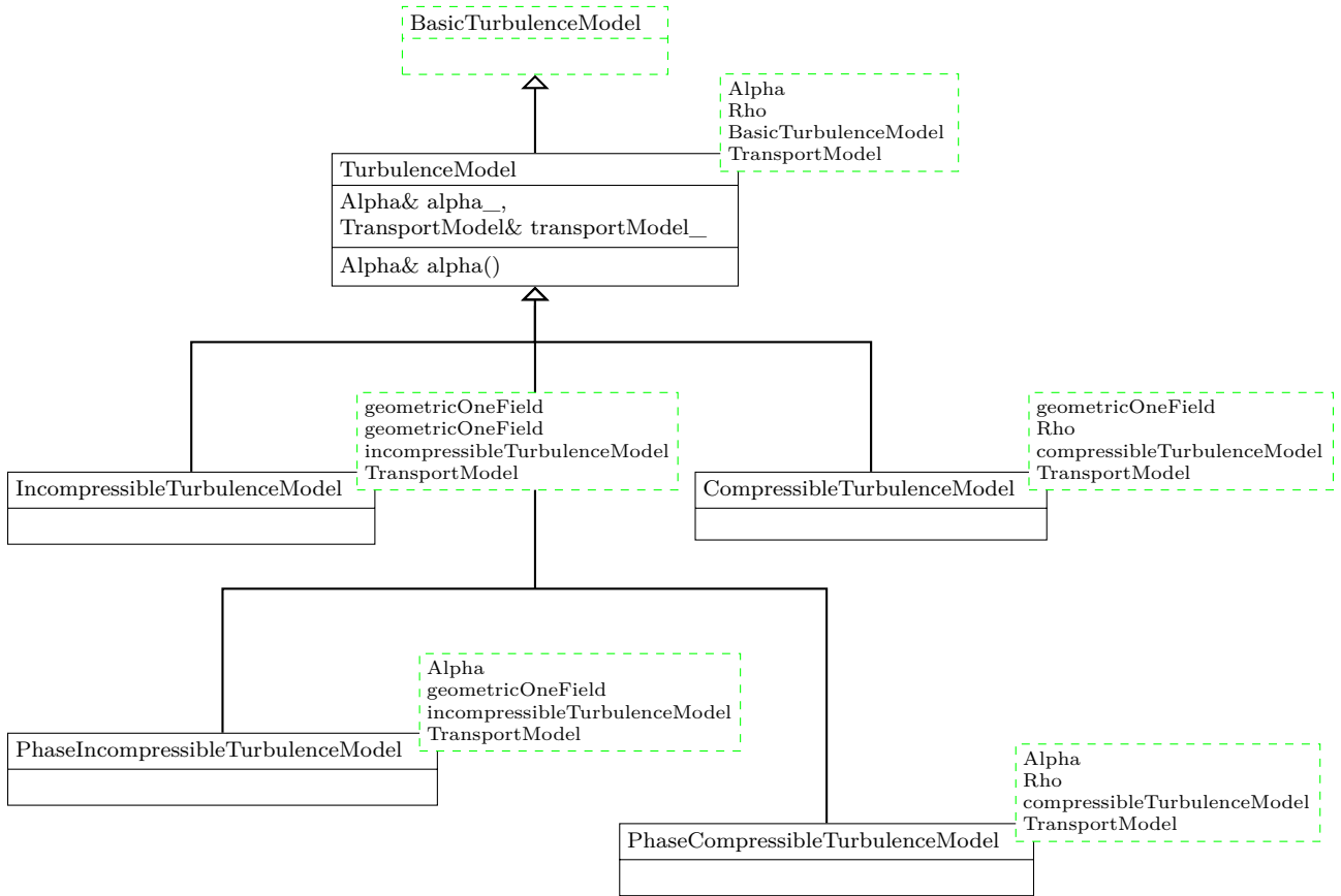
Figure 53: The base class TurbulenceModel has four template parameters and it is derived from one of its template parameters. Note, that the four derived classes – the four incarnations of the turbulence model – differ in the template parameters.
