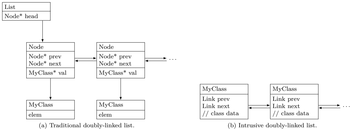
Figure 66: Schematic diagrams of doubly-linked lists.
