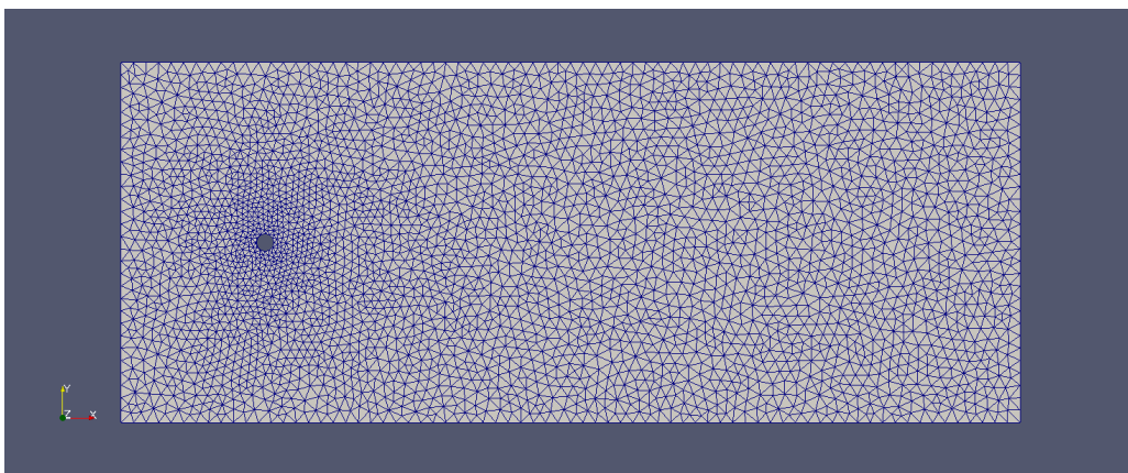
Figure 30: The mesh for a 2D study generated from an STL surface.
