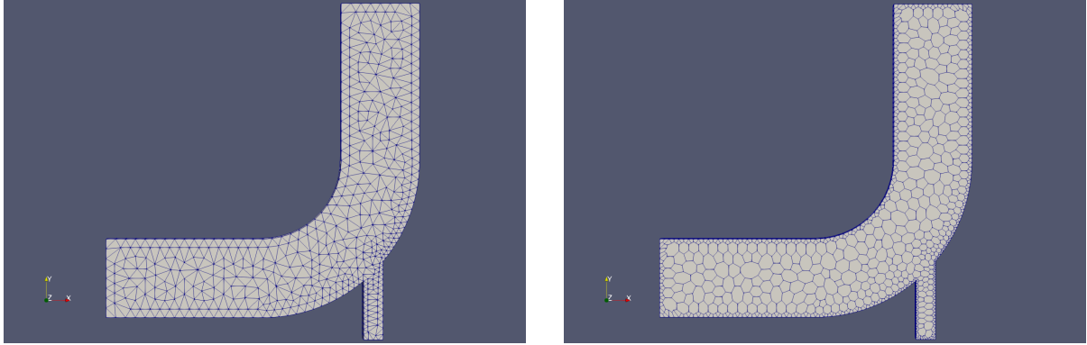
Figure 36: The mesh of the elbow tutorial case; before and after the application of polyDualMesh .
