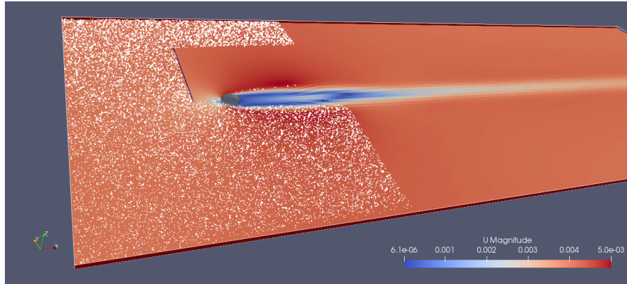
Figure 69: A set of polygons has been defined to count and remove traversing particles. In this case of a cylinder in laminar cross-flow, particles are inserted through the inlet patch. The ParticleCollector cloud function object was set to remove all counted particles, which is clearly visible in this snapshot.
