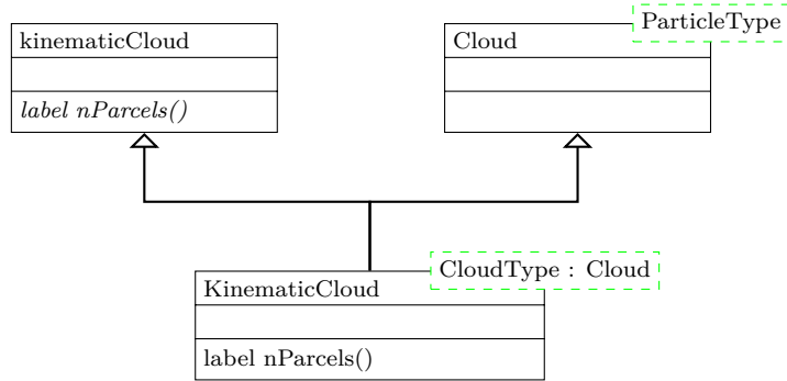
Figure 68: The class hierarchy of the class basicKinematicCloud .
