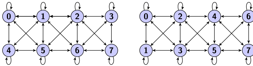
Figure 45: The connectivity graph of our mesh.
