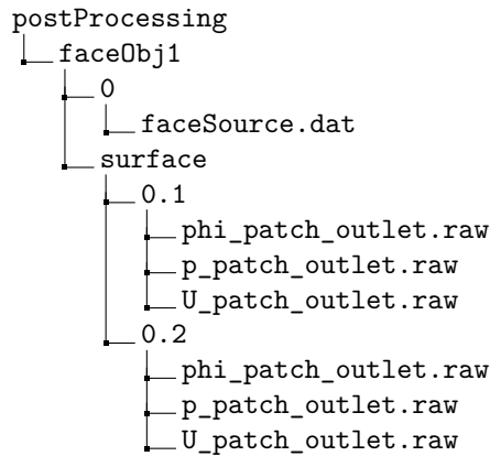
Figure 80: The content of the postProcessing folder
