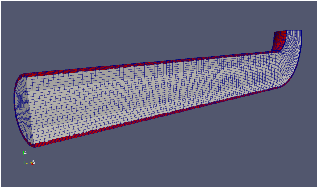
Figure 33: Grow a wall! The walls patch of the pipe mesh was extruded using the linearNormal model.
