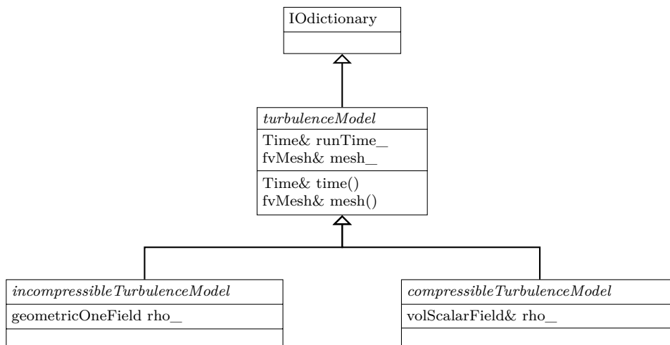
Figure 52: The class hierarchy of the basis of the new turbulence model framework.
