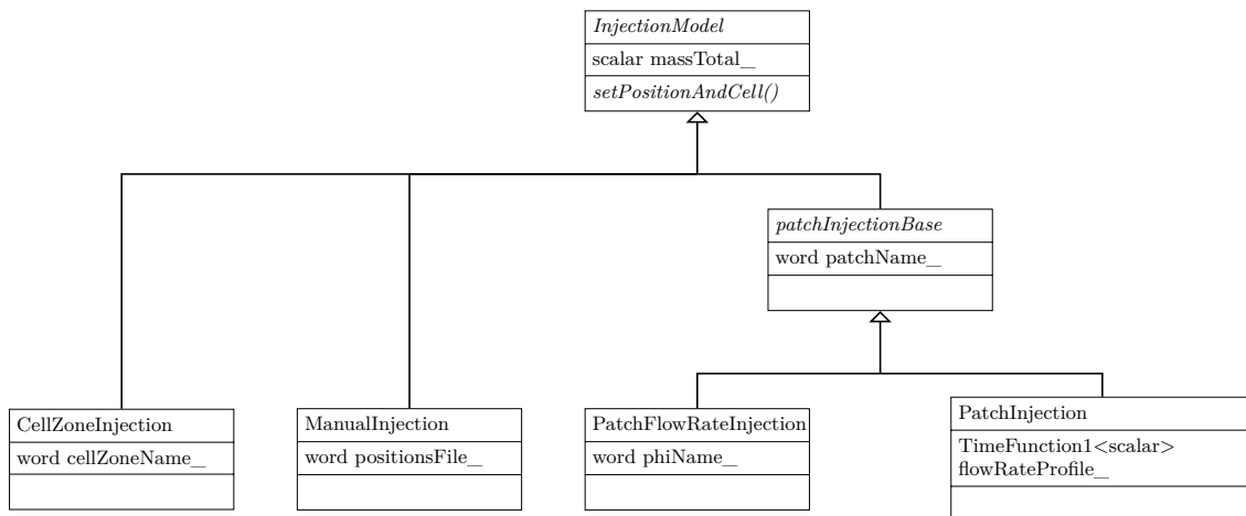
Figure 89: Class hierarchy of some injection models for Lagrangian particles. An intermediate base class is used to reduce code duplication from closely related, yet different injection models.
