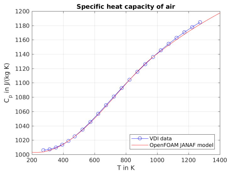
Figure 56: Specific heat capacity C_p of air computed with the JANAF model compared to data from [51].
