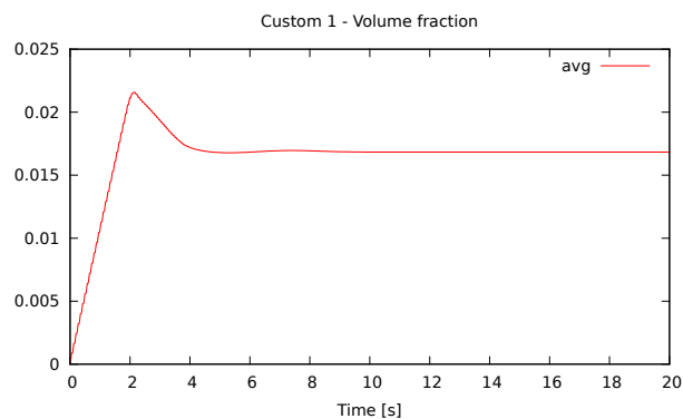
Figure 85: The average volume fraction plotted with pyFoamPlotWatcher and a custom regular expression
