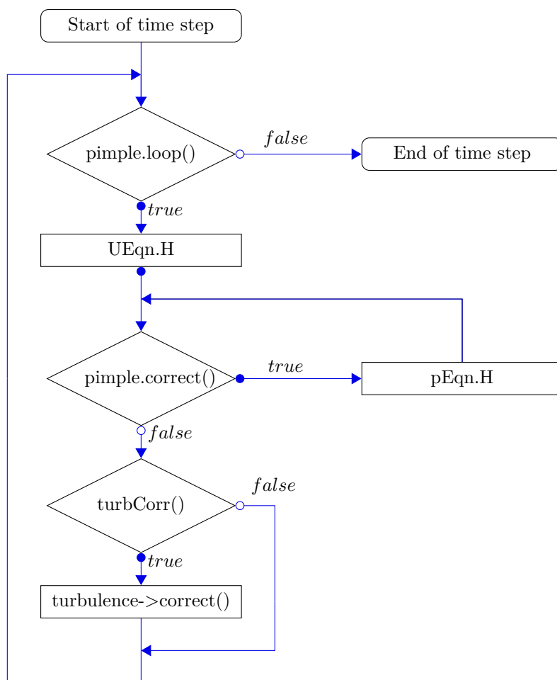
Figure 72: Flow chart of the PIMPLE algorithm
