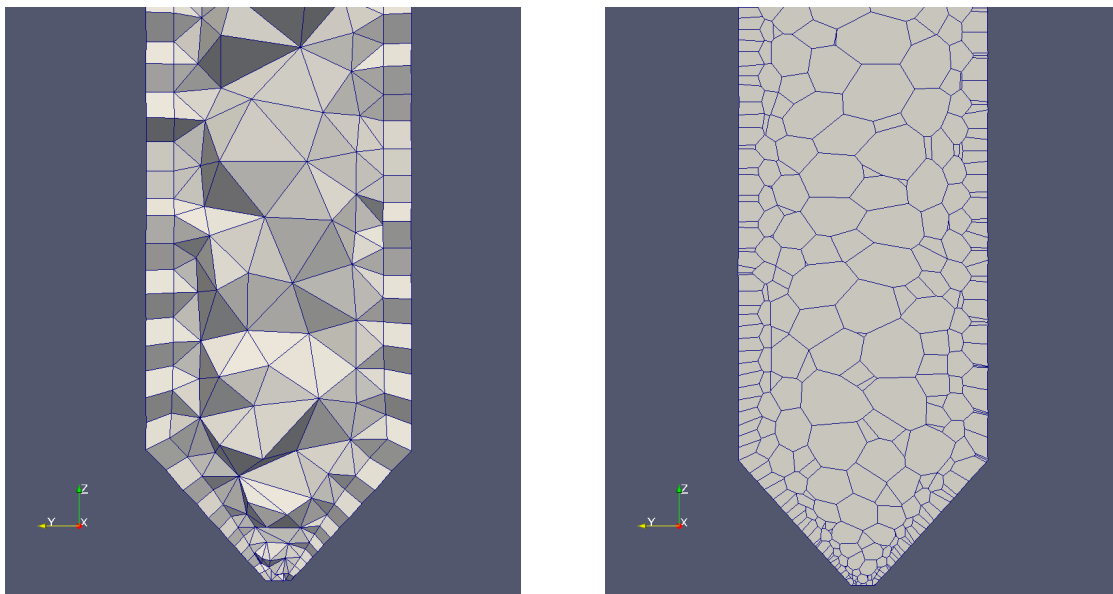
Figure 41: Meshes by enGrid: left : tet-mesh with prismatic boundary layer, right : polyhedral mesh with boundary layer.
