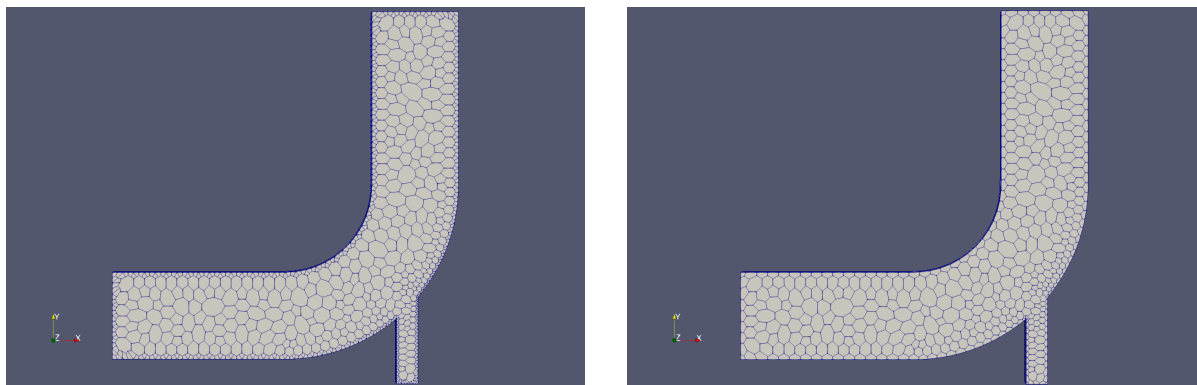
Figure 38: The dual mesh of the elbow tutorial case; before and after the application of combinePatchFaces .
