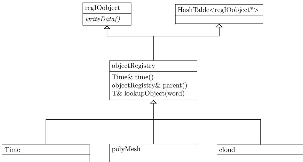
Figure 92: The base classes of the class objectRegistry ; this class is derived from regIOobject and a HashTable ; note that the template parameter of the HashTable is a pointer to regIOobject ; thus objectRegistry is an regIOobject as well as a HashTable of regIOobject pointers – this is C++'s template madness and inheritance wizardry in action.
