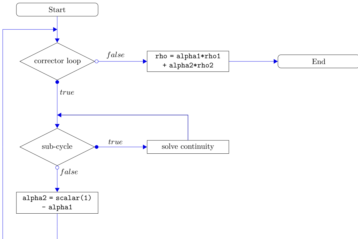
Figure 74: Flow chart of the operations in alphaEqn.H
