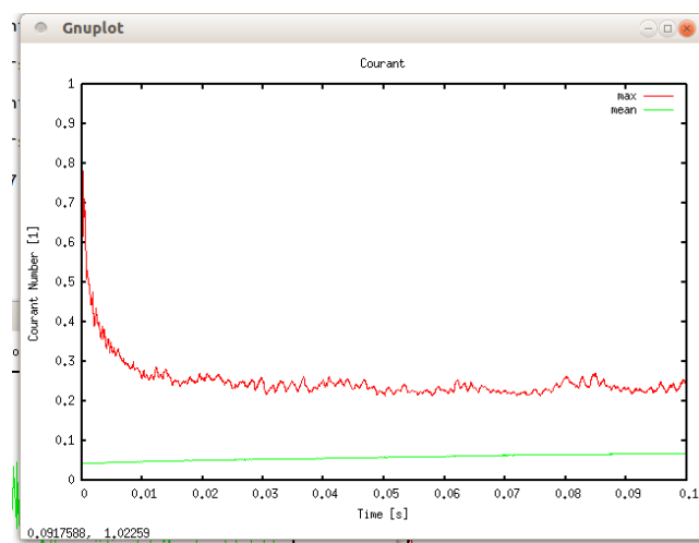
Figure 83: The Courant number plotted with pyFoamPlotWatcher .
