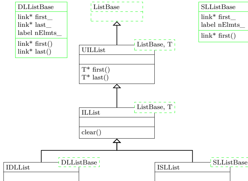
Figure 67: The class hierarchy needed for intrusive lists of objects of type T ; this diagram can be regarded as a subset of the class diagram for singly- and doubly-linked lists, both classic and intrusive.
