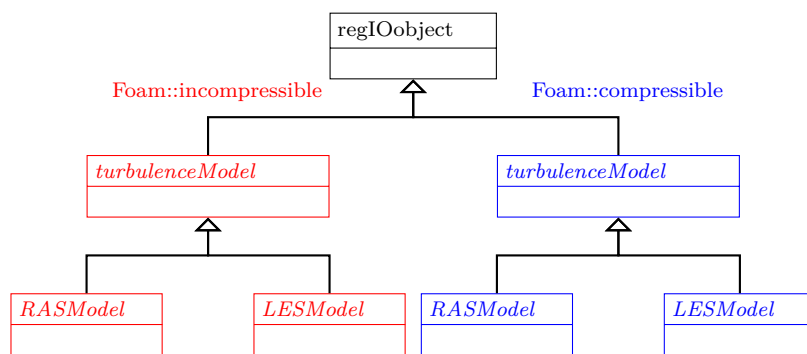
Figure 51: The class hierarchy of the basis of the old turbulence model framework. The namespaces Foam::incompressible and Foam::compressible are indicated by the colours red and blue.
