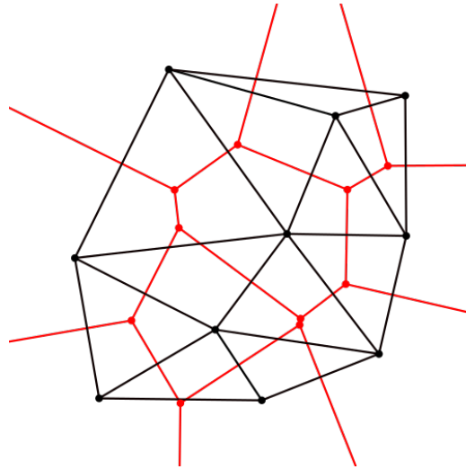
Figure 35: Connecting the centers of the circumcircles produces the Voronoi diagram (in red). Source https://commons.wikimedia.org/wiki/File:Delaunay_Voronoi.svg .
