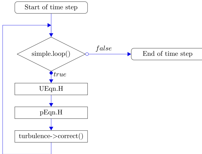
Figure 70: Flow chart of the SIMPLE algorithm
