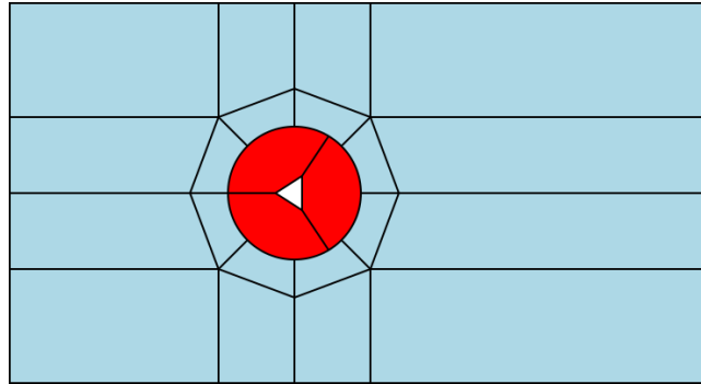
Figure 59: Our simulation domain. The block structure of outer domain, in blue, does not match the block structure of the inner domain, in red. However, by keeping the two regions separate, we can mesh each region individually, which is fairly easy, and use AMI to essentially connect the two regions. After meshing, we can rotate the inner domain with respect to the outer domain to change the orientation of the triangle in the center of the inner domain.
