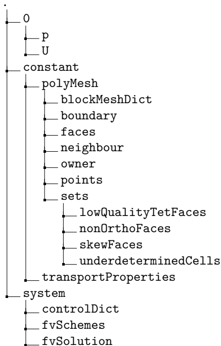
Figure 29: Sets created by checkMesh in the sets directory.
