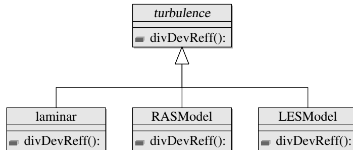
Figure 93: Graphic representation of inheritance of the turbulence model classes.
