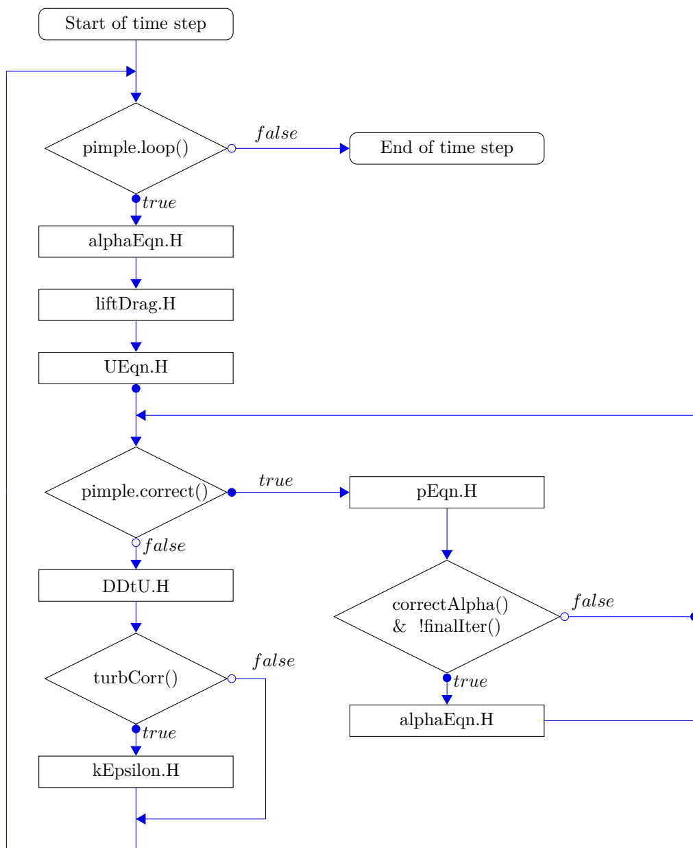
Figure 73: Flow chart of the main loop of twoPhaseEulerFoam
