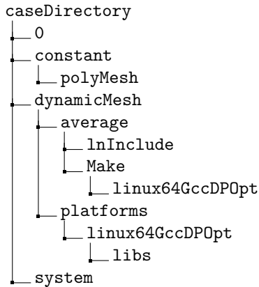
Figure 81: Directory tree after compilation of a coded functionObject
