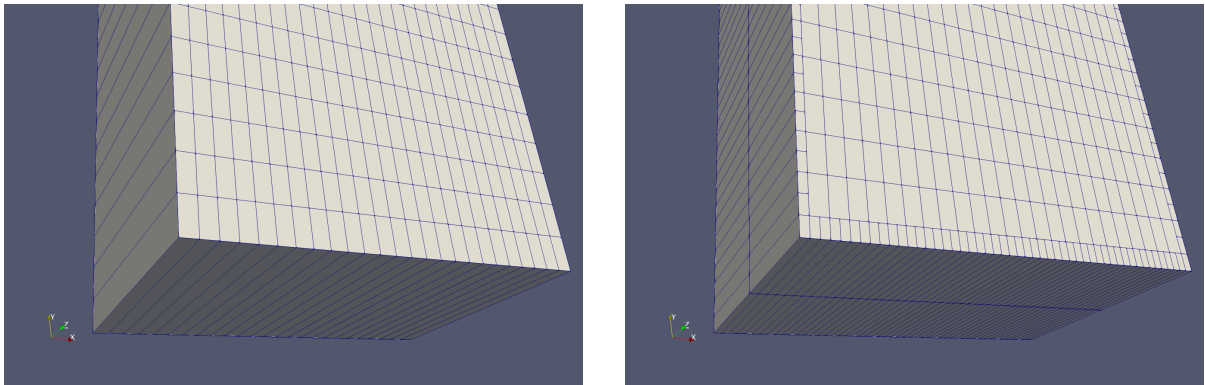
Figure 37: The mesh of the bubble column tutorial case; before and after the application of polyDualMesh .
