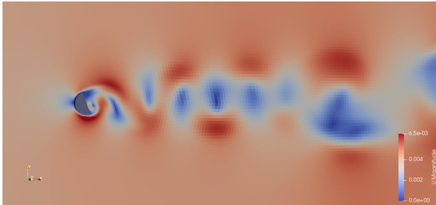
Figure 64: A 2D simulation of the semi-cylinder in laminar cross-flow using ACMI to connect the mesh of the inner region with the mesh of the outer domain.
