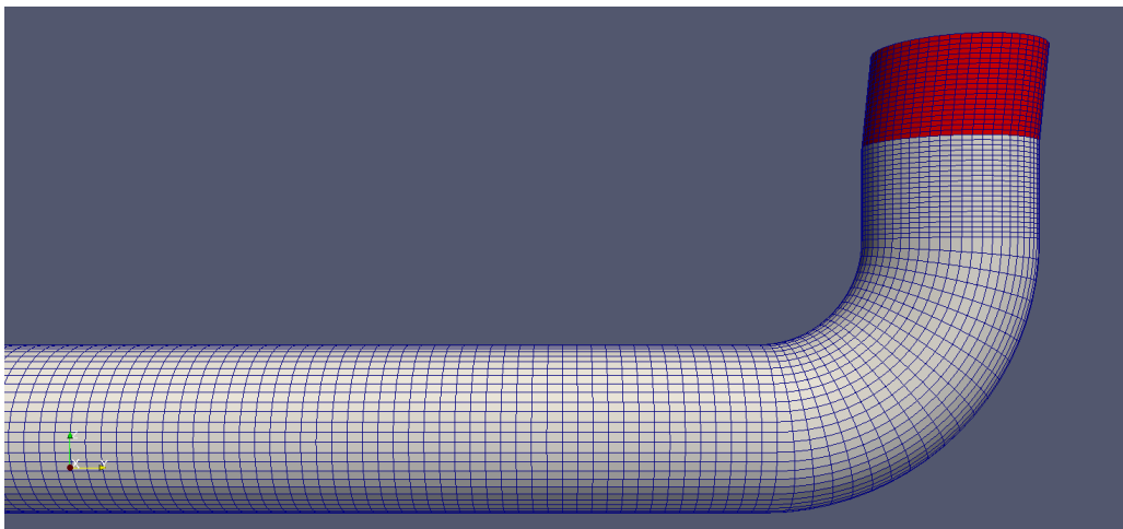
Figure 32: Subsequent mesh extrusions: sector , linearNormal and linearDirection .
