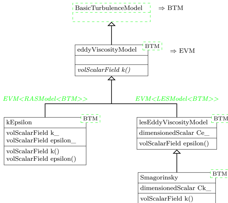
Figure 55: The class hierarchy of a selection of turbulence models of the new turbulence model framework. Note the shorthand notation BTM for the class BasicTurbulenceModel , and EVM for eddyViscosityModel .
