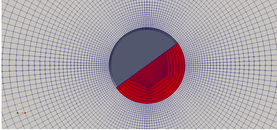
Figure 63: The inner domain in more detail. The block-structure of the inner domain is clearly recognizable. The remaining void is the body under investigation, in this case a semi-cylinder.
