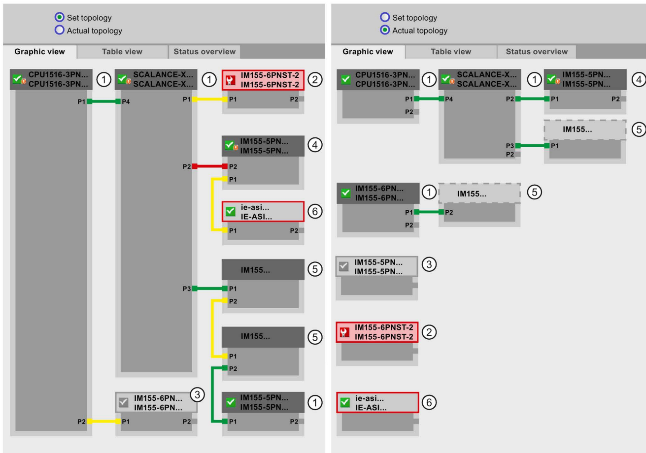
Figure 4-13 Topology - graphic view via the Web server
