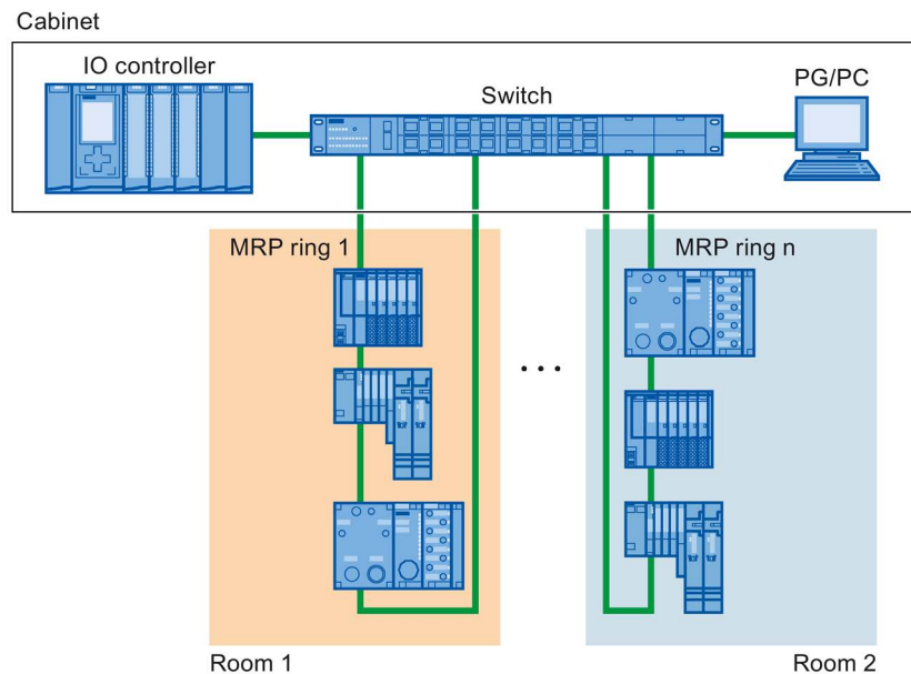
Figure 5-39 Configuration with several rings
