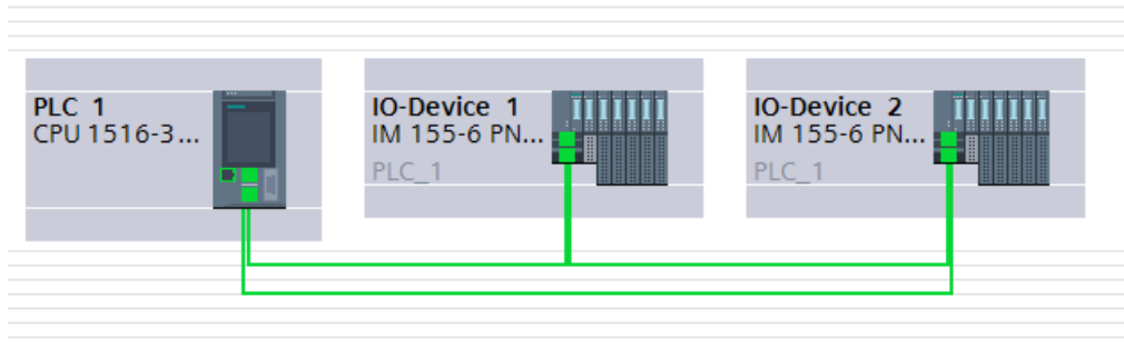
Figure 5-35 Configuring media redundancy
