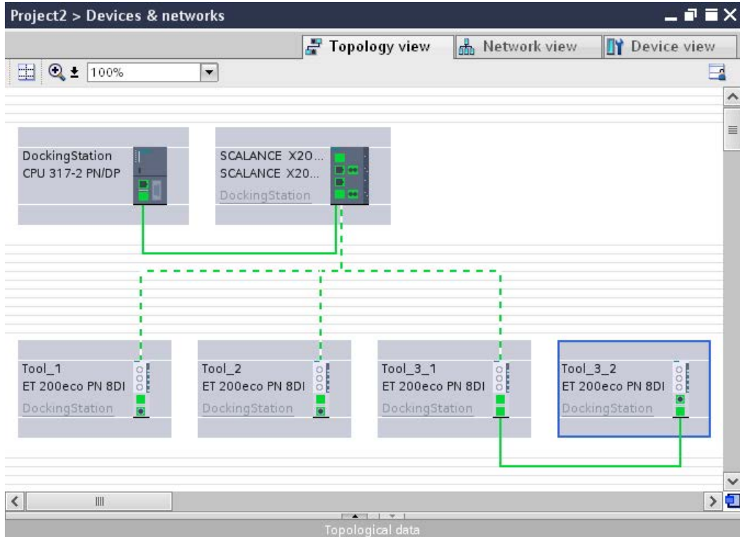
Figure 5-95 Docking system in the topology view of STEP 7
