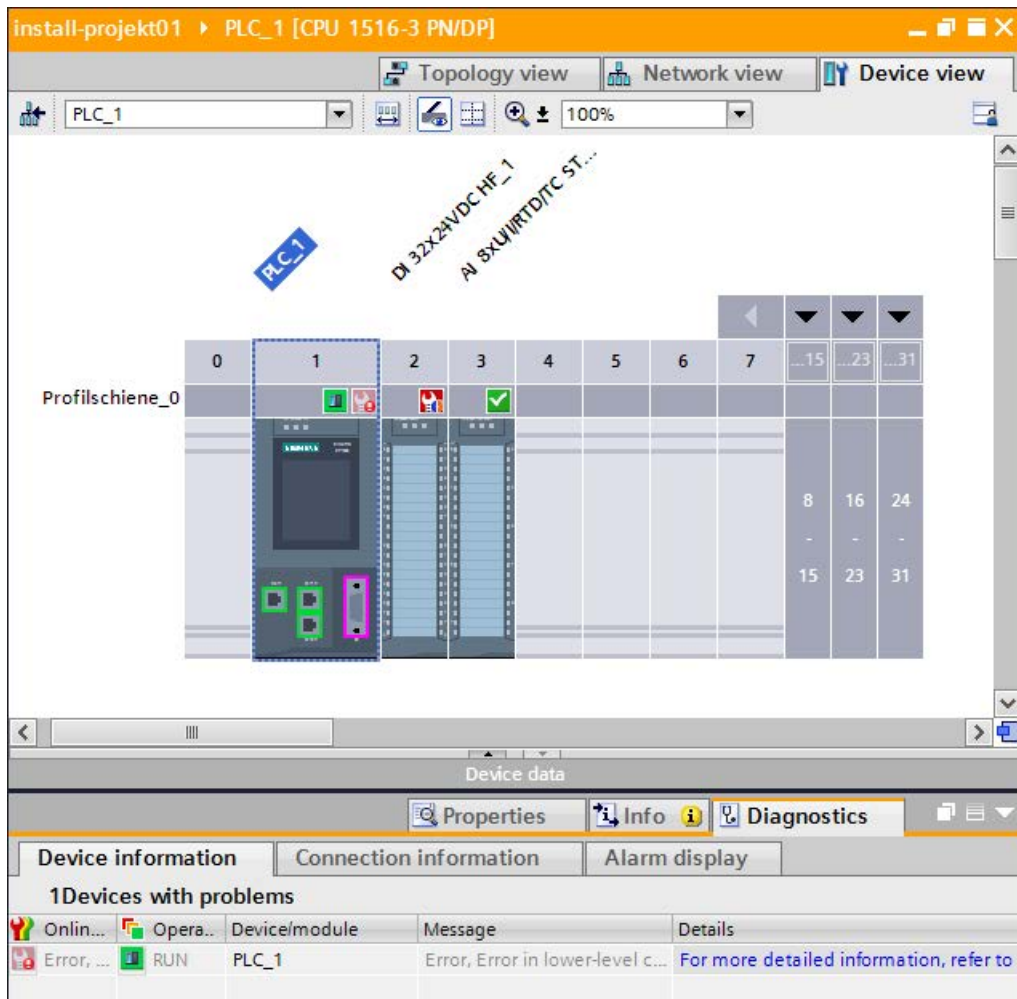
Figure 4-15 Online & diagnostics device view
