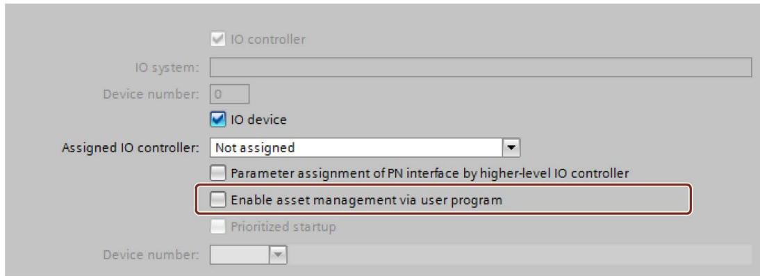
Figure 4-7 Activating asset management using a data record
