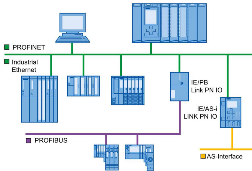
Figure 5-1 Gateways on PROFINET IO
