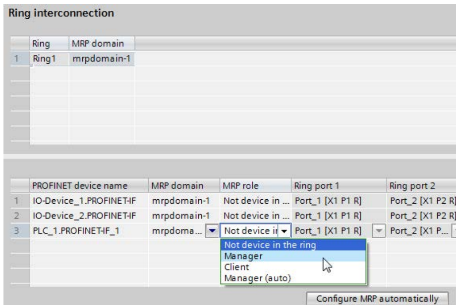
Figure 5-36 MRP domain
