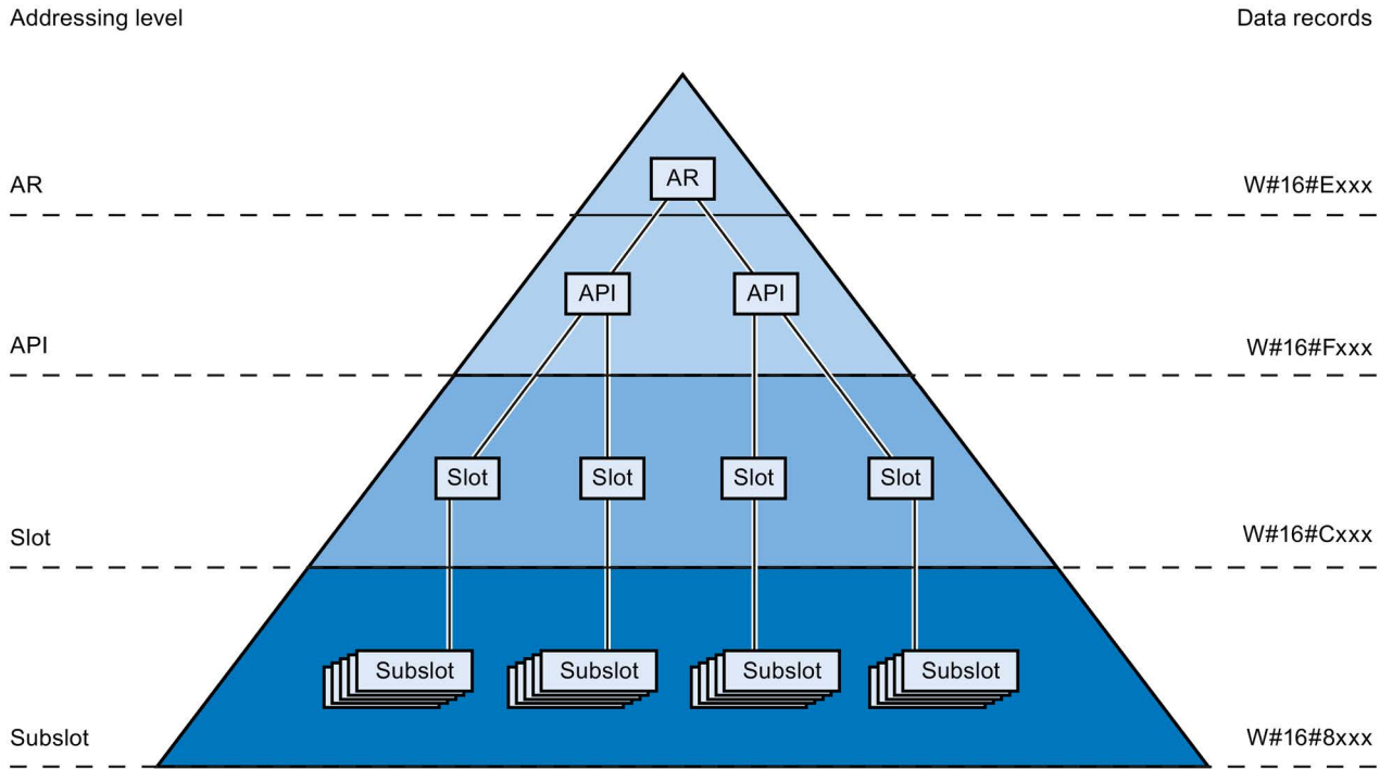
Figure 4-18 Addressing levels of diagnostics data records
