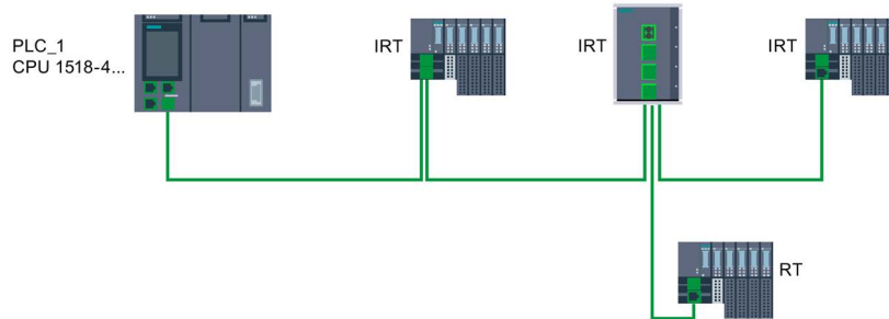
Figure 5-91 Example: Configuration control for IO systems with separated RT device
