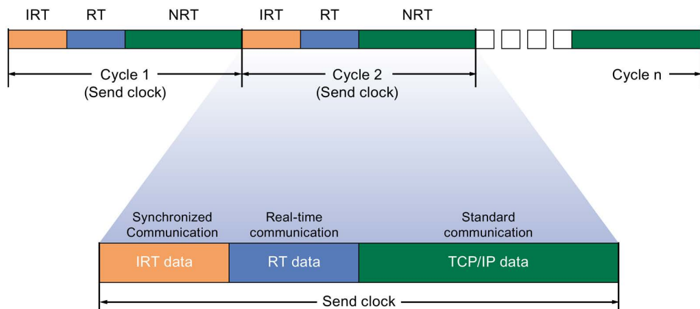
Figure 5-45 Reserving bandwidth
