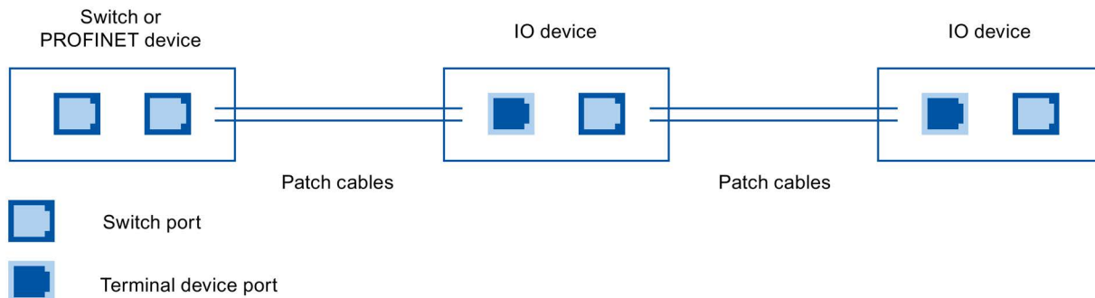
Figure 5-99 Optimized cabling for accelerated startup
