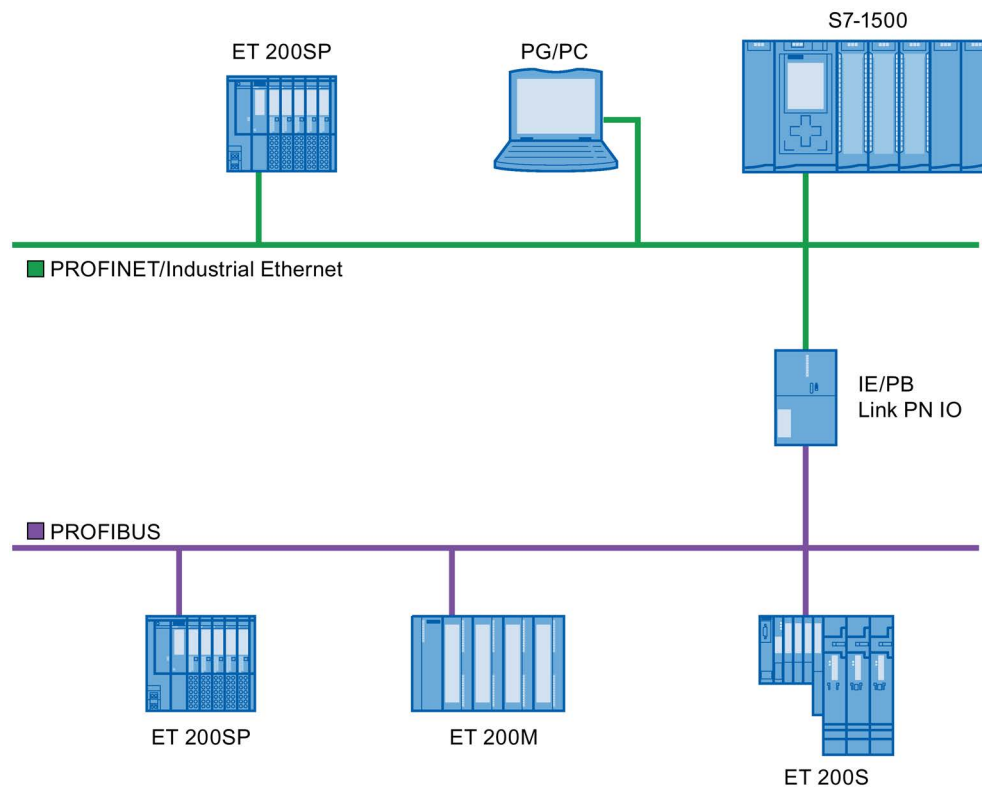
Figure 5-2 Gateway from PROFIBUS and PROFINET via IE/PB link
