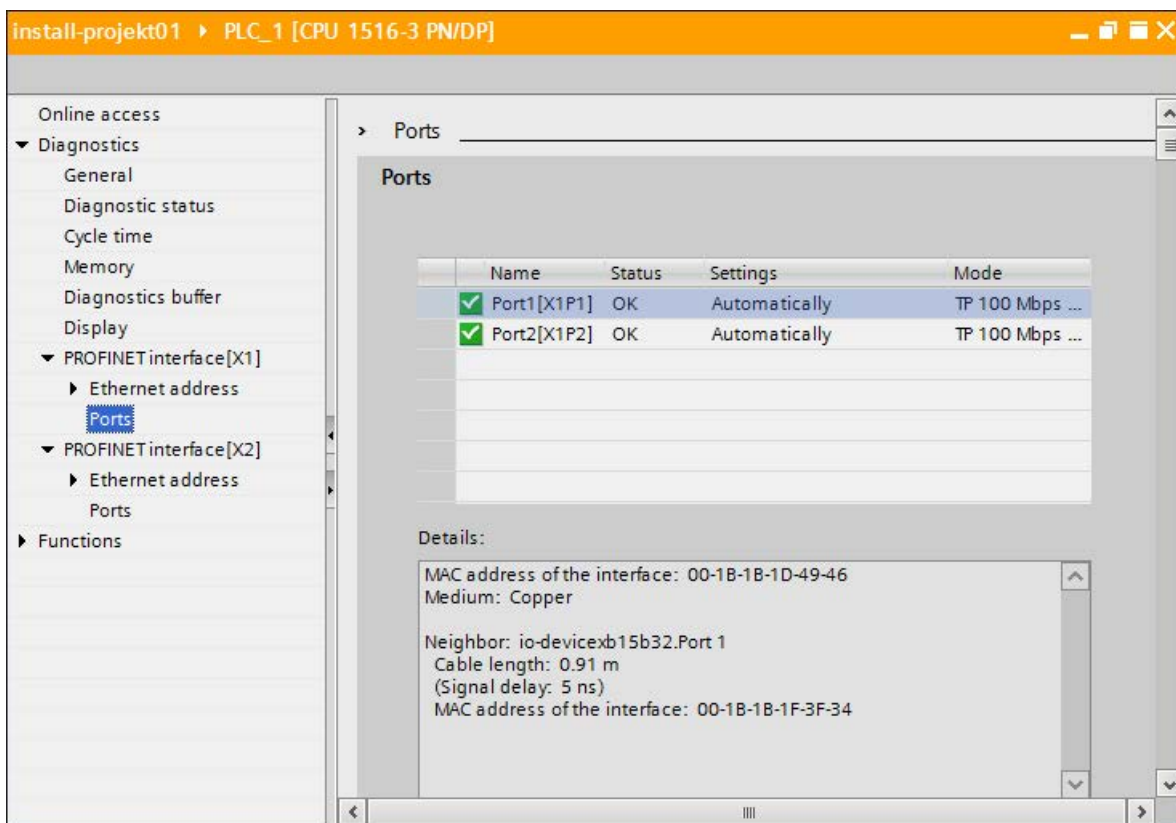
Figure 4-16 Diagnostics of PROFINET ports in STEP 7
