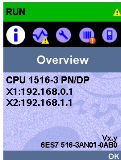
Figure 4-8 Display of overview
