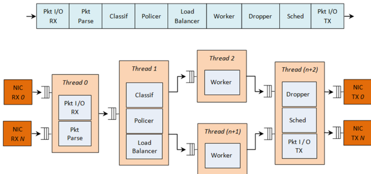
Fig. 40.1: Complex Packet Processing Pipeline with QoS Support
