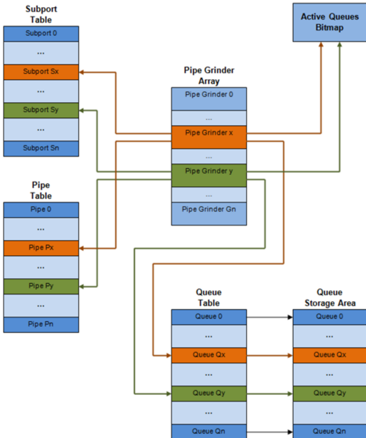
Fig. 40.4: Internal Data Structures per Port
