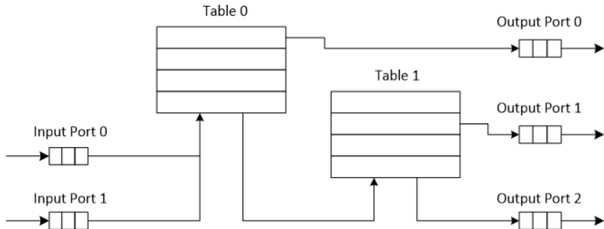
Fig. 43.1: Example of Packet Processing Pipeline where Input Ports 0 and 1 are Connected with Output Ports 0, 1 and 2 through Tables 0 and 1
