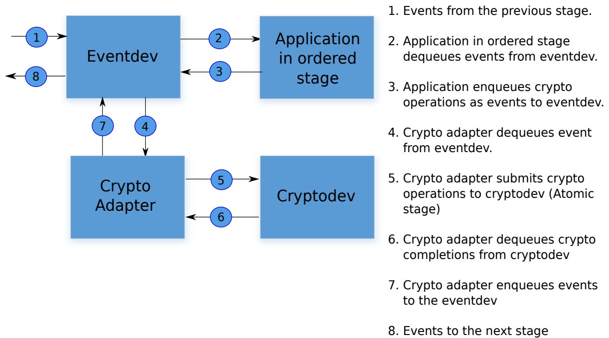
Fig. 39.2: Working model of RTE_EVENT_CRYPTOP_ADAPTER_OP_FORWARD mode
