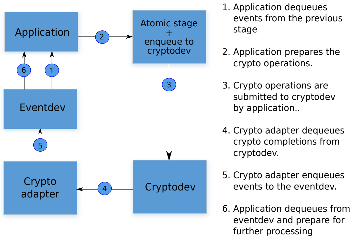
Fig. 39.1: Working model of RTE_EVENT_CRYPTODAPTER_OP_NEW mode
