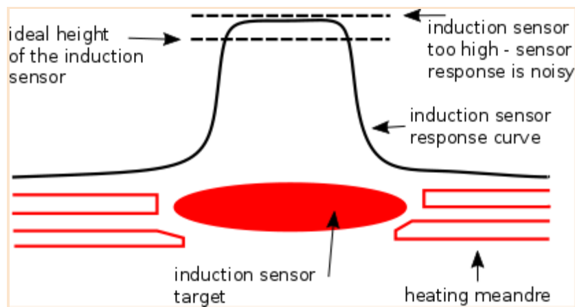
Pict. 11 - Probe response diagram.
