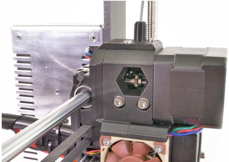
Pict. 37 - Cleaning the extruder - you can see the hobbed pulley through the service hole
