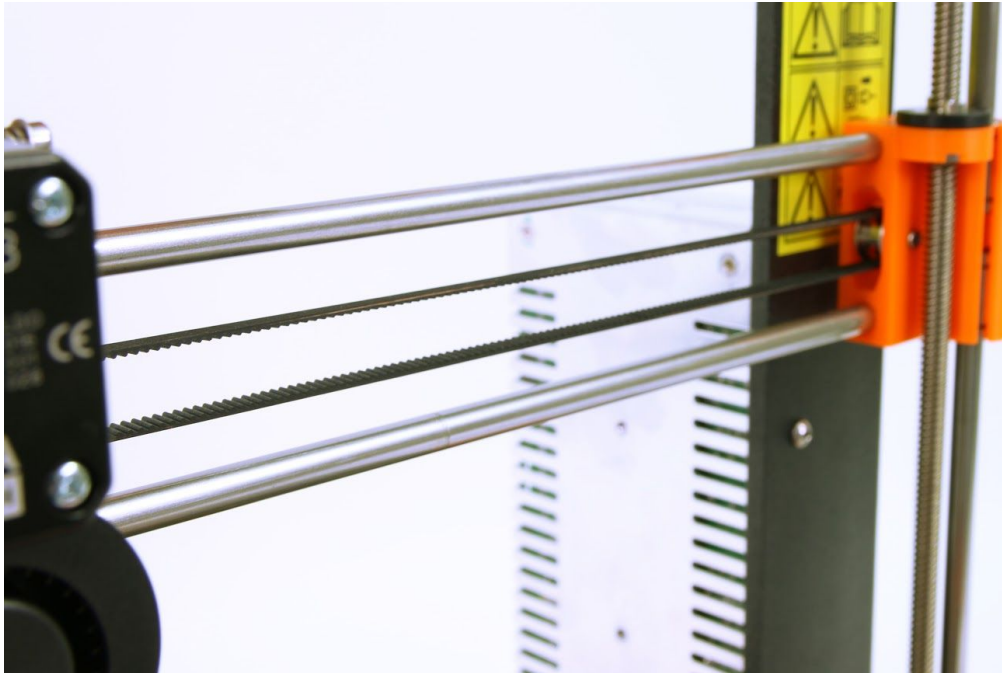
Pict. 42 - A properly tightened X-axis belt
