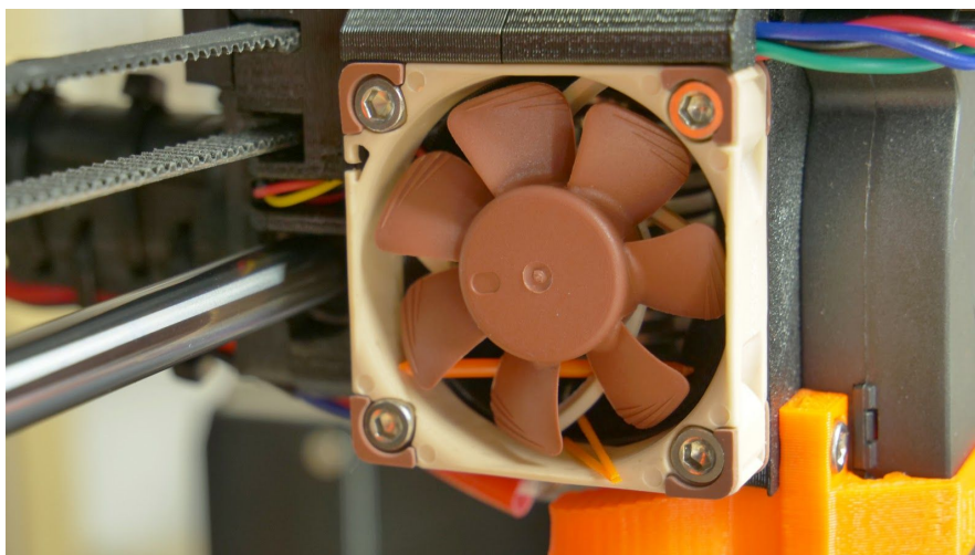
Pict. 33 - Nozzle cooling fan from Noctua
