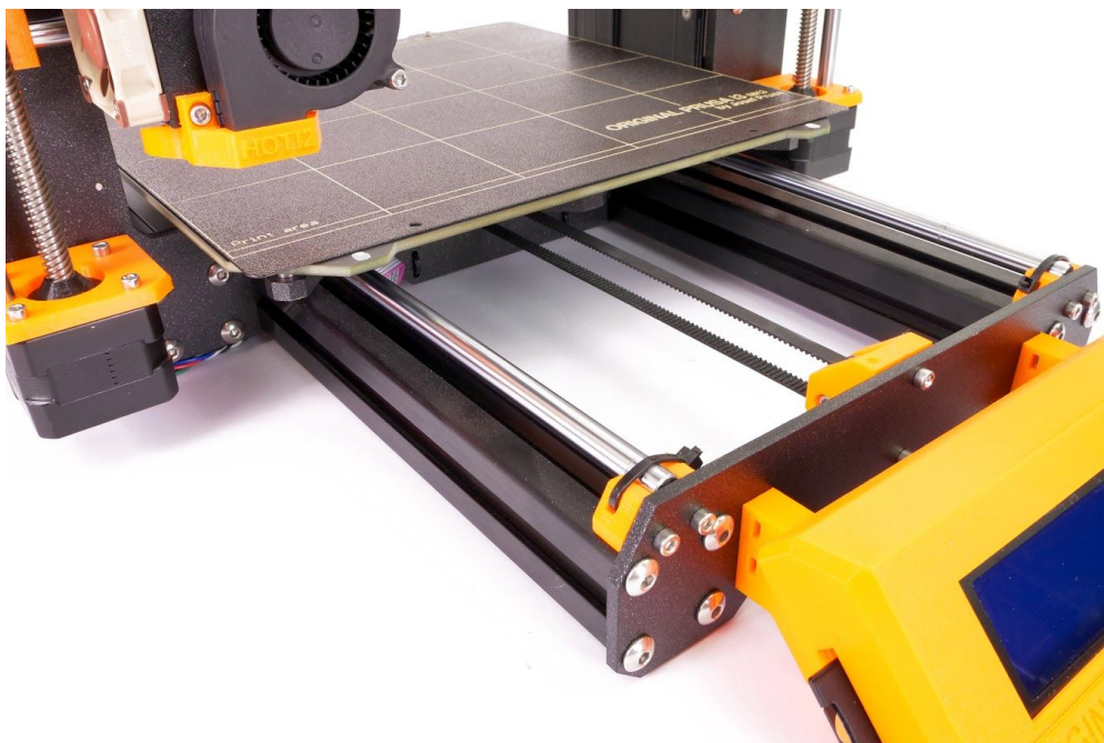
Pict. 41 - A properly tightened Y-axis belt under the heatbed
