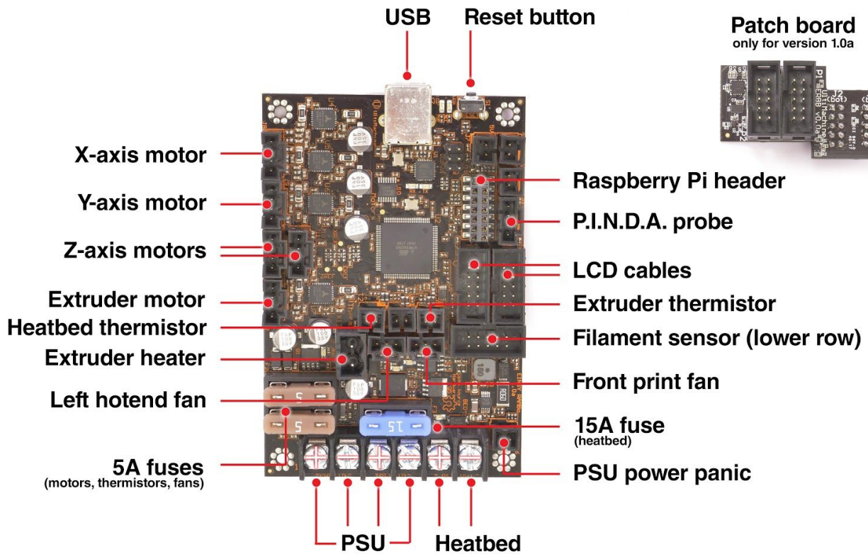
Pict. 40 - Proper wiring of the connectors
