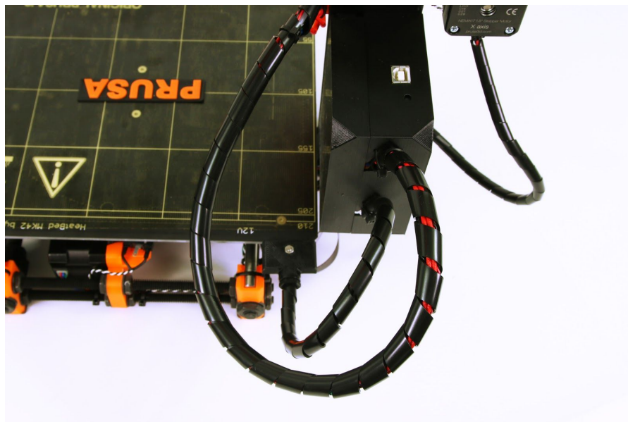
Pict. 43 - Cables to be wrapped in a spiral wrap
