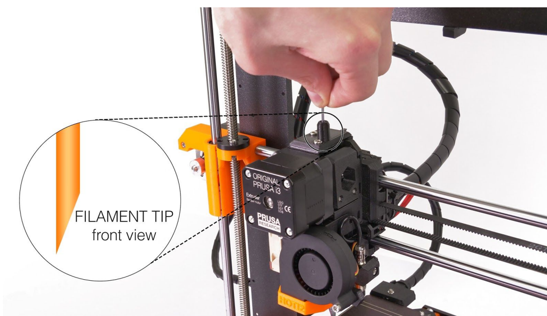
Pict. 8 - Loading the filament to the extruder
