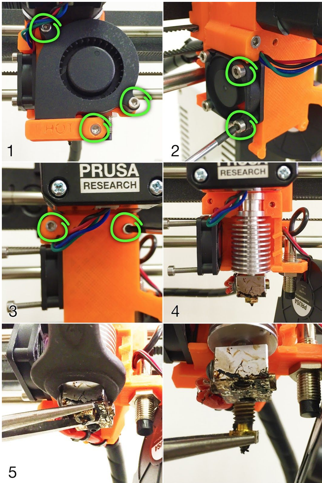
Pict. 38 - Nozzle change
