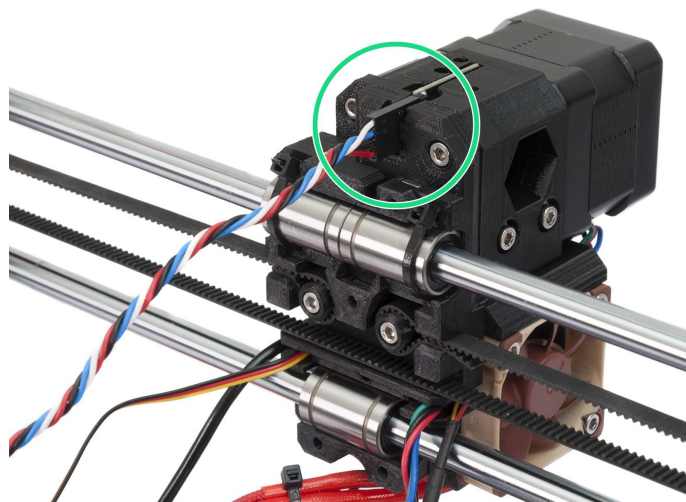
Pict. 35 - Properly connected filament sensor
