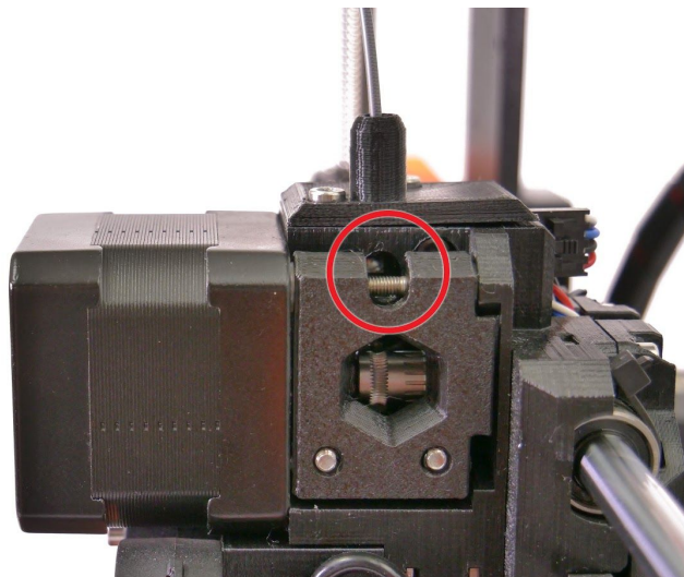
Pict. 36 - Access hole for cleaning the filament sensor
