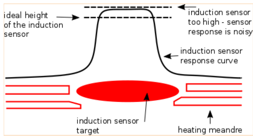
Pict. 12 - Probe response diagram.
