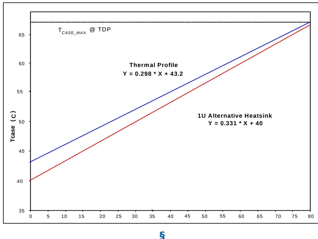
Figure A-3. 1U Alternative Heatsink Thermal Adherence to Quad-Core Intel® Xeon® Processor L5400 Series Thermal Profile
