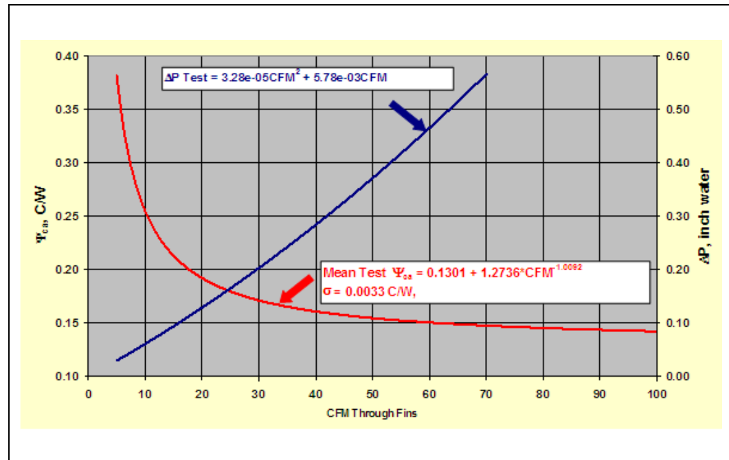
Figure 2-17. 2U+ CEK Heatsink Thermal Performance
