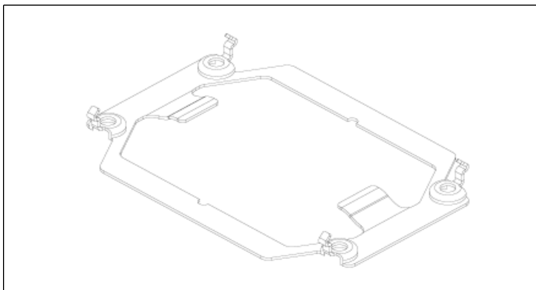
Figure 2-25. Isometric View of CEK Spring Attachment to the Base Board
