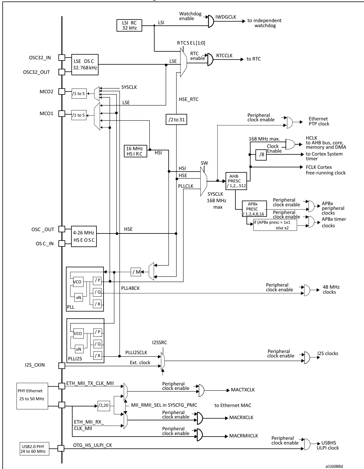
Figure 21. Clock tree
