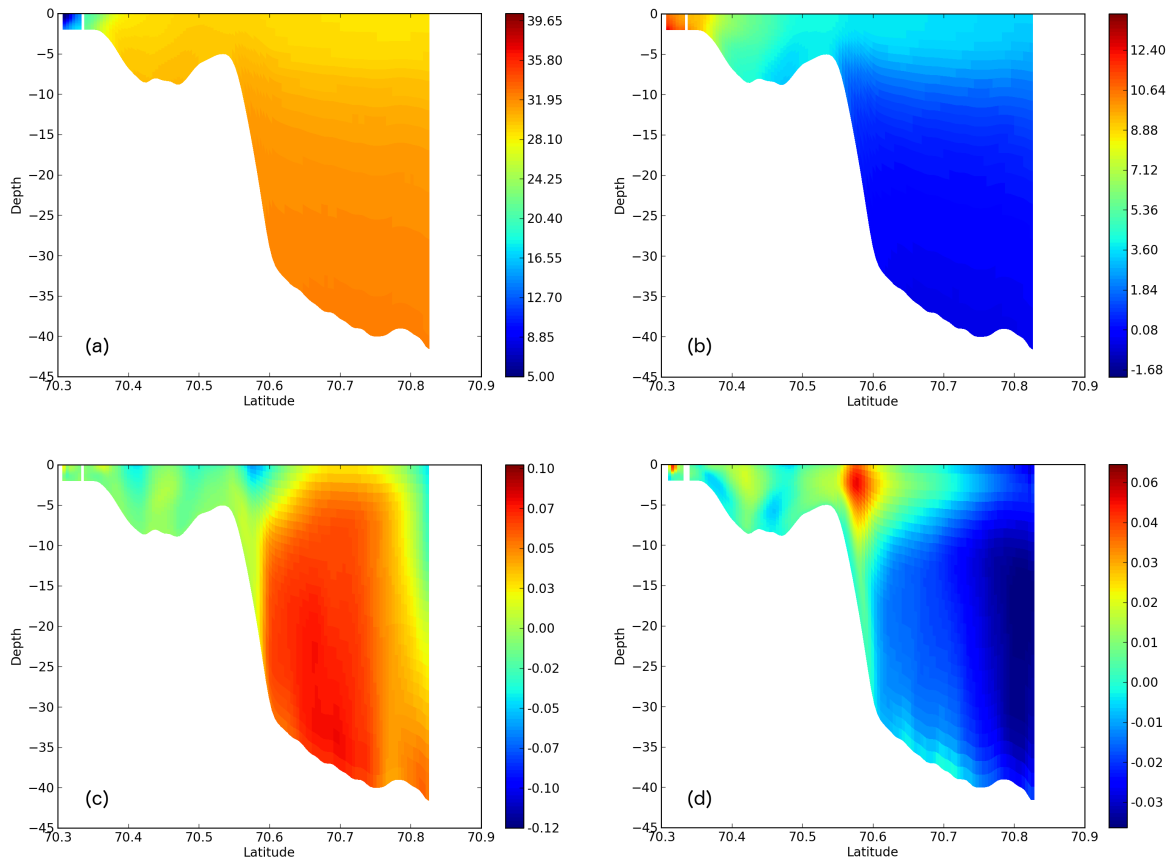
Figure 33: Vertical slices for the August climatology in the Beaufort3 domain, (a) salinity, (b) temperature ( ^{\circ}\text{C} ), (c) longshore velocity ( m/s ) and (d) cross-shore velocity ( m/s ). Note the warm, fresh water right up on the shelf, trapped by a barrier island.
