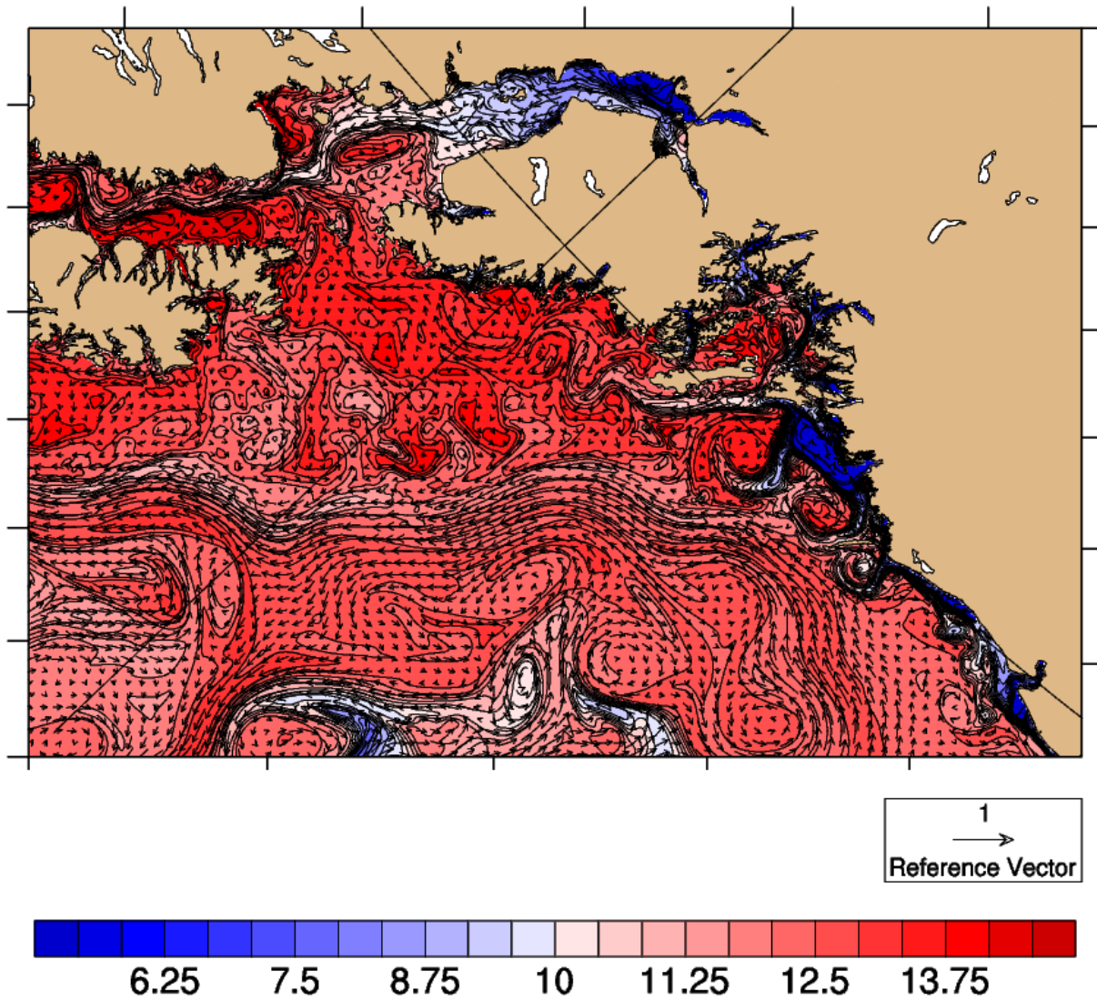
Figure 28: Surface temperature and velocities for 10 August, 2008. Graticules shown are 60°N and 150°W.
