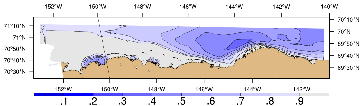
Figure 32: Sea-ice concentration for the June climatology in the Beaufort3 domain. Note the location of a few warm rivers between 148° and 151° W longitude.
