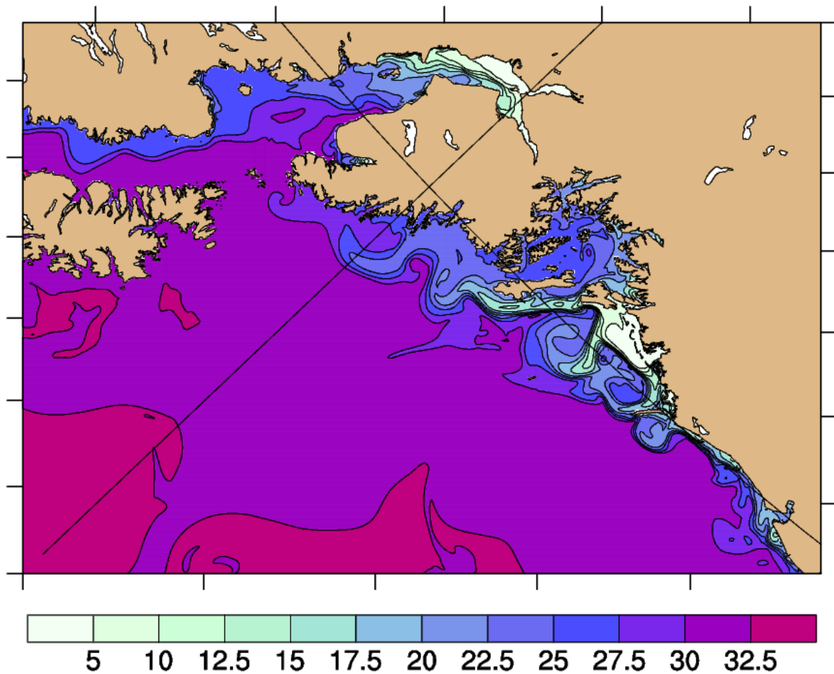
Figure 27: Surface salinity for 10 August, 2008. Graticules shown are 60°N and 150°W.
