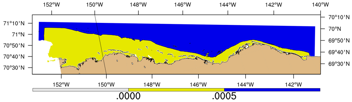
Figure 31: Ice speed contour at 0.0005 m/s for the April climatology in the Beaufort3 domain. This contour was chosen as an estimate of the land-fast ice extent.
