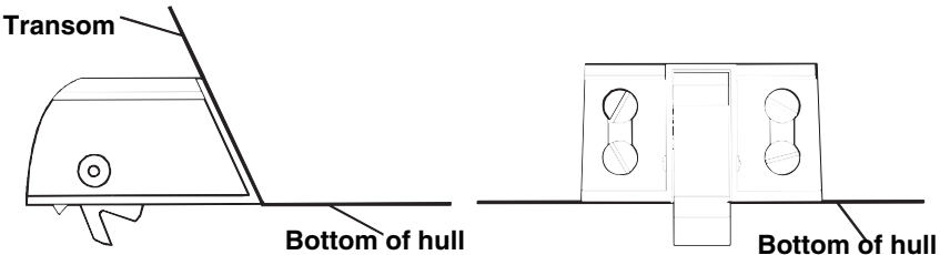
Speed sensor mounting configuration: side view (left) and rear view (right.)
