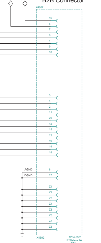
20 pin VT Camera Flex B2B Connector
