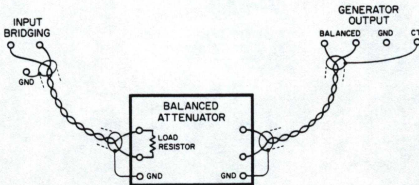
Figure 3-3. Balanced Load Test Setup.
