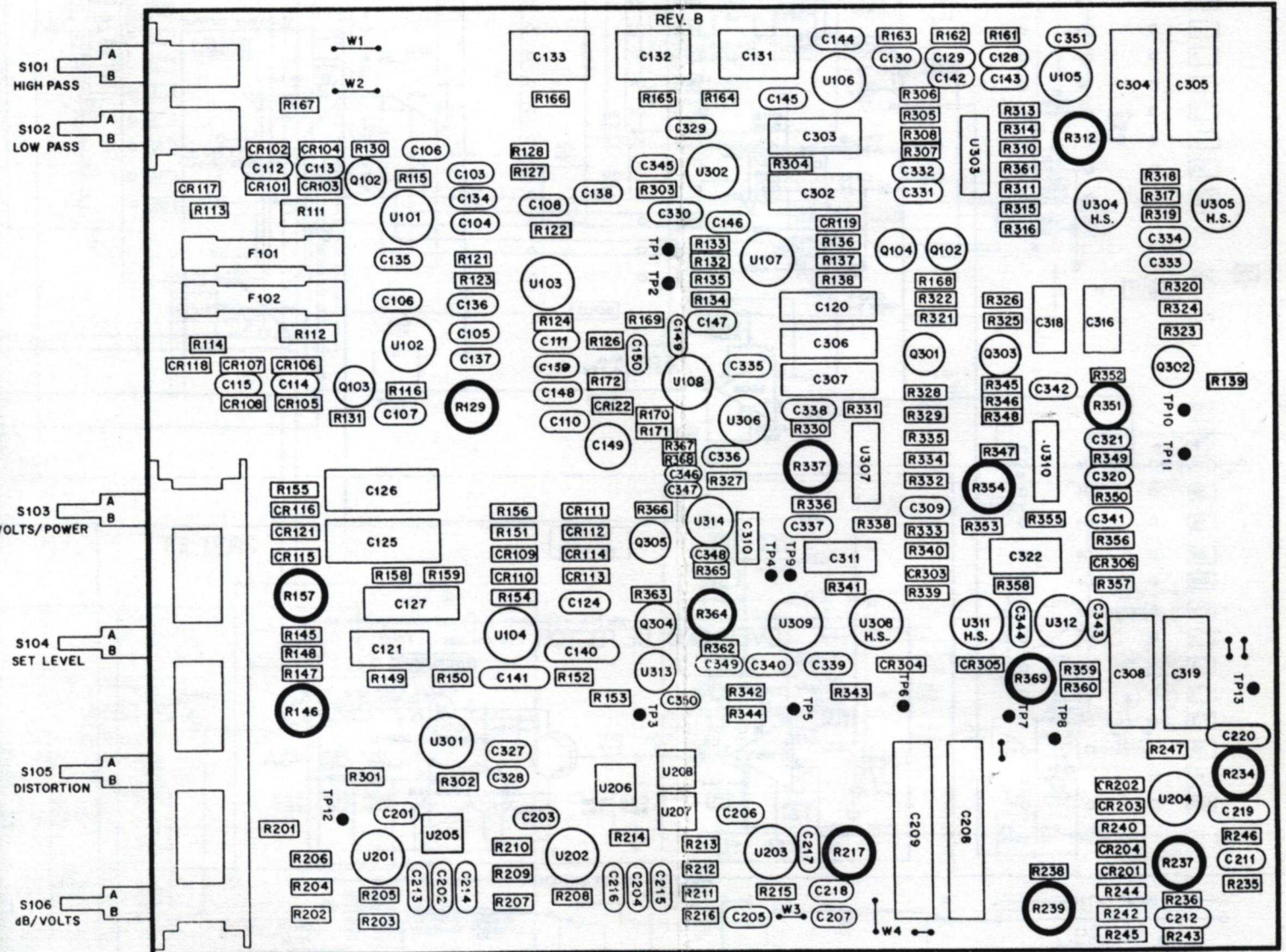
FIGURE 4-1 COMPONENT LOCATOR ANALYZER BOARD
