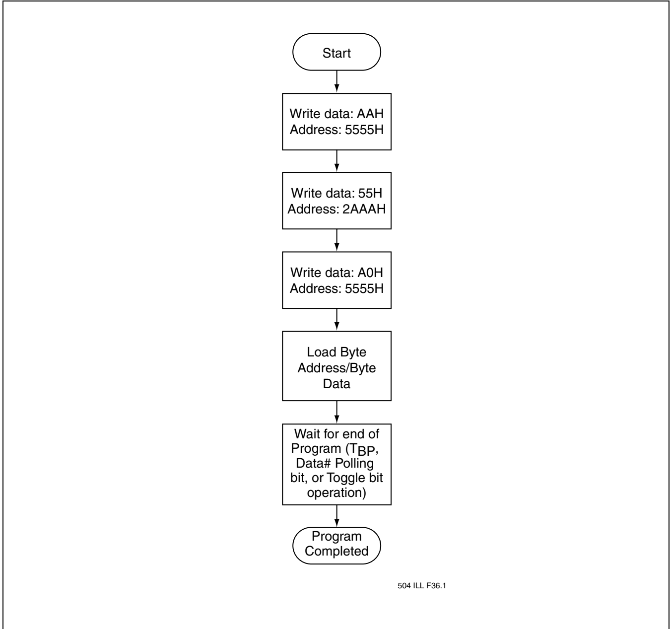
FIGURE 26: BYTE-PROGRAM ALGORITHM
