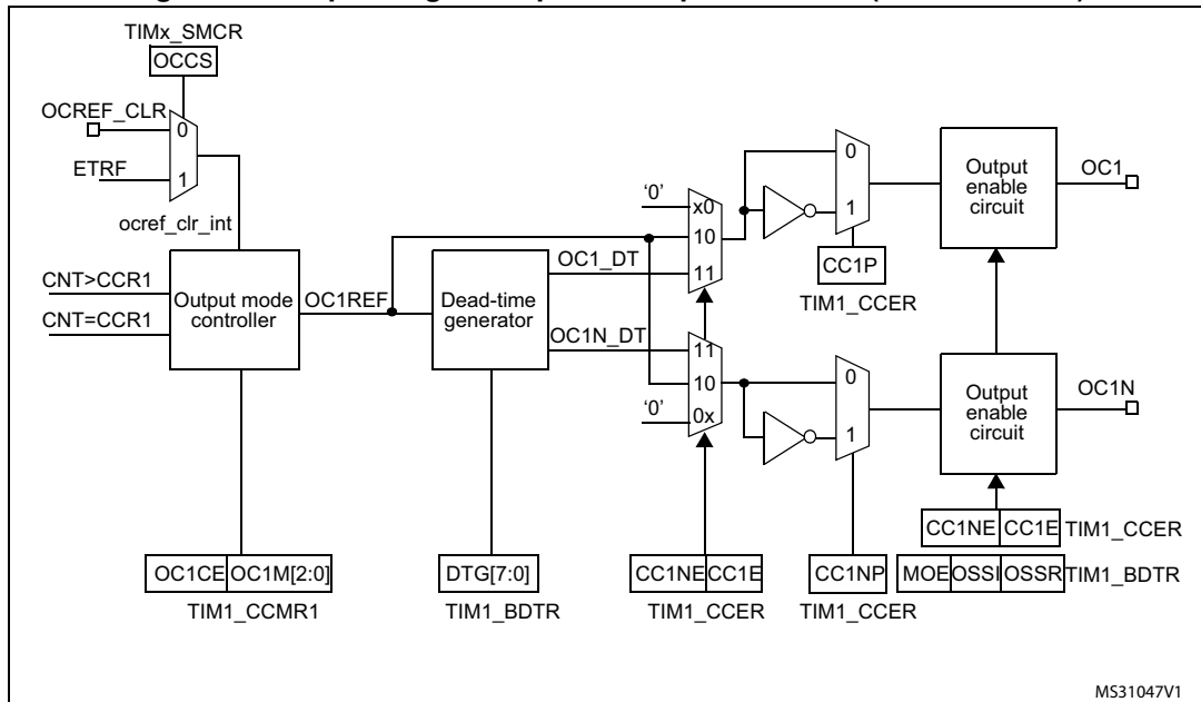
Figure 87. Output stage of capture/compare channel (channel 1 to 3)
