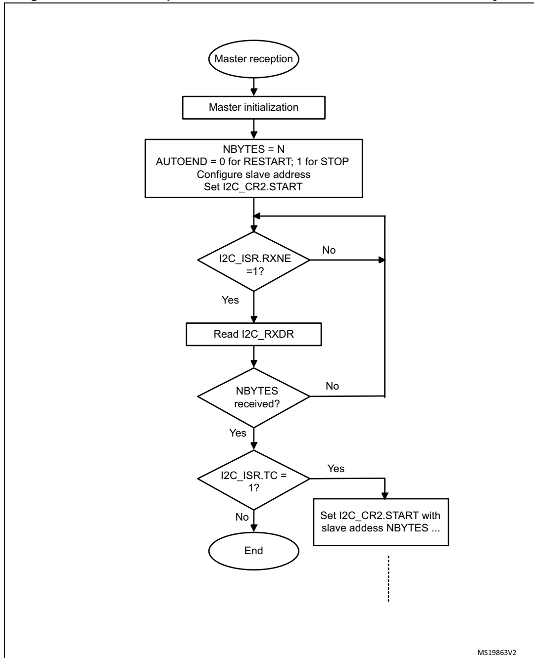
Figure 234. Transfer sequence flowchart for I2C master receiver for N \leq 255 bytes
