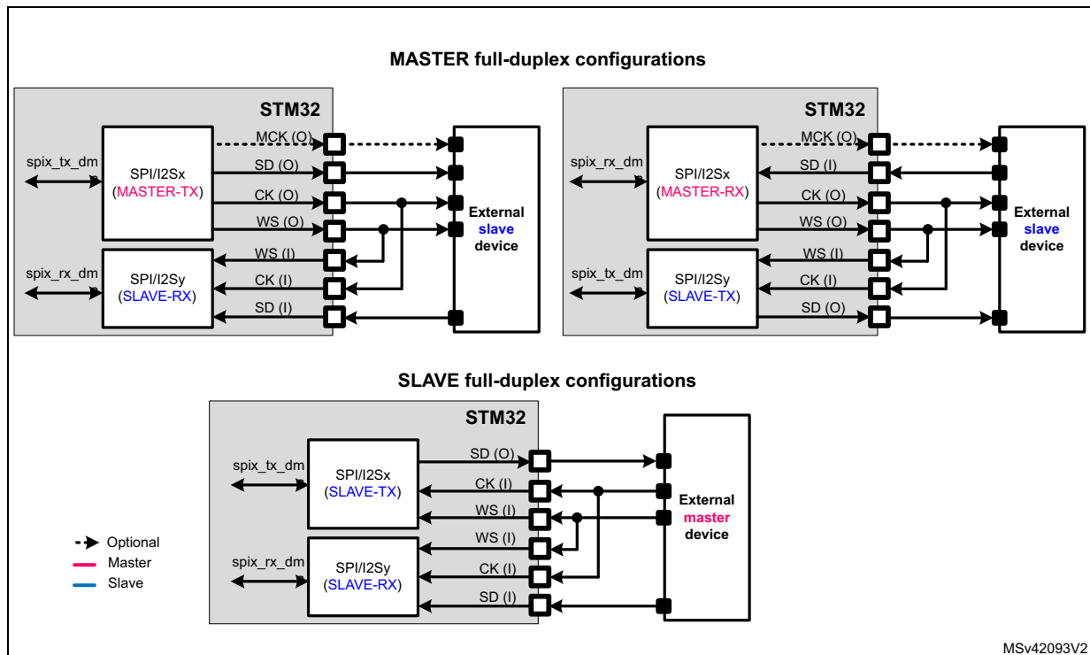
Figure 287. Full-duplex communication
