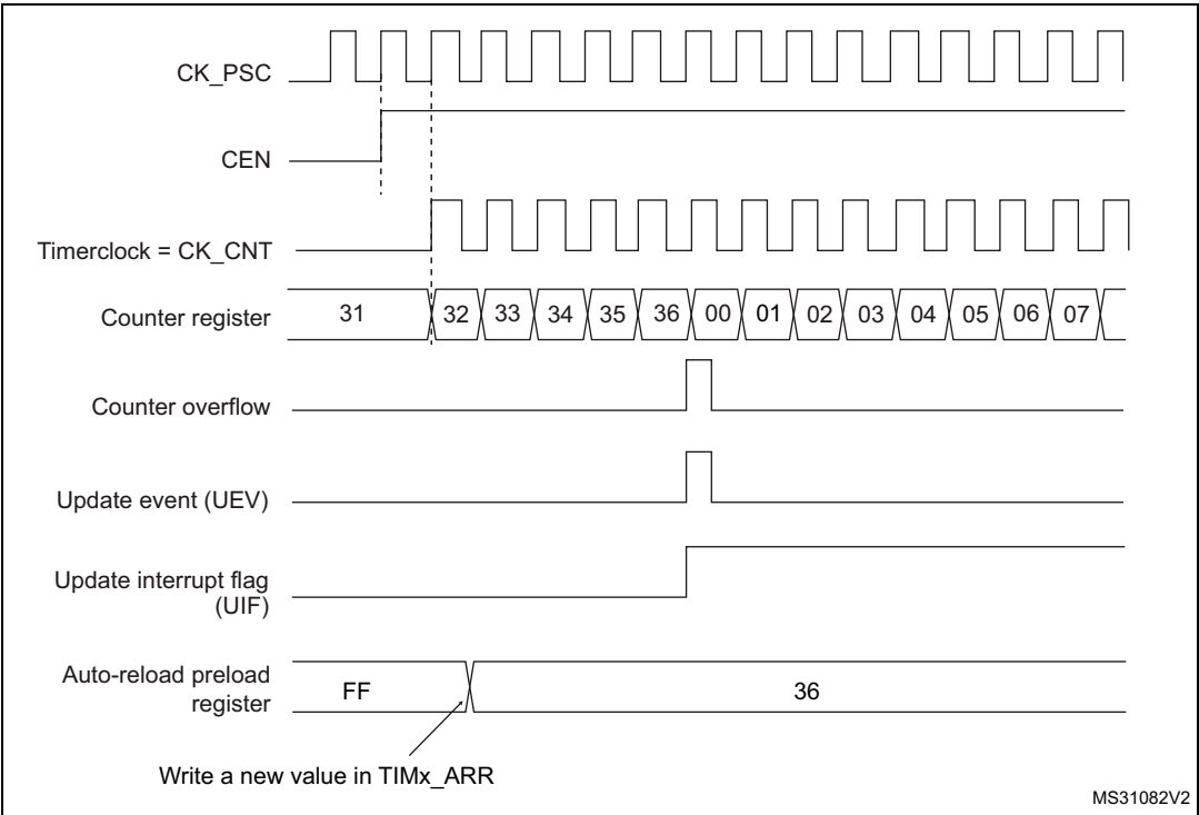
Figure 66. Counter timing diagram, update event when ARPE=0 (TIMx_ARR not preloaded)
