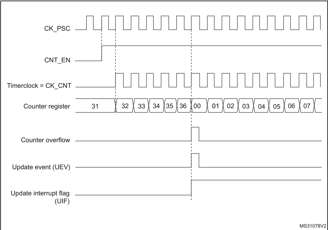
Figure 62. Counter timing diagram, internal clock divided by 1
