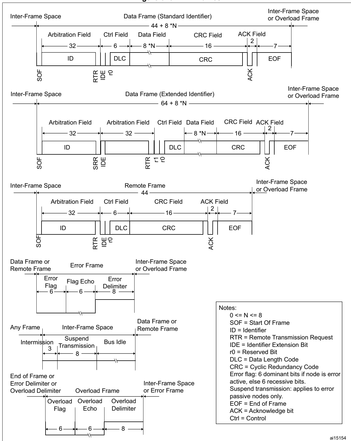
Figure 320. CAN frames
