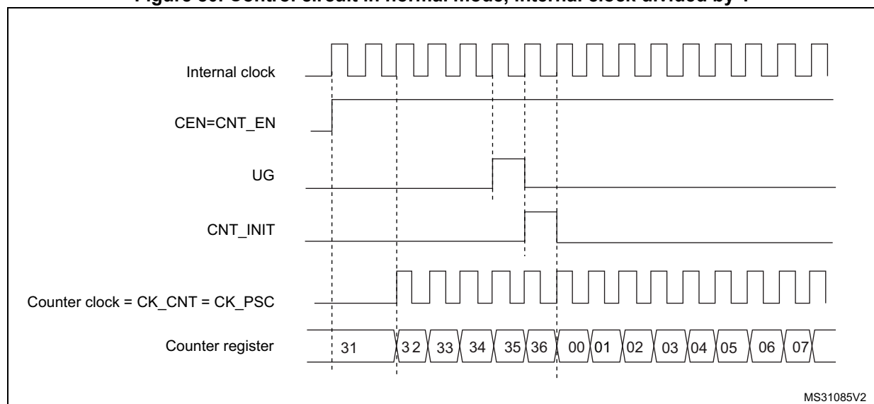
Figure 80. Control circuit in normal mode, internal clock divided by 1
