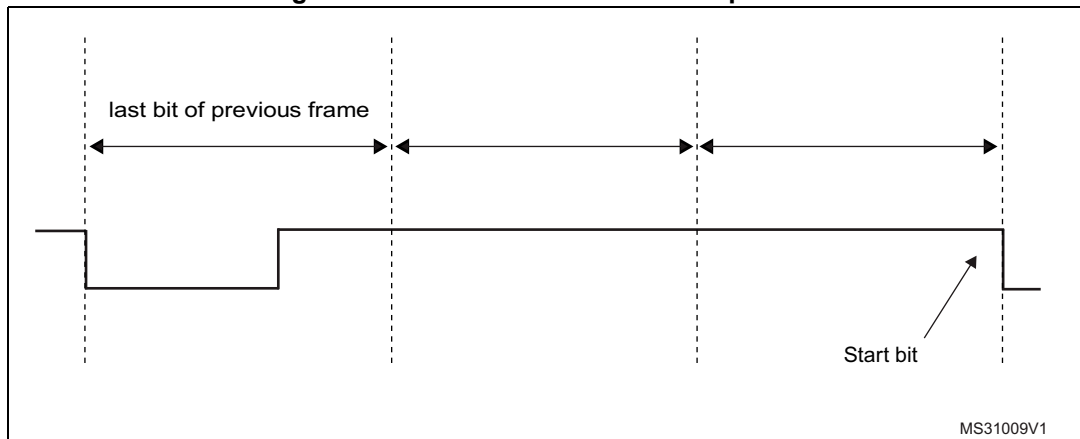
Figure 331. SFT of three nominal bit periods
