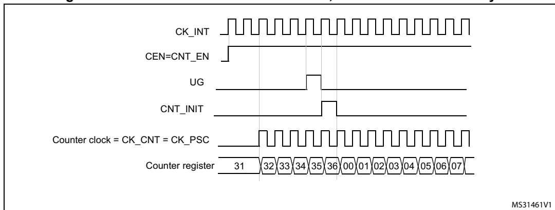
Figure 162. Control circuit in normal mode, internal clock divided by 1
