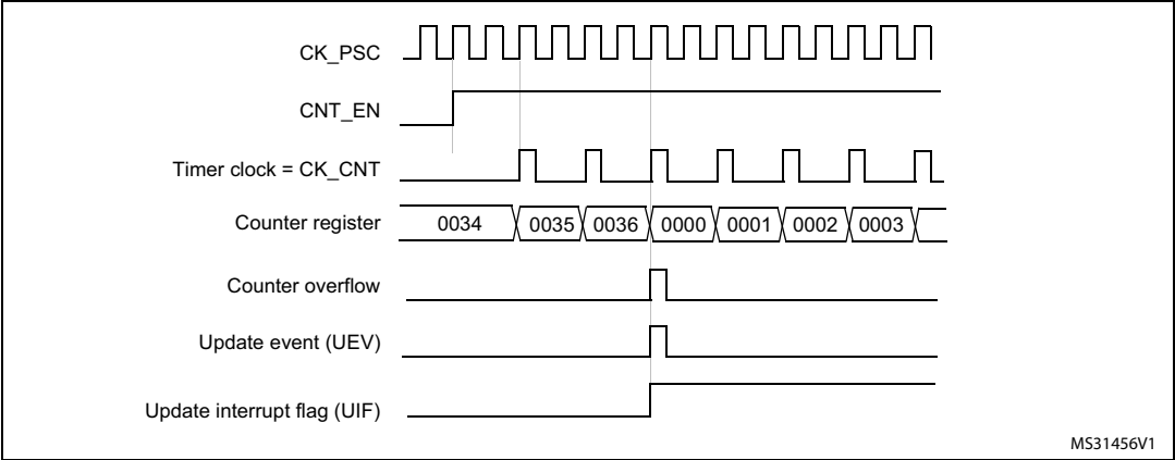
Figure 157. Counter timing diagram, internal clock divided by 2
