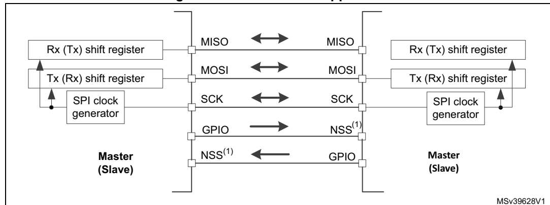
Figure 275. Multi-master application
