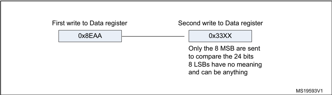
Figure 290. Transmitting 0x8EAA33
