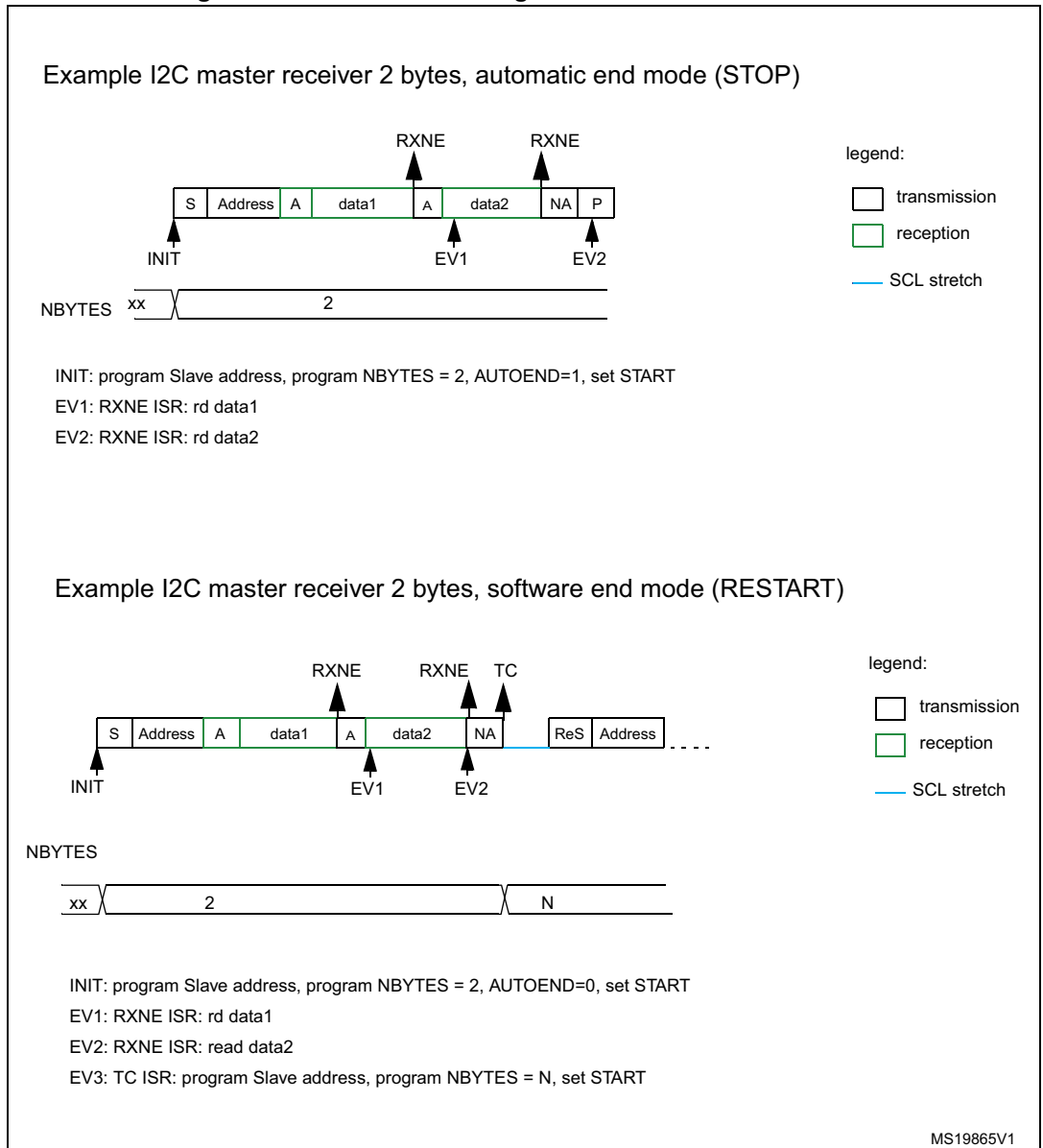
Figure 236. Transfer bus diagrams for I2C master receiver
