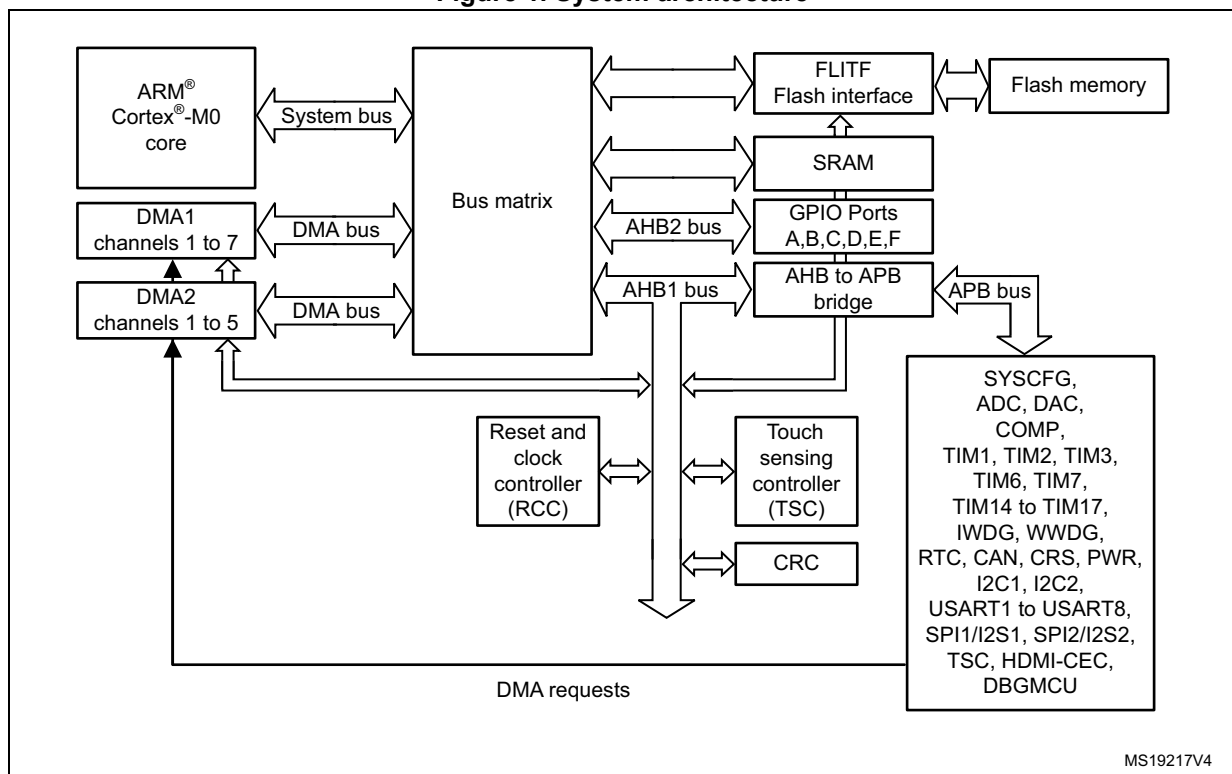
Figure 1. System architecture
