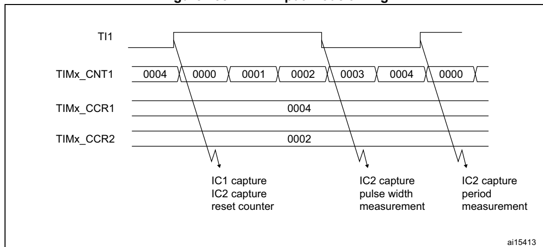
Figure 135. PWM input mode timing
