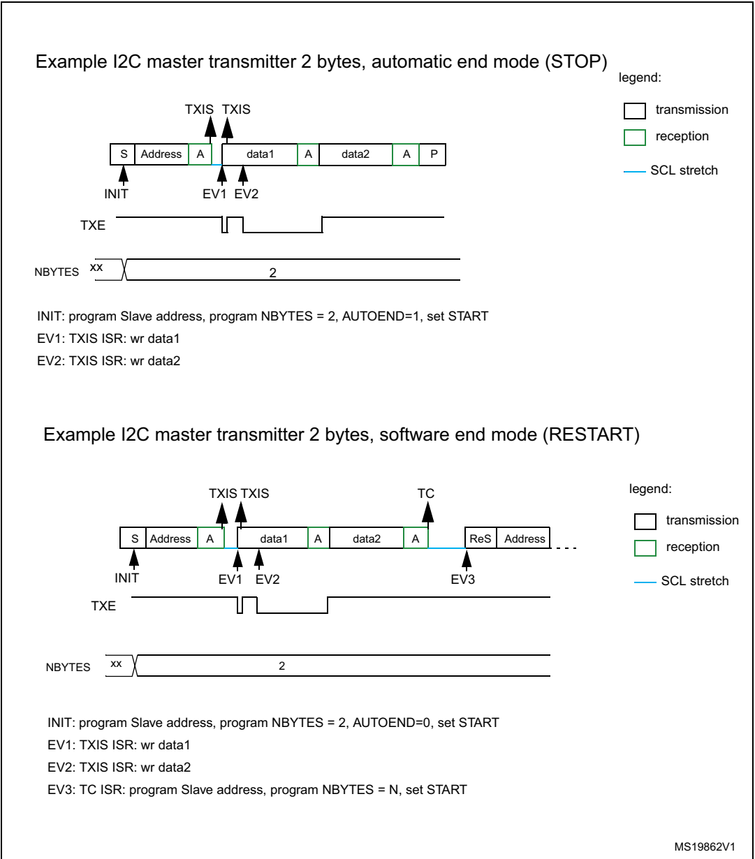
Figure 233. Transfer bus diagrams for I2C master transmitter
