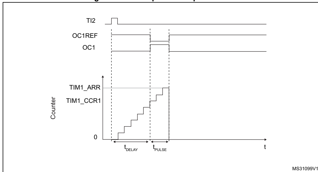
Figure 193. Example of One-pulse mode
