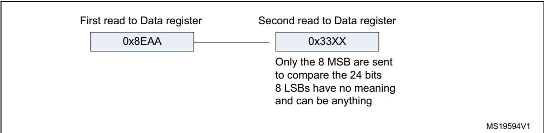
Figure 291. Receiving 0x8EAA33
