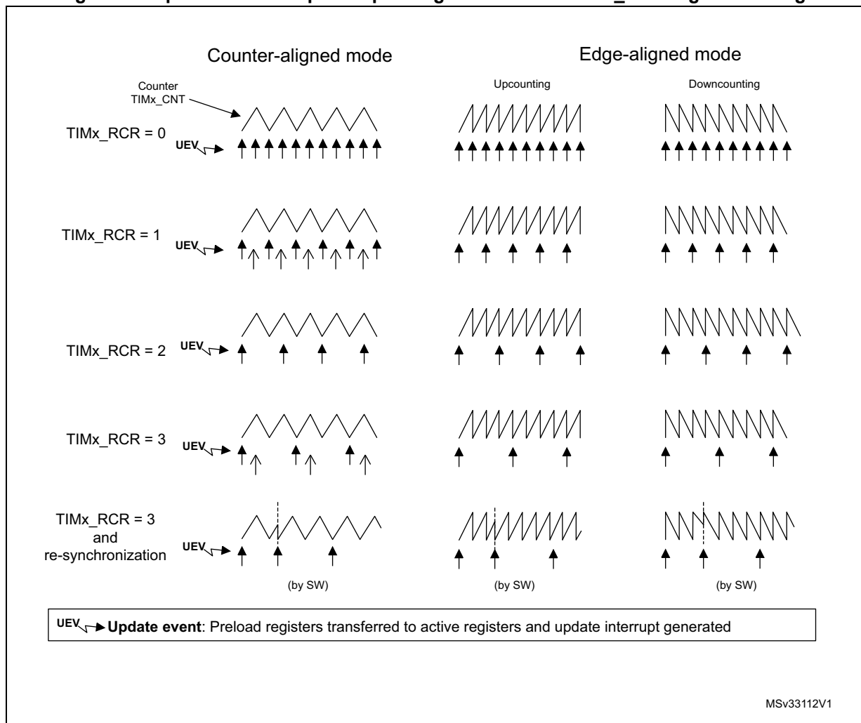
Figure 79. Update rate examples depending on mode and TIMx_RCR register settings
