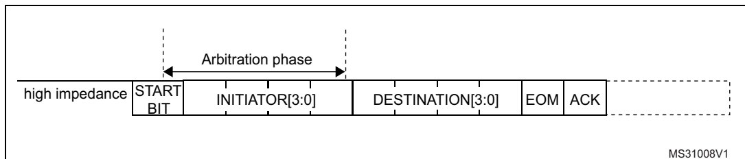
Figure 330. Arbitration phase
