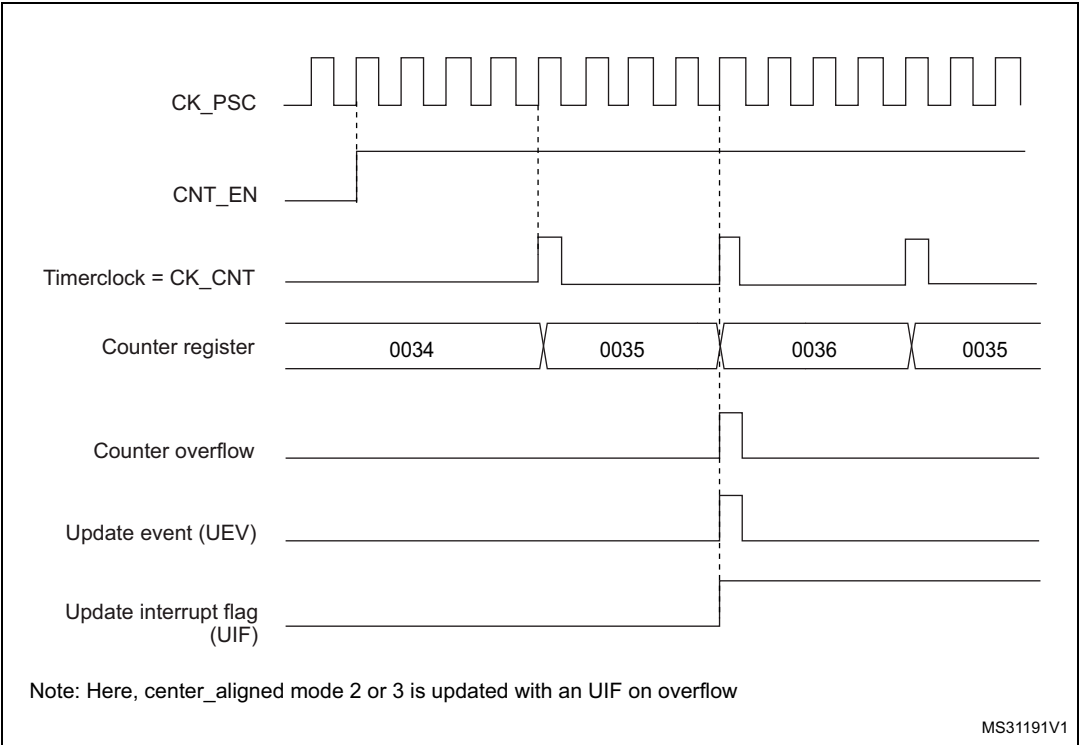
Figure 75. Counter timing diagram, internal clock divided by 4, TIMx_ARR=0x36
