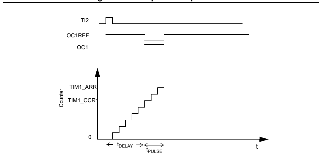
Figure 99. Example of one pulse mode
