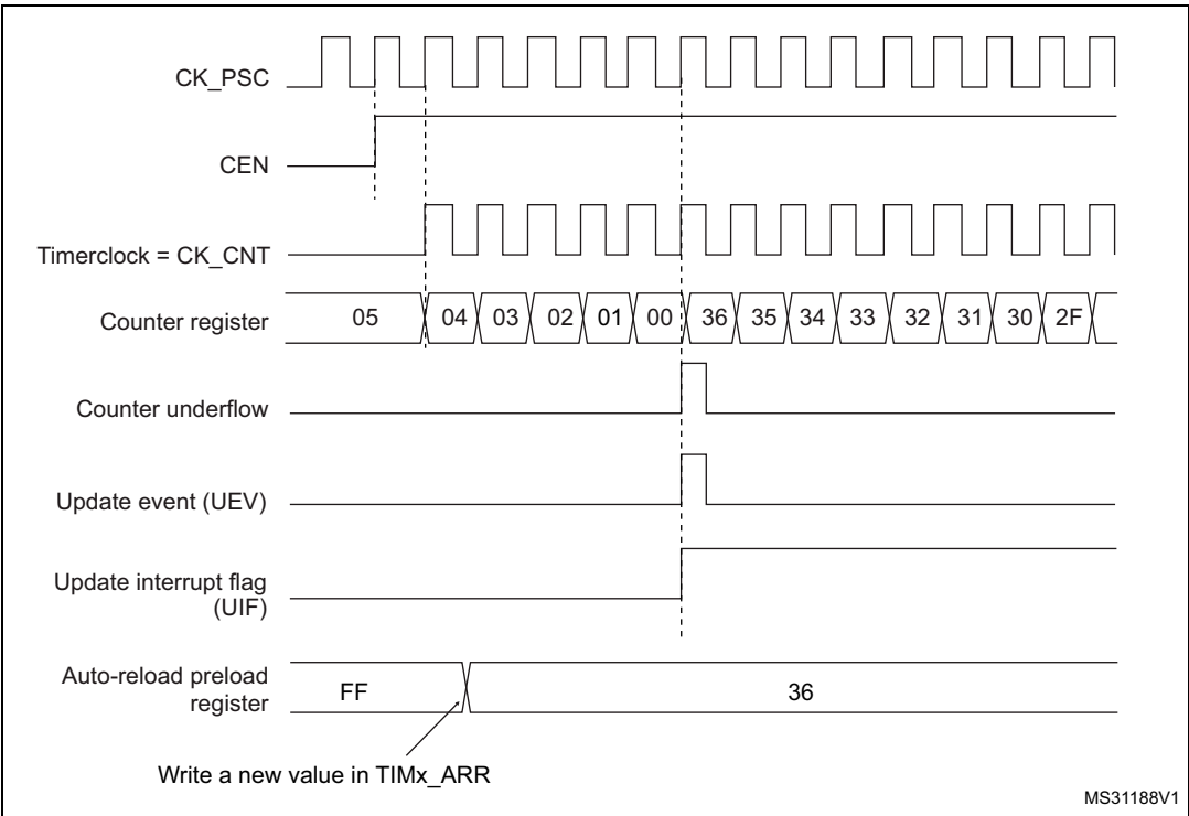
Figure 120. Counter timing diagram, Update event when repetition counter is not used
