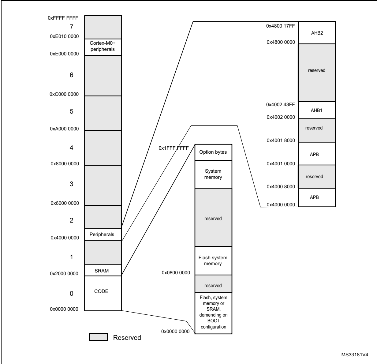
Figure 2. Memory map
