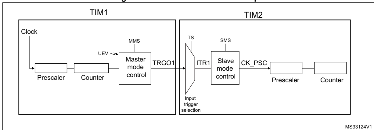
Figure 147. Master/Slave timer example
