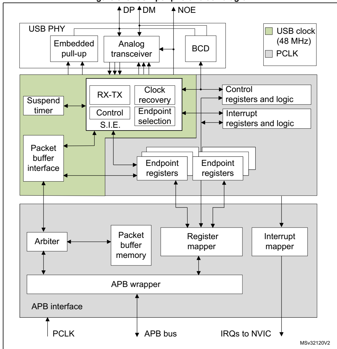
Figure 323. USB peripheral block diagram
