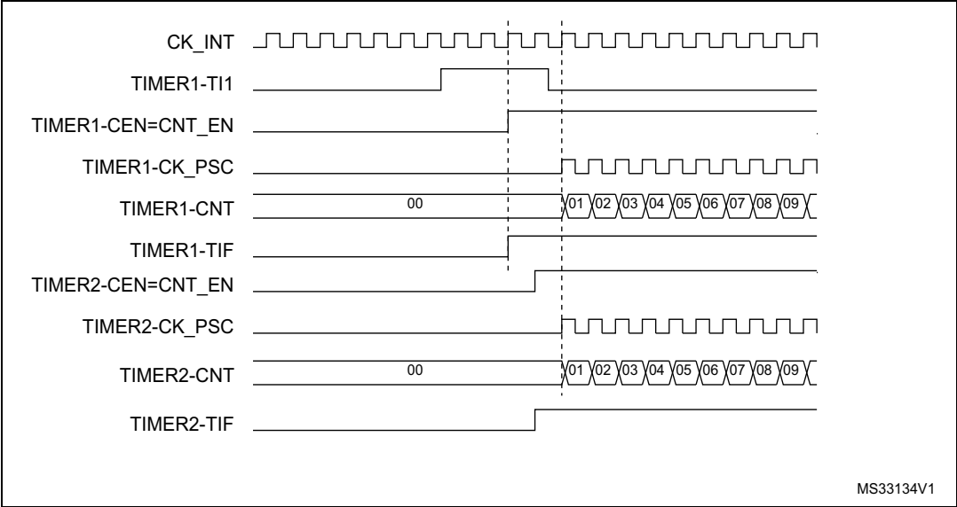
Figure 152. Triggering timer 1 and 2 with timer 1 TI1 input
