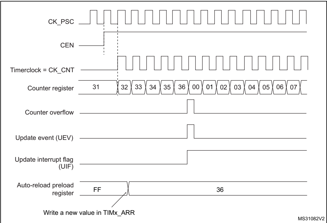
Figure 114. Counter timing diagram, Update event when ARPE=0 (TIMx_ARR not preloaded)
