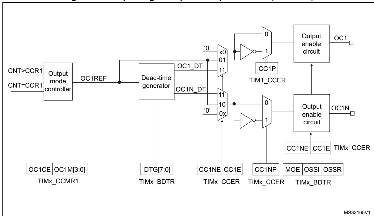
Figure 184. Output stage of capture/compare channel (channel 1)
