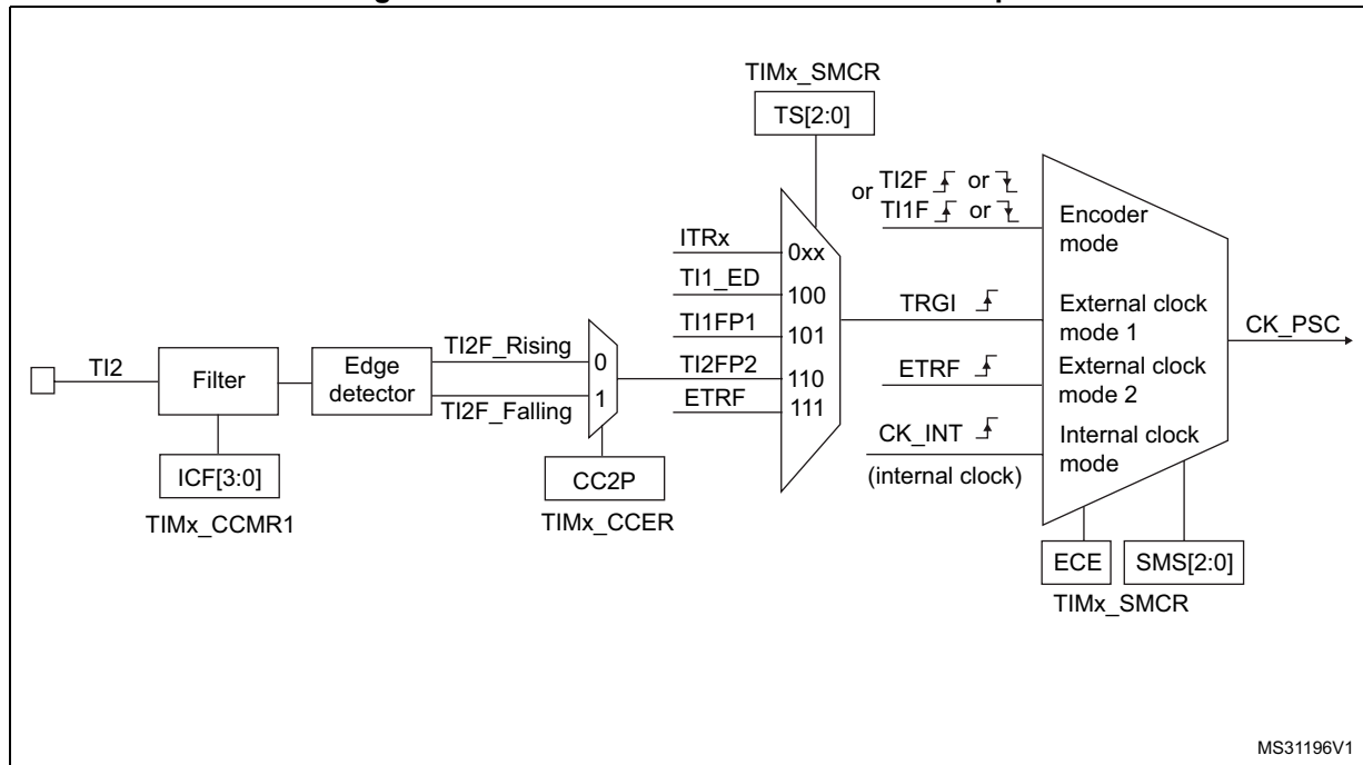
Figure 81. TI2 external clock connection example
