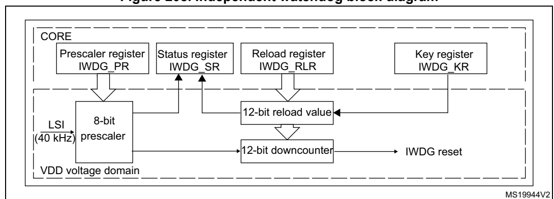
Figure 208. Independent watchdog block diagram
