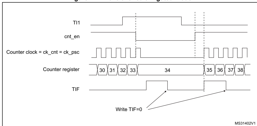
Figure 144. Control circuit in gated mode
