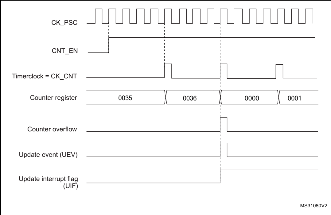
Figure 64. Counter timing diagram, internal clock divided by 4
