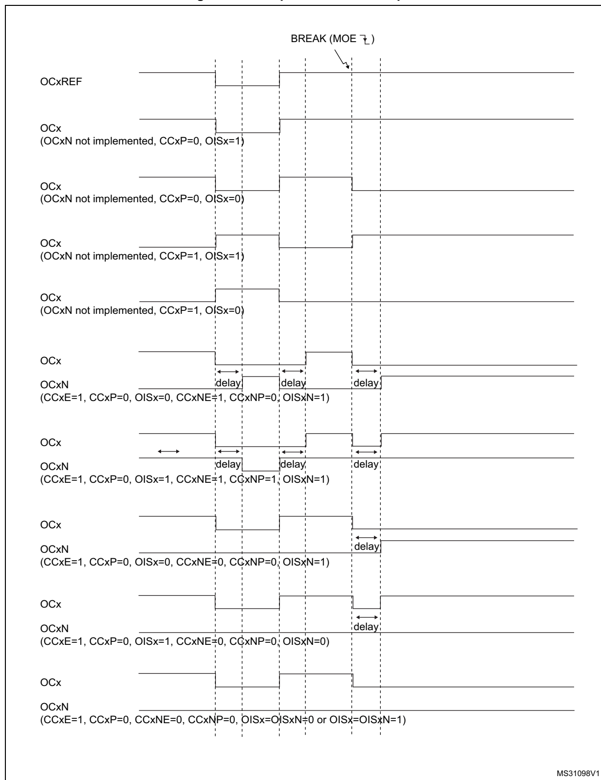
Figure 192. Output behavior in response to a break
