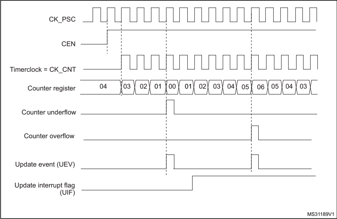
Figure 121. Counter timing diagram, internal clock divided by 1, TIMx_ARR=0x6
