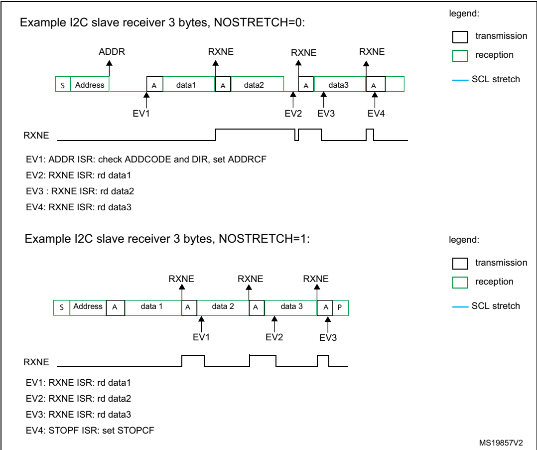
Figure 226. Transfer bus diagrams for I2C slave receiver
