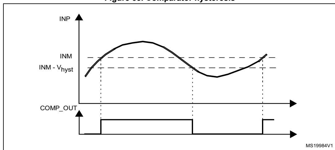
Figure 53. Comparator hysteresis
