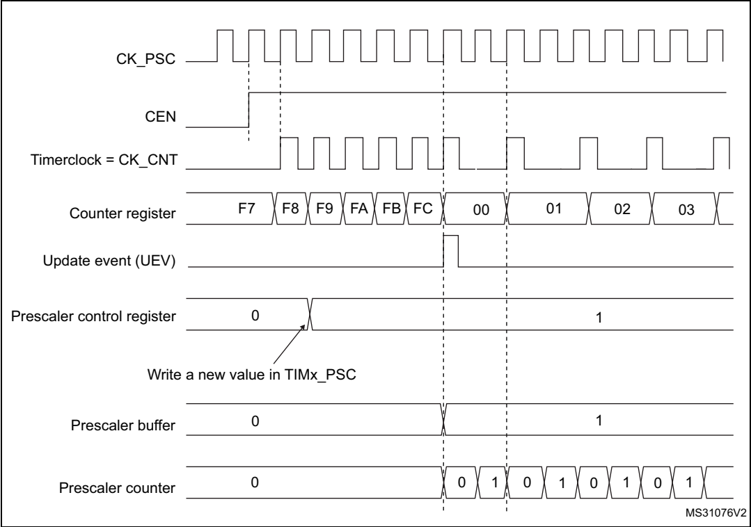
Figure 60. Counter timing diagram with prescaler division change from 1 to 2
