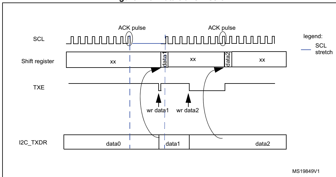
Figure 219. Data transmission
