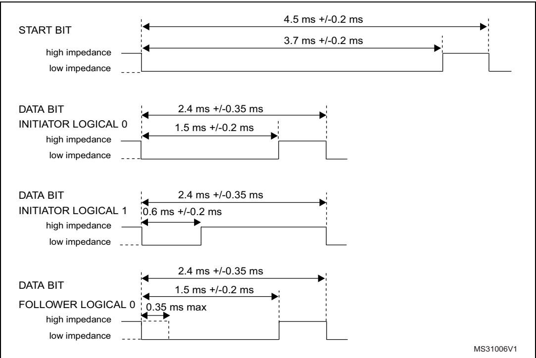
Figure 328. Bit timings
