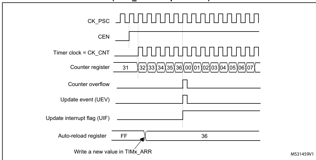
Figure 160. Counter timing diagram, update event when ARPE=0 (TIMx_ARR not preloaded)
