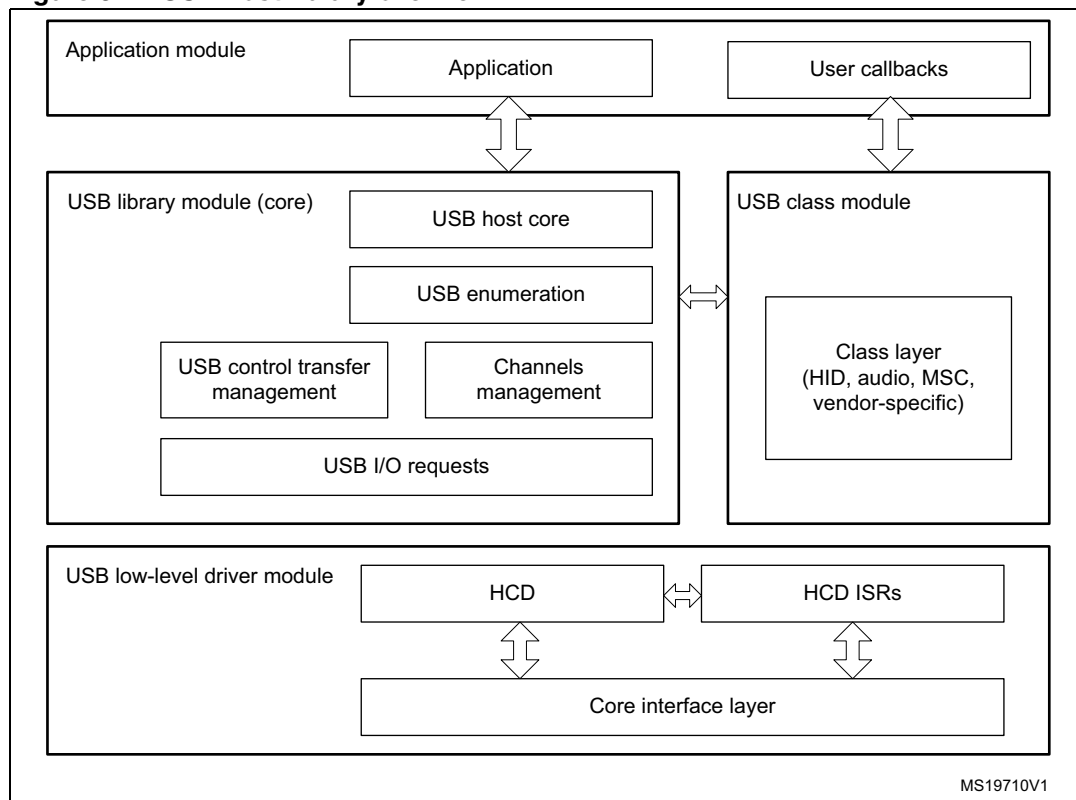
Figure 32. USB host library overview
