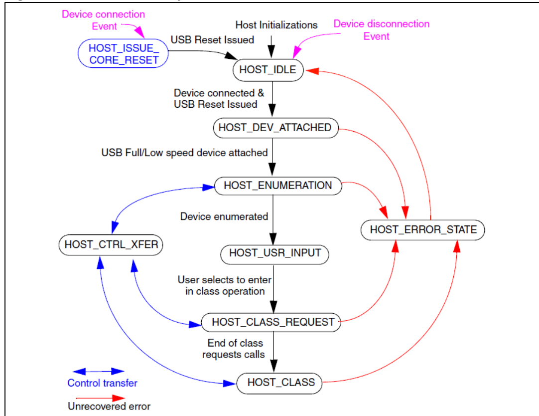
Figure 34. USB host library state machine
