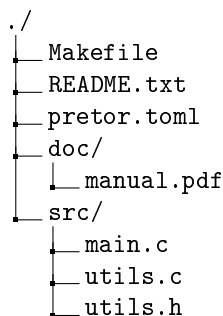
Figure 2: Sample project structure after adding pretor.toml .
