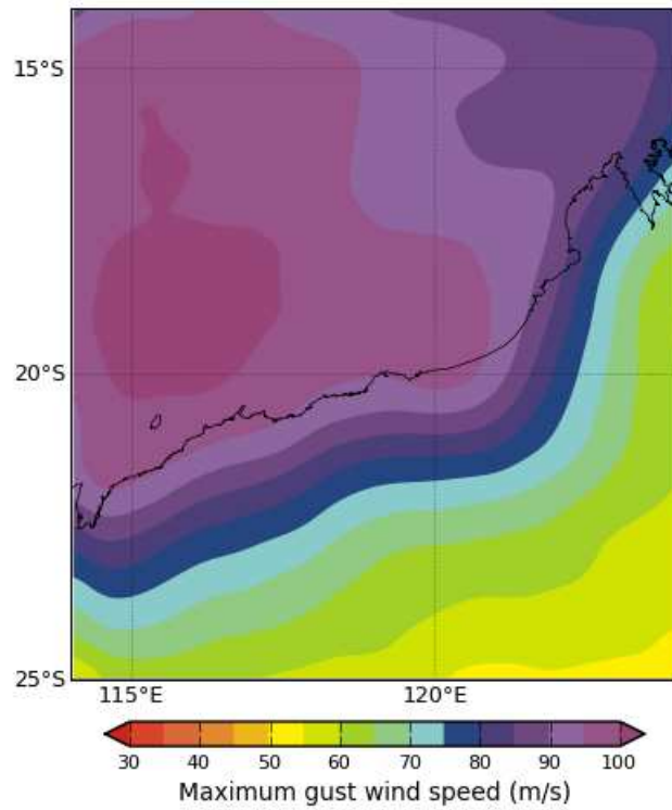
Figure 4: 500-year return period cyclonic wind hazard for north-west Australia
