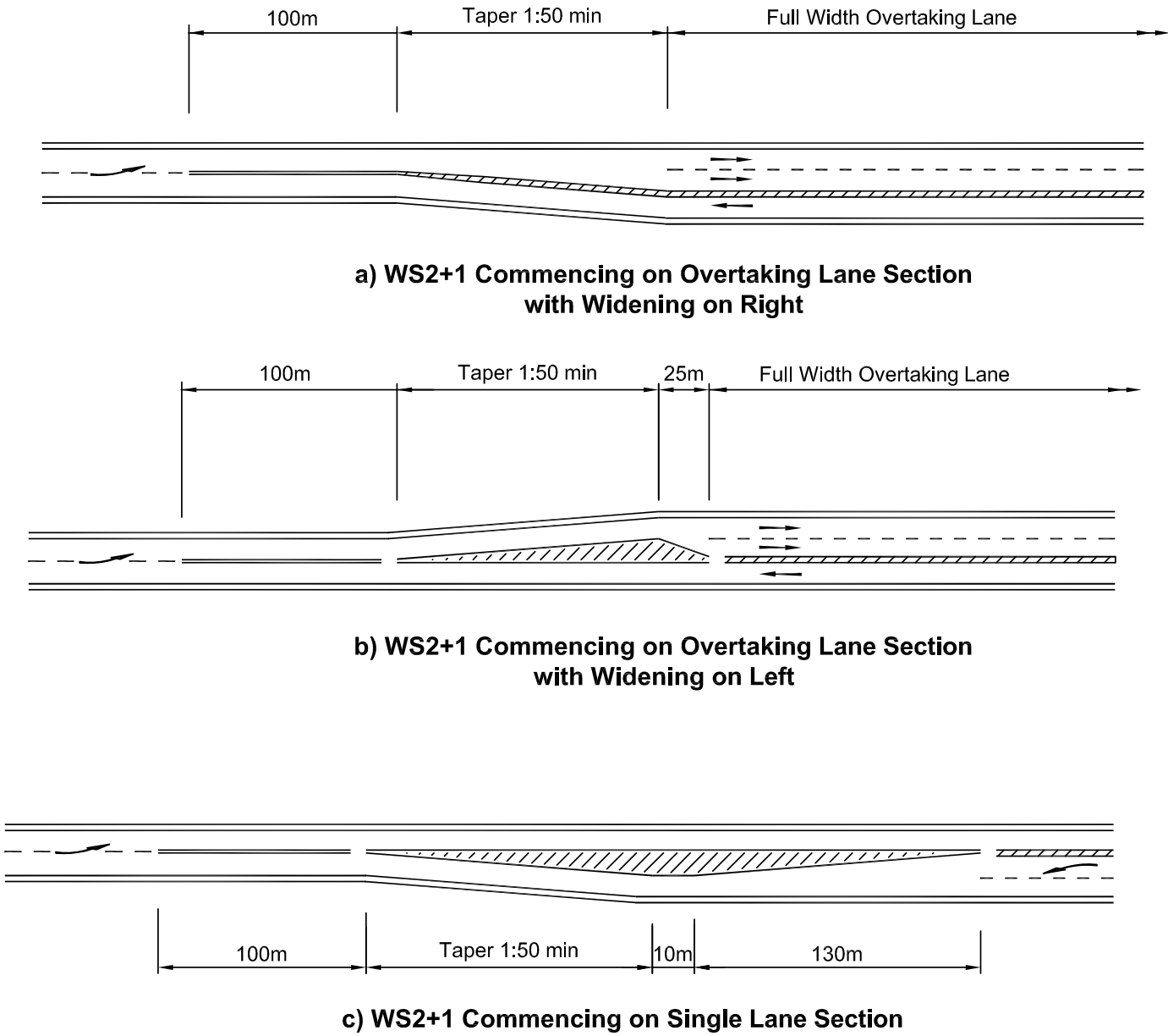
Figure 3/4: WS2+1 Interfaces
