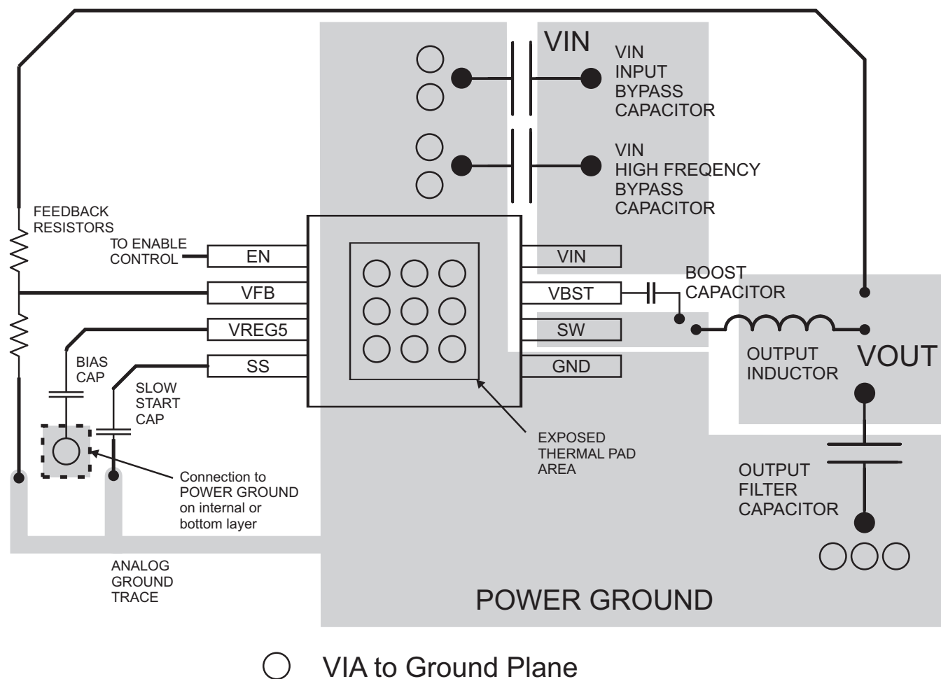
Figure 16. PCB Layout
