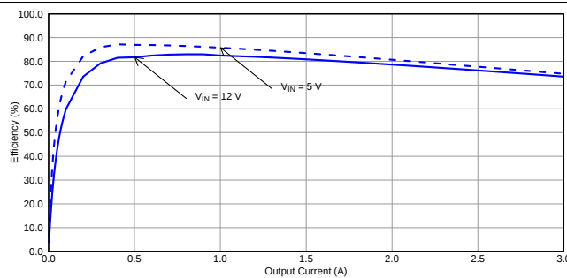
Figure 14. TPS54327EVM-686 Efficiency
