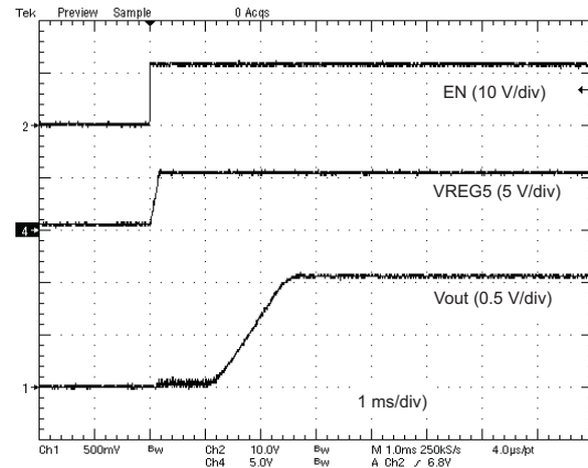
Figure 11. Start-Up Wave Form
