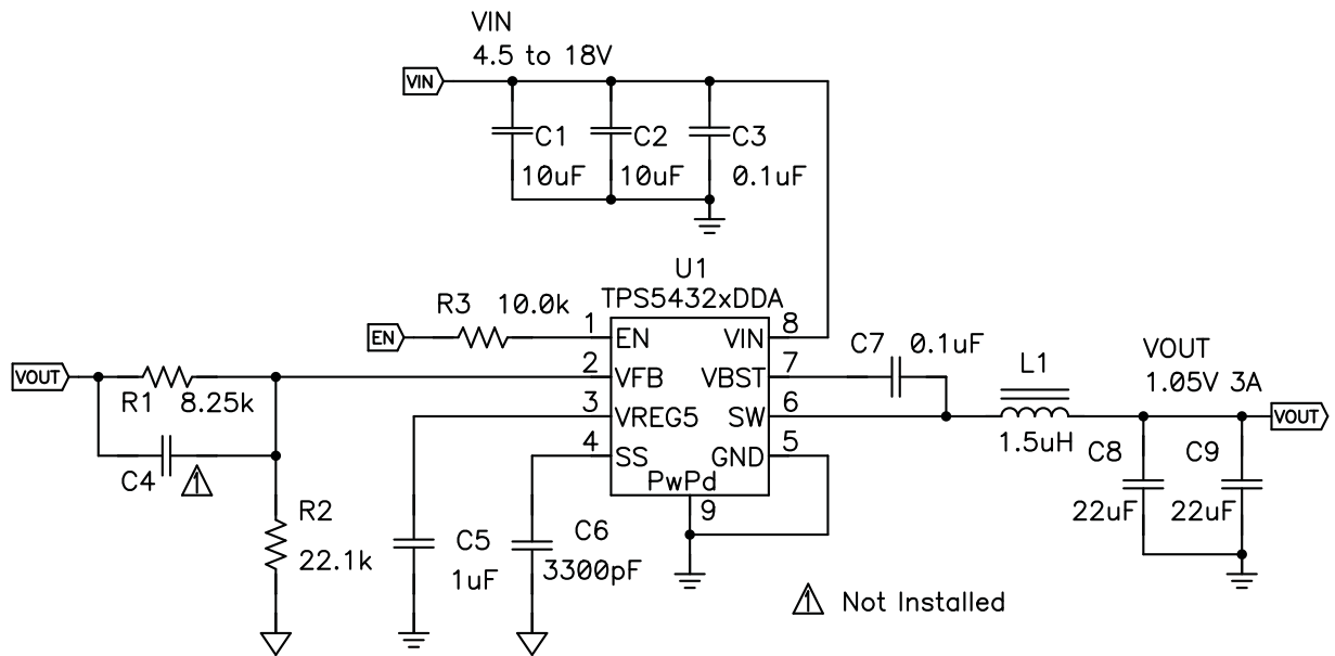
Figure 7. Schematic Diagram
