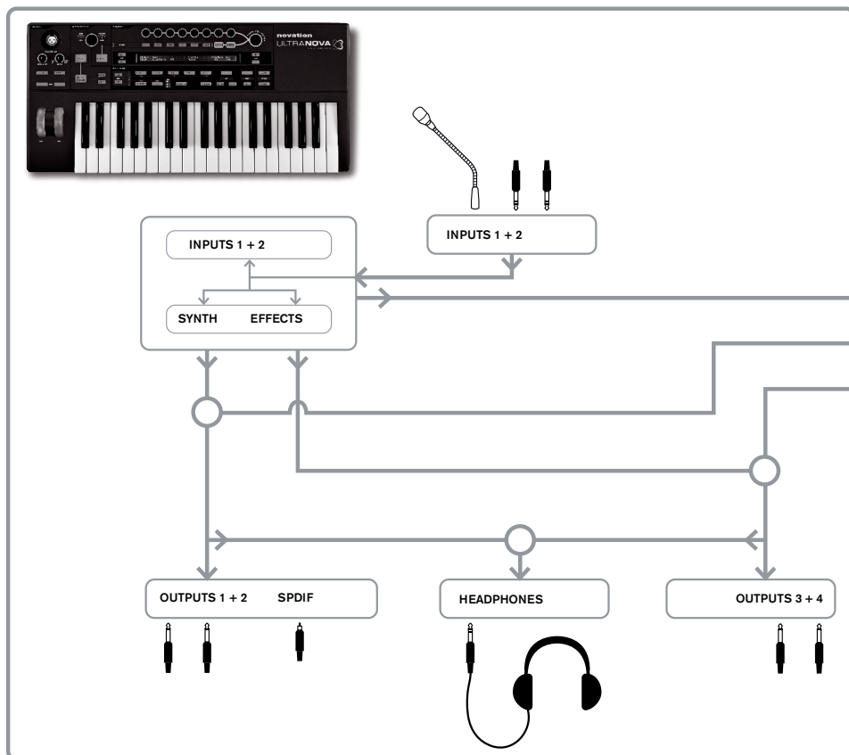
AUDIO ROUTING IN THE ULTRANOVA
