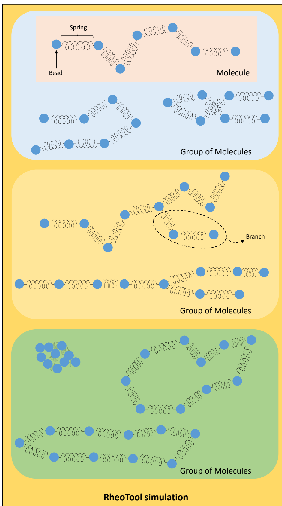
Figure 3.1: Polymer molecules representation by a bead-spring model. The organization levels used in rheoTool are also represented: beads and springs, molecules and groups of molecules.
