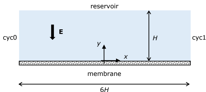
Figure 5.24: Planar reservoir with an ion-selective membrane (only permeable to cations) on its bottom.
