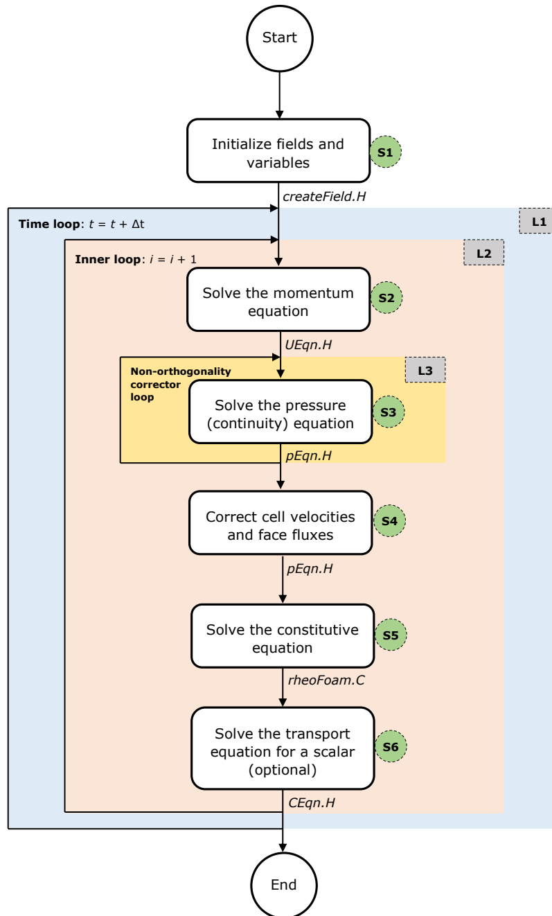
Figure 4.2: Solving sequence of rheoFoam under a segregated solution method (steps related with mesh motion are omitted for simplicity).
