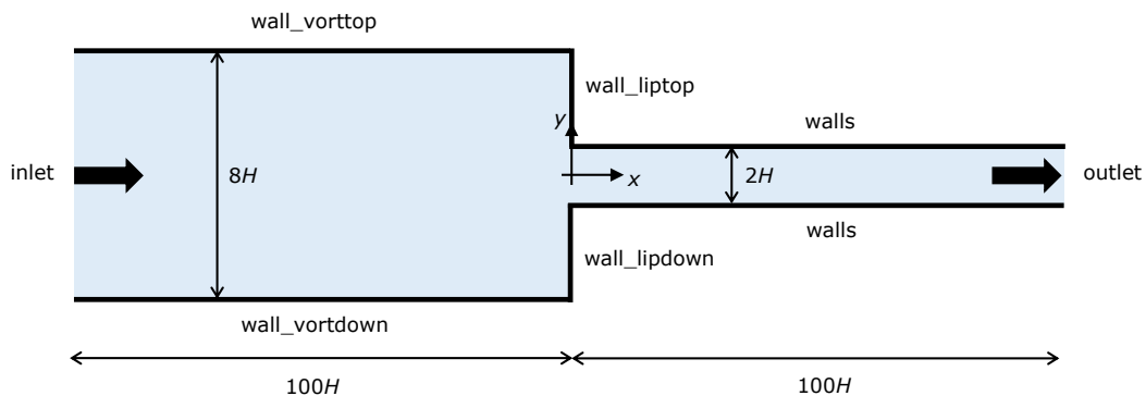
Figure 5.6: Geometry for the 4:1 planar contraction.
