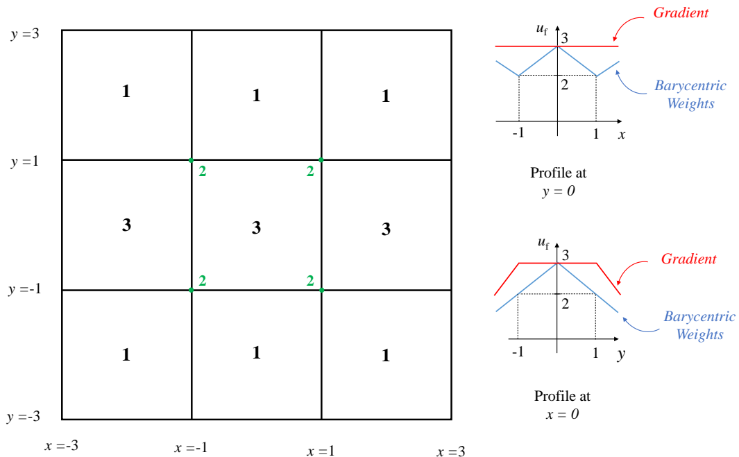
Figure 4.1: Hypothetical 2D external forcing field (a scalar field to simplify) in a co-located grid (values at cell centers), aiming to represent a fully-developed field in the x -direction. The green values defined at vertices are obtained by inverse distance weighting of the cell-centered data. On the right, the profiles of u_f taken at x = 0 and y = 0 are represented for two different interpolation methods.
