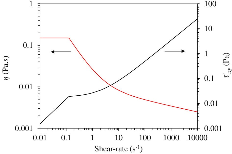
Figure 5.15: Shear viscosity and \tau'_{xy} (the only non-zero component of the symmetric extra-stress tensor) as a function of the shear-rate, in a steady shear flow, for the Herschel-Bulkley model with parameters: \tau_0 = 0.0175 Pa, k = 8.9721 \times 10^{-3} Pa.s n , n = 0.8601 and \eta_0 = 0.15 Pa.s.
