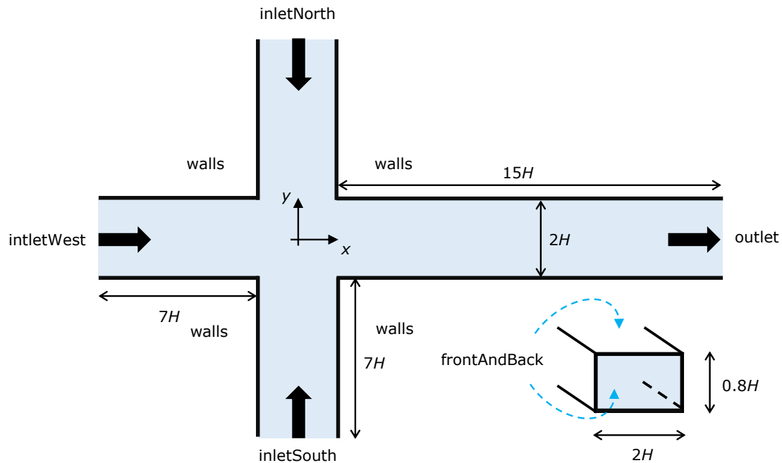
Figure 5.25: Three-dimensional flow-focusing device.
