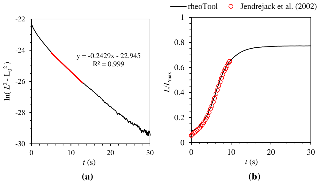
Figure 5.31: (a) Decay of the molecular length over time during relaxation in no-flow conditions. The red line represents a linear fit to the data for 5 \leq t \leq 13 s. (b) Fractional molecular length evolution over time in a planar extensional flow at Wi = 2 . The symbols represent the numerical results from [25].
