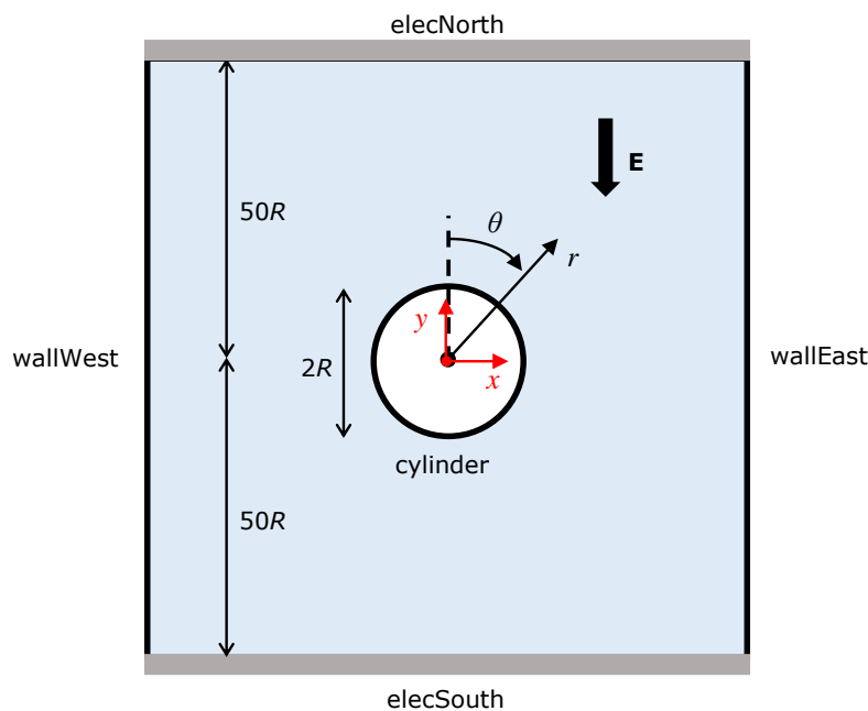
Figure 5.23: Metallic cylinder placed over an electric field. The surrounding domain is square (edge size: 100R ) and the cylinder lays on its center. The cylindrical coordinate system (r, \theta) is plotted in black, while the Cartesian coordinate system (x, y) is represented in red (remember that OpenFOAM ® uses the Cartesian system for computations).
