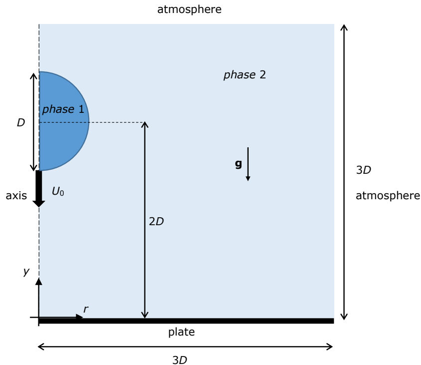
Figure 5.17: Geometry for the impacting drop problem.
