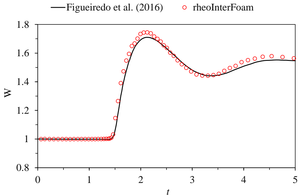
Figure 5.18: Evolution of the drop width over time for Fr = 2.26 , Re = 5 , Wi = 1 and \beta = 0.1 . The profile obtained with rheoInterFoam is compared with the data of Figueiredo et al. [49].
