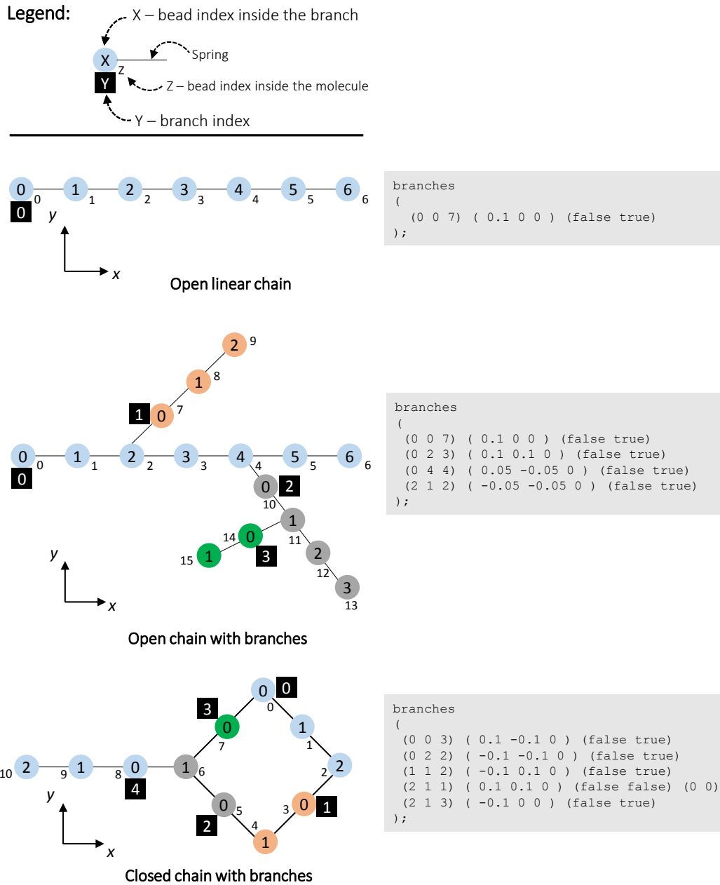
Figure 4.4: Example of 3 molecules and corresponding branches settings to generate them with utility initMolecules .
