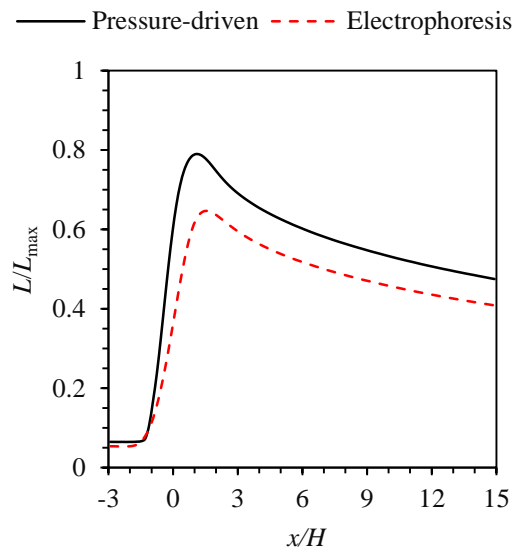
Figure 5.32: Fractional molecular length of 7\lambda -DNA in the flow-focusing geometry, under two types of external forcing. Results are for VR = Wi = 20 .
