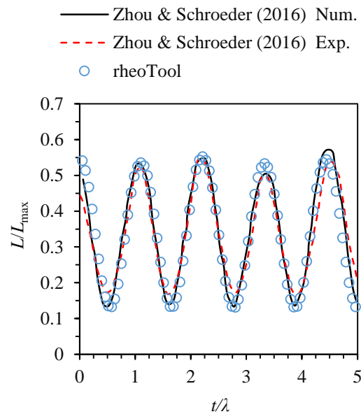
Figure 5.33: Fractional molecular length of \lambda -DNA in LAOE, for Wi = 6.5 and De = 0.45 . The lines are for the experimental (dashed) and numerical (solid) results in [59], while the symbols represent the numerical results obtained with rheoTool .
