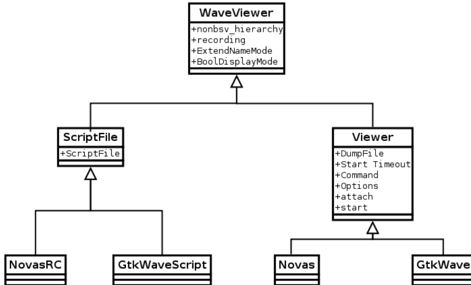
Figure 38: Inheritance of WaveViewer Class
