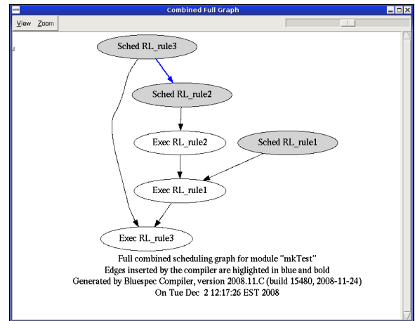
Figure 26: Combined Full Graph
