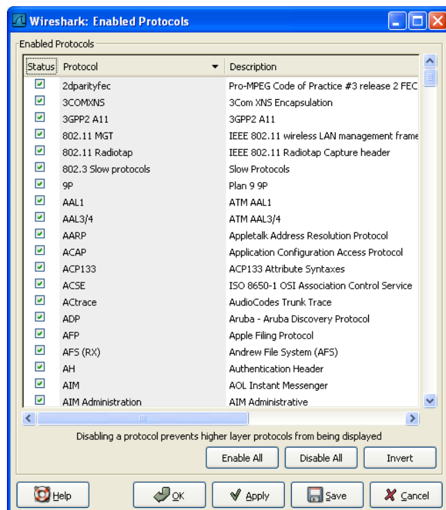
Figure 10.5. The "Enabled Protocols" dialog box
