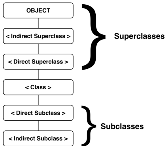
Fig. 8.2 Class Relationships
