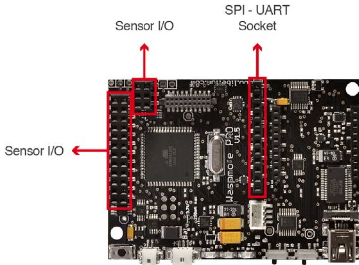
Figure: I/O connectors in Waspote
