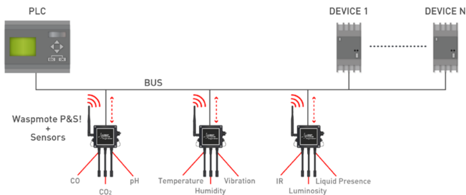
Figure: Module in wireless sensor network applications
