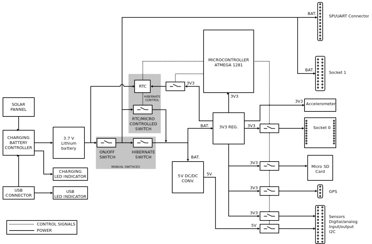
Figure: Waspote block diagrams – Power signals
