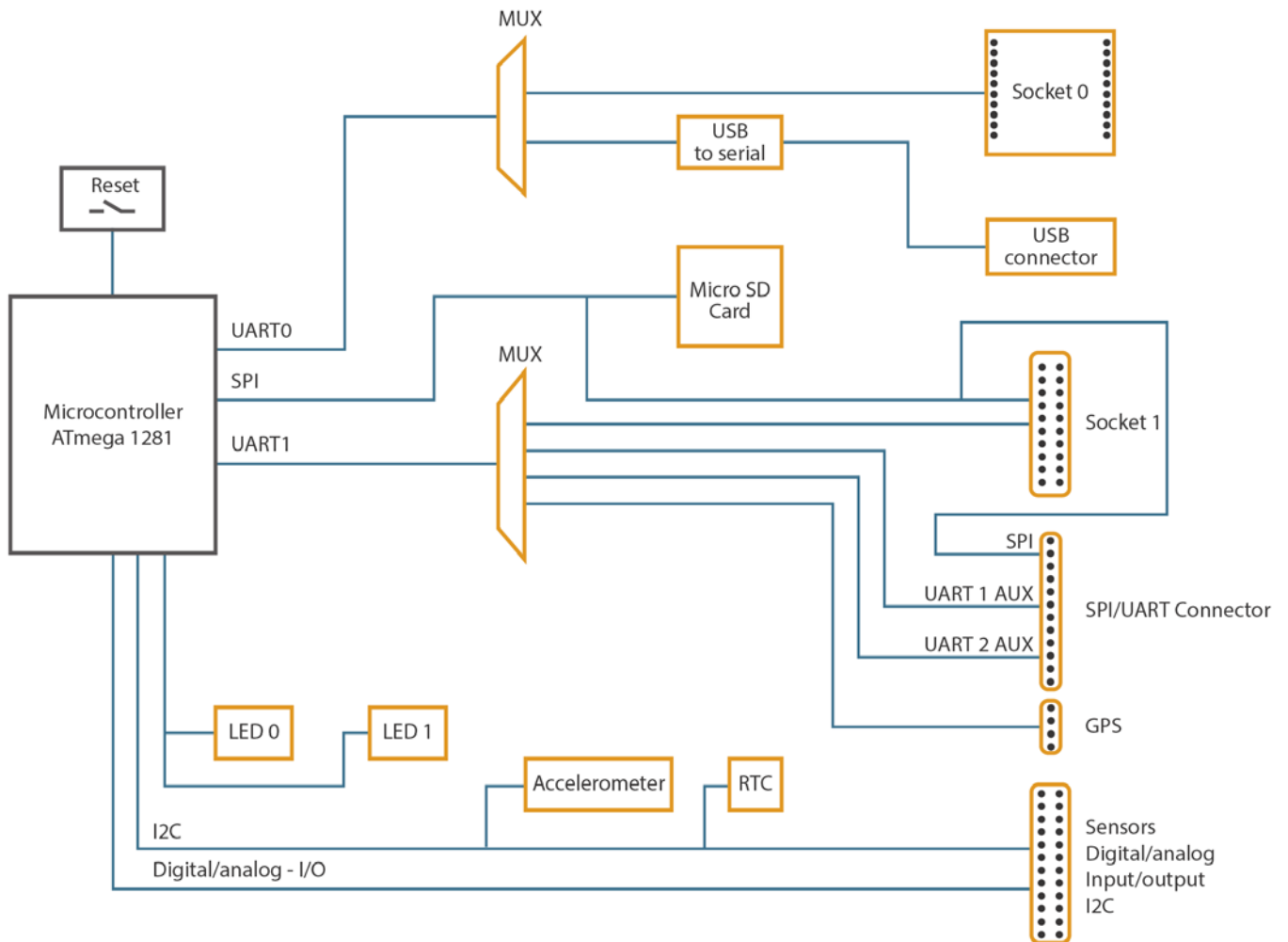
Figure: Waspmote block diagrams - Data signals
