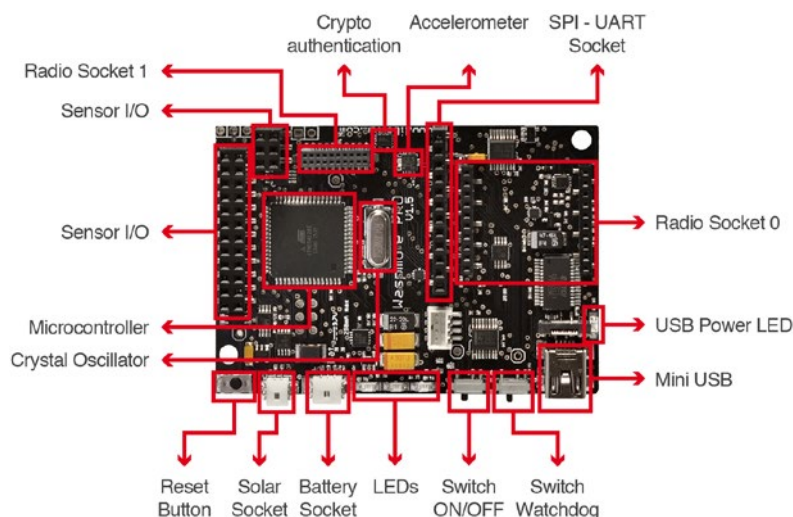
Figure: Main Wasp mote components – Top side
