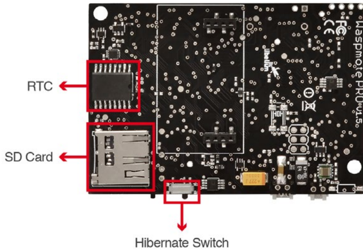
Main Waspmote components - Bottom side
