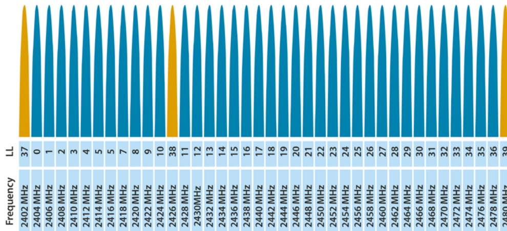
Figure: Channel distribution on the BLE standard
