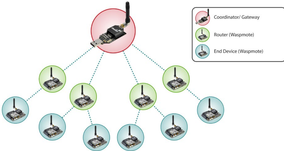
Figure: Tree topology
