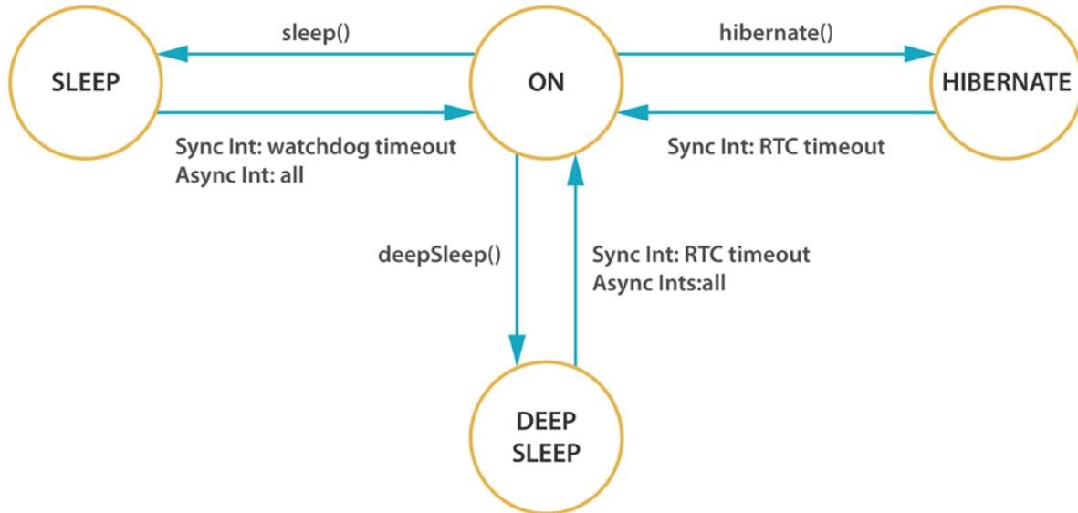
Figure: Diagram of mode in Waspote
