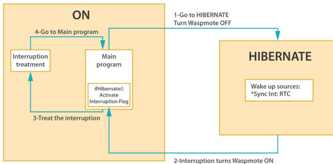
Figure: From on to Hibernate mode
