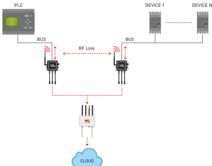
Figure: Wasp mote for wire replacement
