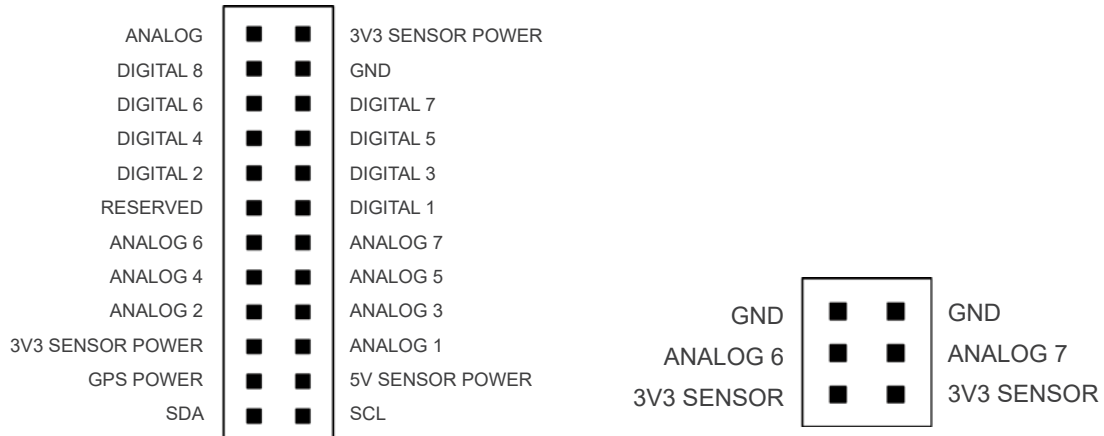
Figure: Description of sensor connector pins
