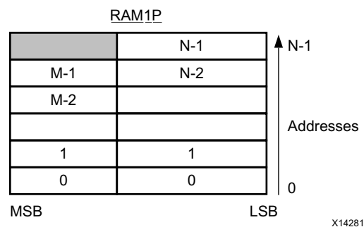
Figure 1-69: Memory for Vertical Mapping
