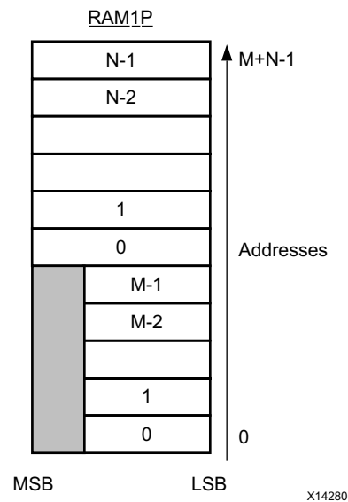
Figure 1-66: Memory for Horizontal Mapping
