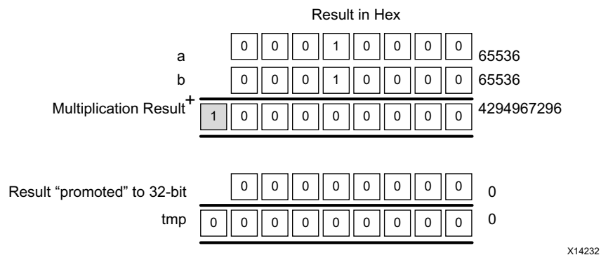
Figure 2-2: Integer Promotion
