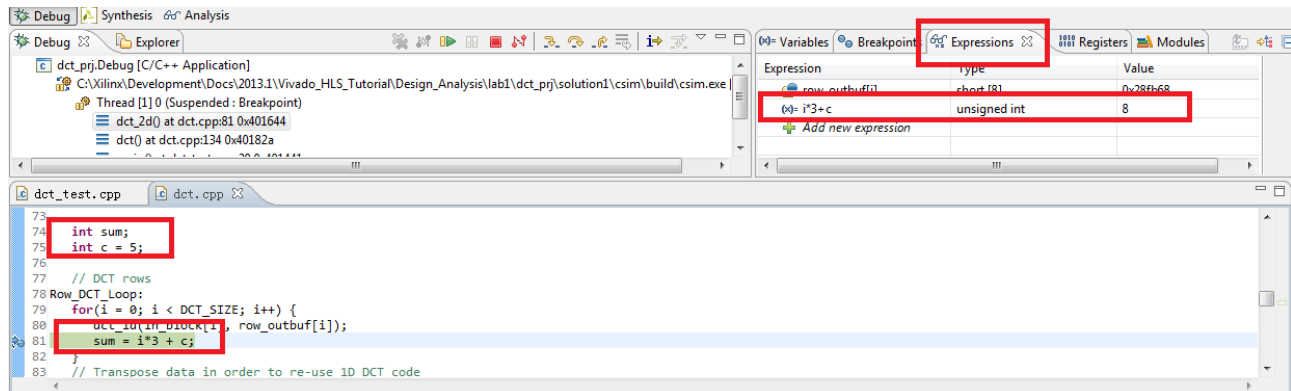
Figure 4-2: Monitoring Expressions
