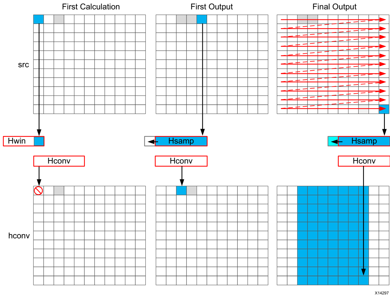
Figure 3-6: Streaming Horizontal Convolution
