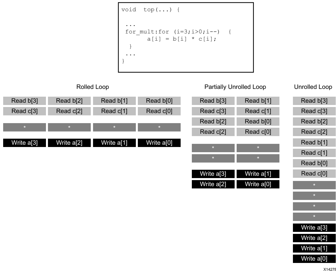
Figure 1-60: Loop Unrolling Details
