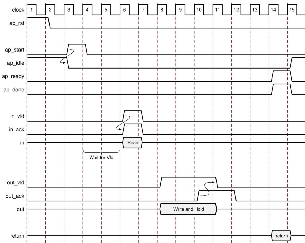
Figure 4-8: Behavior of ap_hs Interface
