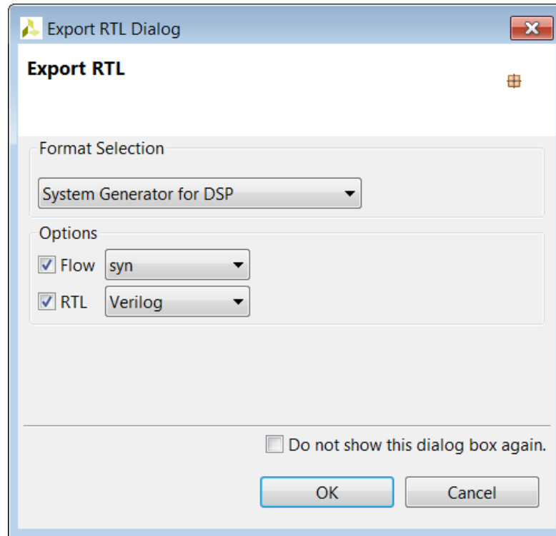
Figure 1-76: Export RTL to System Generator
