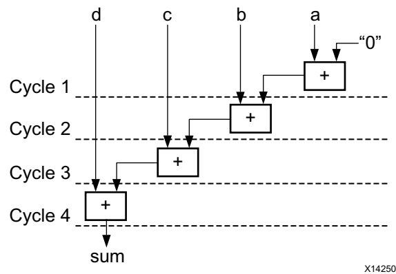
Figure 1-71: Adder Tree
