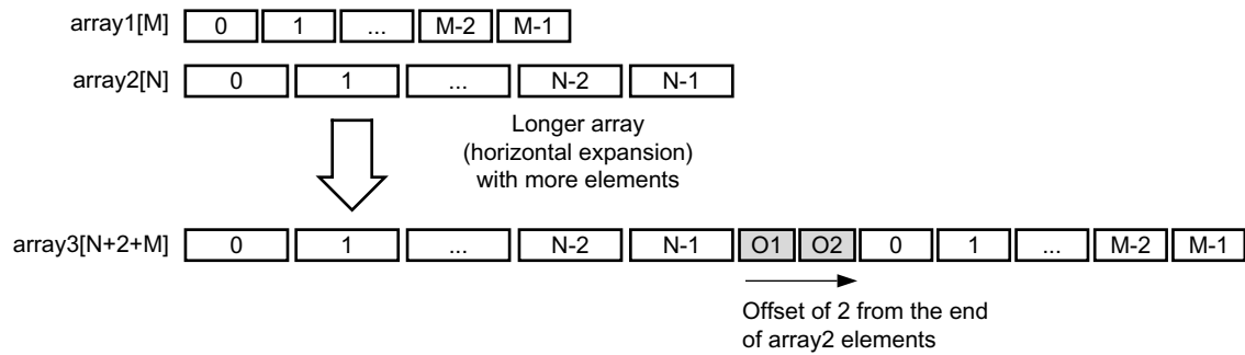
Figure 1-67: Horizontal Mapping with Offset
