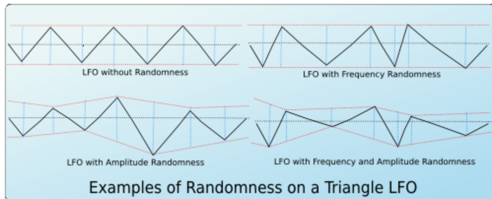
Figure 61: LFO Randomization
