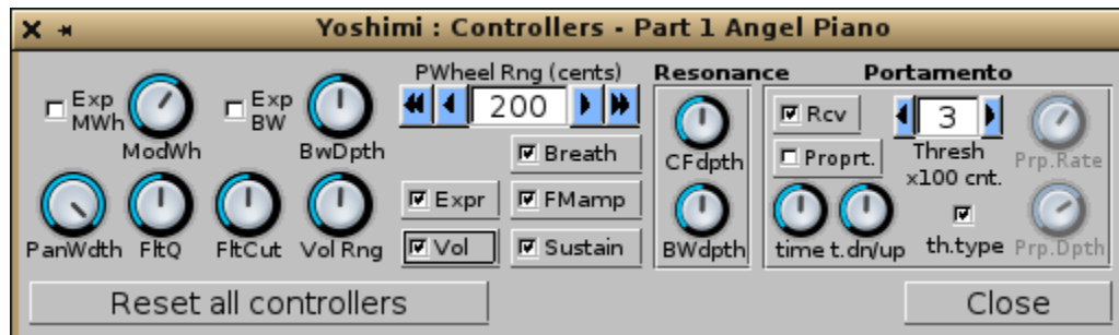
Figure 107: Controllers Dialog
