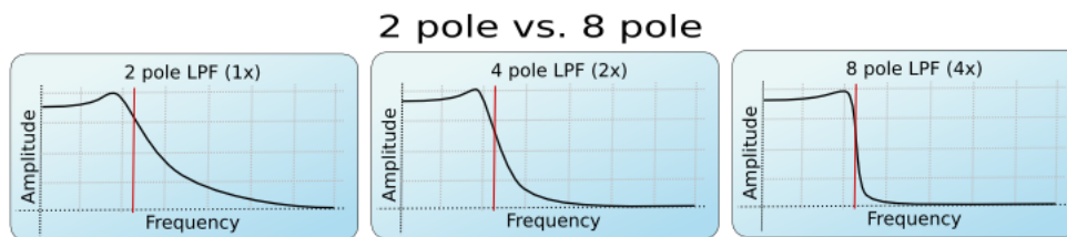
Figure 51: The Effect of the Order of a Filter
