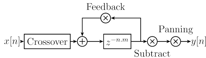
Figure 95: Chorus Circuit Diagram
