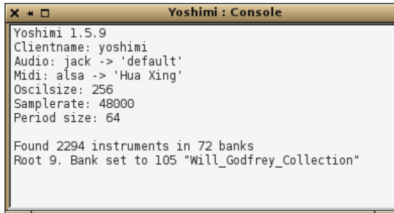
Figure 15: Console Window
