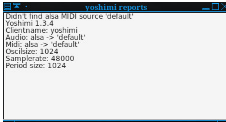
Figure 85: Effects / Reports
