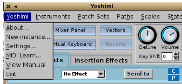
Figure 5: Yoshimi Menu
