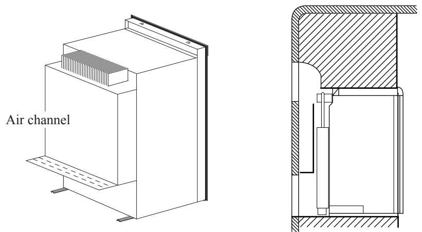
SIDE VIEW WITH DUCT SYSTEM DM2852, DM2862, DM3862 & NDM1062
