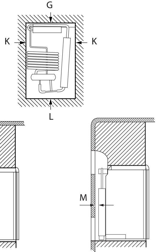
SIDE VIEW WITH DUCT SYSTEM DM2852, DM2862, DM3862 & NDM1062
