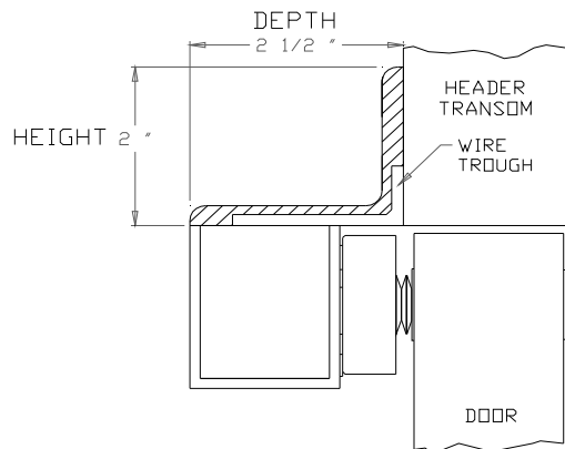
1194 ANGLE BRACKET
