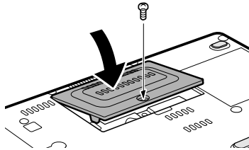
Figure 8-7 Seating the memory module cover
