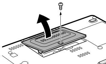
Figure 8-5 Removing the memory module cover
